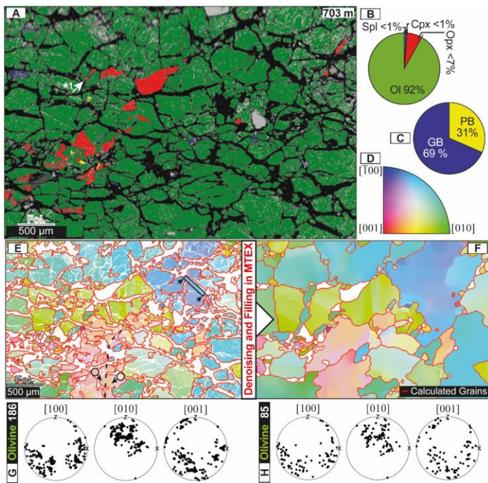
Fig. 5. A: Example microstructure of olivine-rich matrix in sample from 703 m distance to the NW-B. Area percentages (B), phase and grain boundary percentages (C) are given in pie charts. The olivine orientation colour key for maps E & F is given in D. EBSD data reconstruction and denoising, optimized for olivine, is shown in E-H. E: Original ol orientations data with calculated grain boundaries (red). Examples of intracrystalline deformation by bending of the crystal lattice (box) and subgrain boundary (dashed line) covering and crossing multiple calculated fragmental grains are annotated. F: Denoised and filled ol orientation map with calculated grain boundaries (red). Olivine orientation plots of original (G) and reconstructed data (H).
