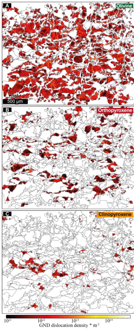
[345 Fig. 7. Geometrically necessary dislocation (GND) density maps for olivine (A), orthopyroxene (B) and clinopyroxene (C) off from the mylonitic mixed matrix shown in figure 6A-i. Note grain internal deformation in all phases and the formation of subgrain boundaries visible by bright yellow lines.
