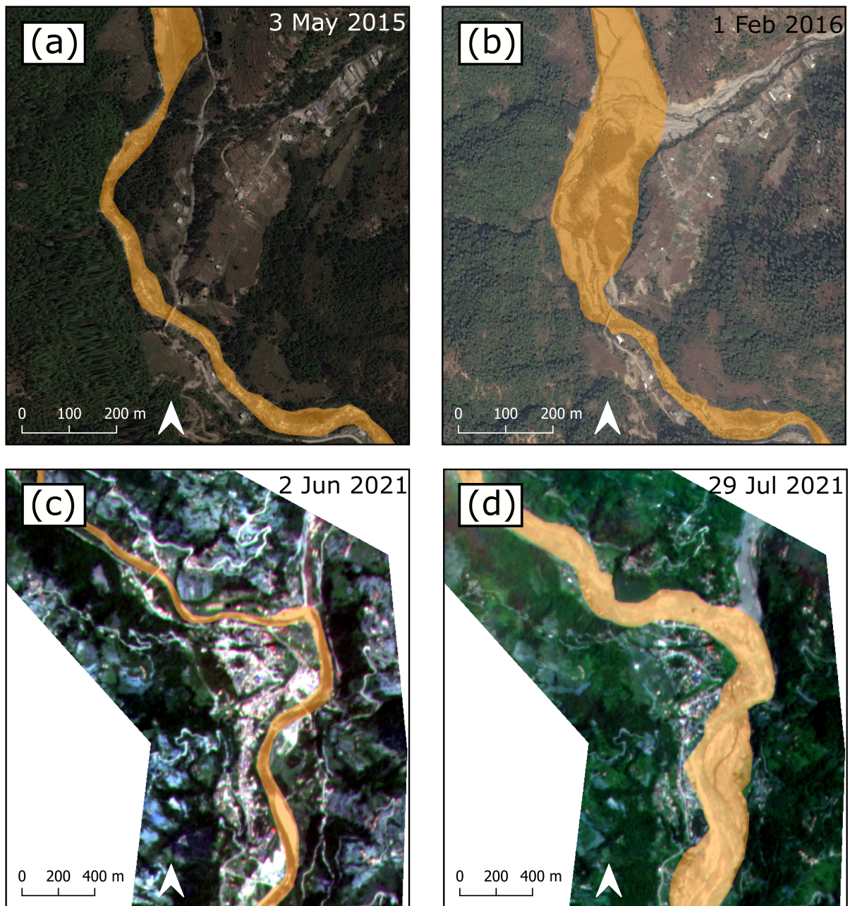
Figure 3. Examples of mapped sections, with the mapped sediment area polygons shown in yellow. Top panels show a section around Timbu overlain on imagery obtained through Google Earth Pro (©2022 Maxar Technologies). Bottom panels show a section around Melamchi Bazaar overlain on Planetscope imagery (Planet Team, 2017). See Fig. 1b for location of the sections within Melamchi-Indrawati catchment. (a) Sediment area on 3 May 2015; (b) Sediment area on 1 February 2016. Note the influx of sediment from the tributary to the NE; (c) Sediment area on 2 June 2021; (d) Sediment area on 29 July 2021. Note the dramatic increase in sediment area extent following the 15 June 2021 Melamchi disaster.
