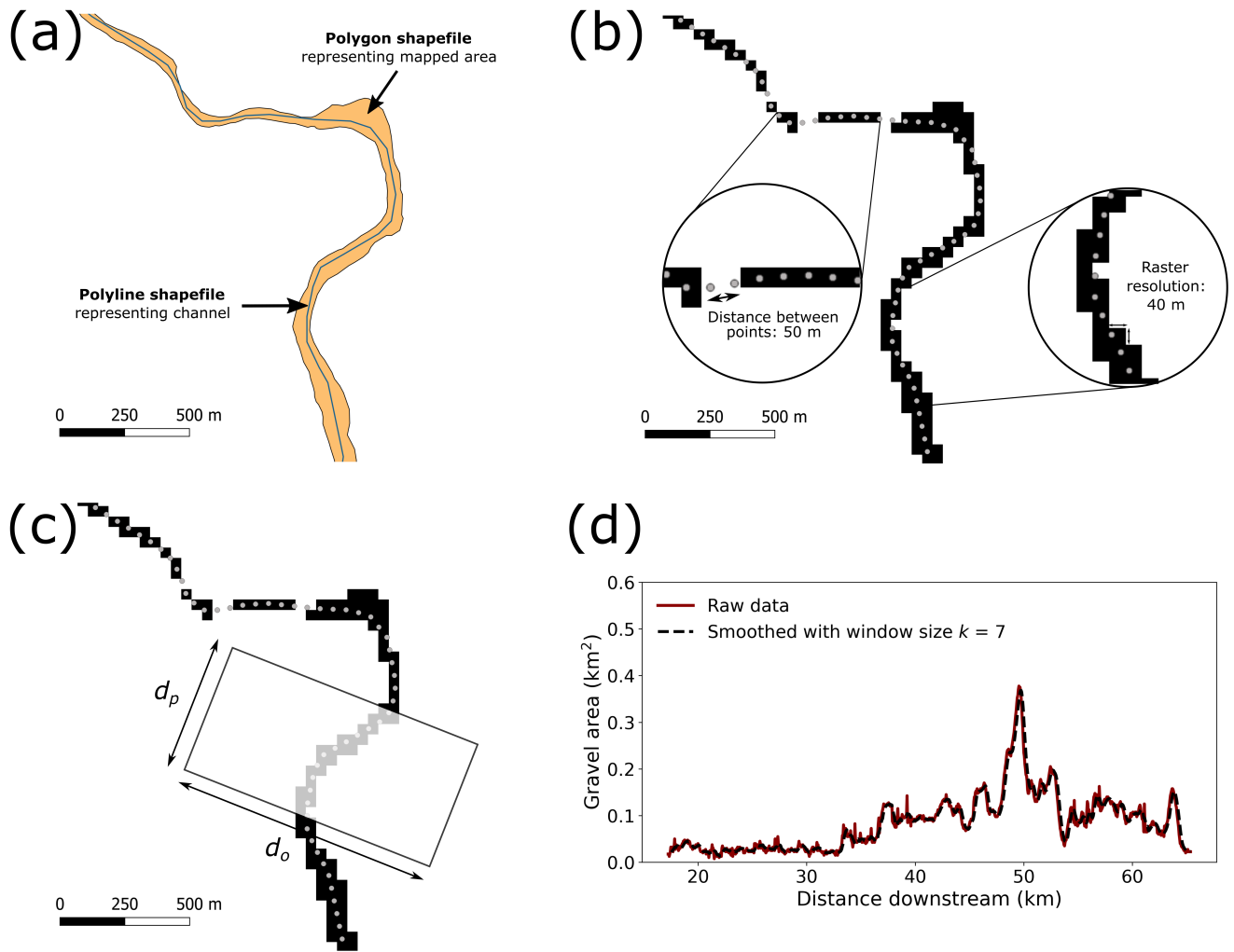
Figure 4. Steps for processing the data shown using an example section near Melamchi Bazaar (see Figs. 1b and 3c, d for location). (a) Original mapped channel and sediment areas. (b) The polygon representing the sediment area is converted to a raster and the line representing the channel is split into points. Note that the rasterisation process creates apparent gaps where sediment areas are narrower than the resolution of the raster res_r ; this does not affect the trends in area along the channel (Figs. A1a and A2a in the Supplementary Information). (c) A window of width d_o and length d_p is created around each channel point and the raster area within each window is calculated. (d) The raster area calculated within each window along the river is smoothed using a rolling window and plotted as a function of distance along the channel.
