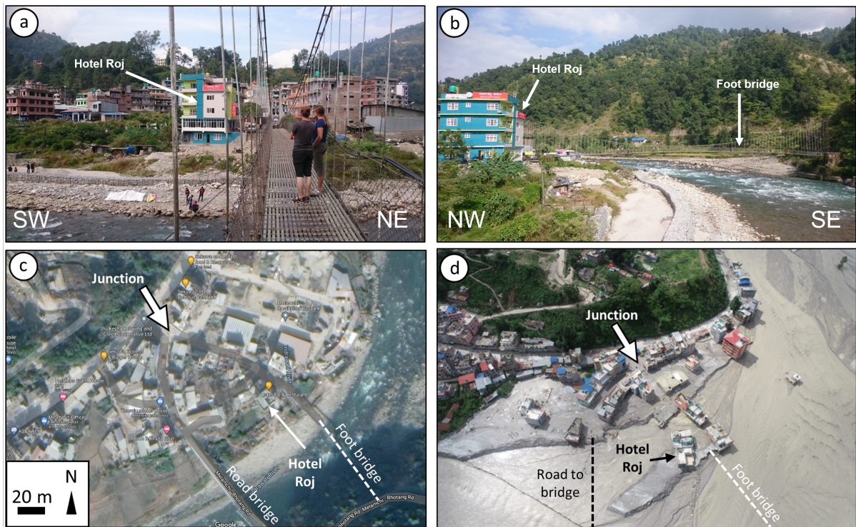
Figure 2. Impact of the 2021 Melamchi flood in Melamchi Bazaar (MB in Fig. 1b). (a) Picture from footbridge towards Melamchi Bazaar, looking NW, taken on 28/10/2019. Colourful building in the centre of the photo is Hotel Roj, used as a reference in the other photos (position: 27.82917^{\circ}\text{N} , 85.57714^{\circ}\text{E} ). Note gabions along the gravel bar to limit bank erosion during monsoon floods. (b) Picture from road bridge looking NE, upstream the Indrawati River, taken on 28/10/2019. Hotel Roj is to the left. Note gabions on the gravel bar. (c) Google Map of Melamchi Bazaar before the 2021 Melamchi flood (©2021 Maxar Technologies). Road and foot bridges are located, as well as road junction and Hotel Roj, for reference. (d) Aerial image of Melamchi Bazaar after the main flood event of June 2021, looking NW (source: Geovation Nepal). Both bridges have been destroyed, and only the top two floors of Hotel Roj emerge from the sediment, indicating aggradation in excess of 10 m.
