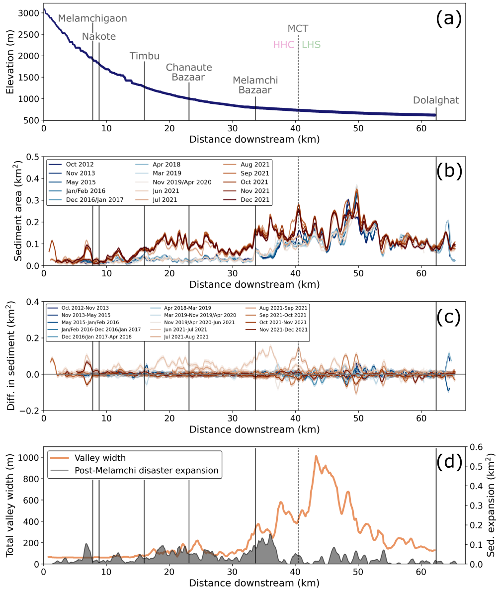
Figure 6. Changes in sediment area along the Melamchi-Indrawati rivers: (a) Long-profile of Melamchi-Indrawati river within the study area; (b) Mapped sediment area per 0.5 \text{ km}^2 window along profile; (c) Difference in mapped area along profile between each time period; (d) Valley width extracted with LSDTopoTools plotted alongside mapped expansion in sediment between June and July 2021 (i. e. difference in mapped sediment area before and after the Melamchi event). Areas until November 2019/April 2020 inclusive mapped in Google Earth Pro; areas from June 2021 onward mapped in QGIS from Planetscope imagery. Locations mentioned in the text are labelled in (a) and shown with vertical grey lines. Dashed grey line indicates approximate location of Main Central Thrust (MCT), separating the Higher Himalayan Crystallines (HHC) from the Lesser Himalayan Sequence (LHS).
