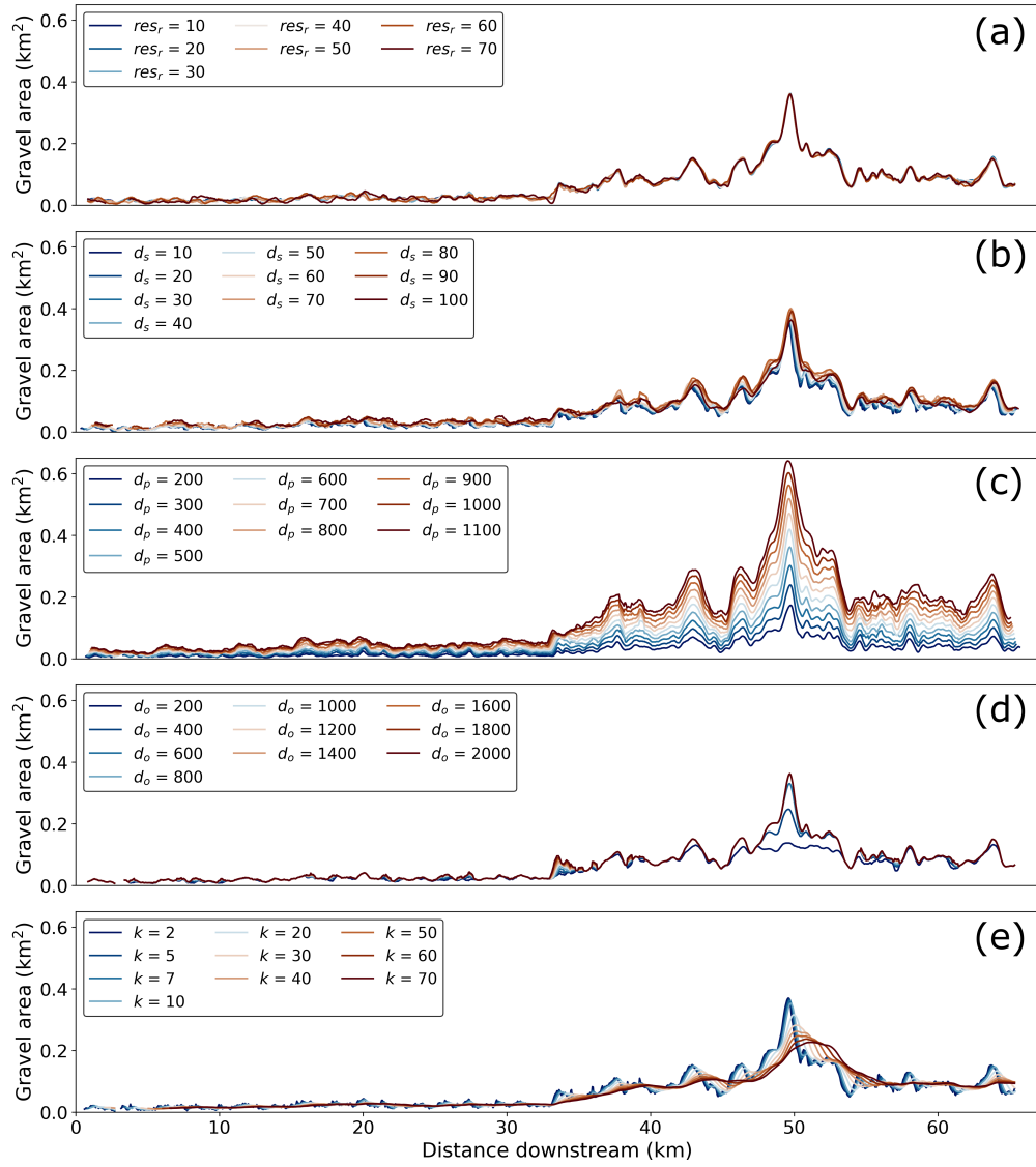
Figure A2. Area along profile for one mapping epoch, showing variation between parameter values. Areas are mapped along the Melamchi-Indrawati rivers from Planetscope imagery of 30/10/2020.
