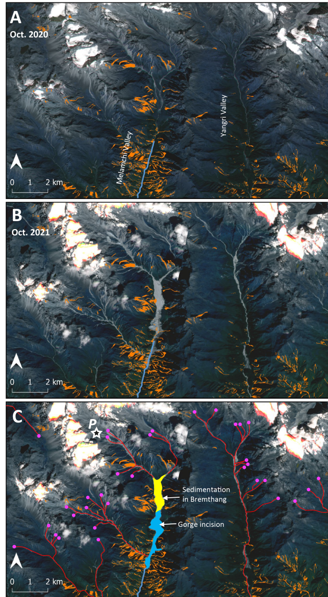
Figure 9. Planet Explorer 3.7 m optical satellite imagery (Planet Team, 2017) of the upper reaches of the Melamchi and Yangri valleys from October 2020 (A) and October 2021 (B). The images are overlain by the coseismic landslide data (orange) by Roback et al. (2018)). The lighter grey portions along the channels in B represent the remobilisation of sediment during the Melamchi disaster (see text). Panel C is an interpretation of B highlighting the channels where sediment has been remobilised during the event (in red), where extensive accumulation of sediment occurred in the Bremthang valley (yellow), and where gorge incision has taken place downstream of the Bremthang valley (blue shading). The pink dots approximate the position of the headwaters that record the first evidence of sediment remobilisation. We hypothesise that an extreme storm event initiated the disaster: the pink dots delineate the extent of the area affected by this hypothetical storm. Star labelled P shows location of Pemdang Lake where a glacial outburst flood has originated.
