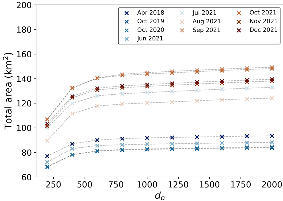
Figure A3. Total sediment
