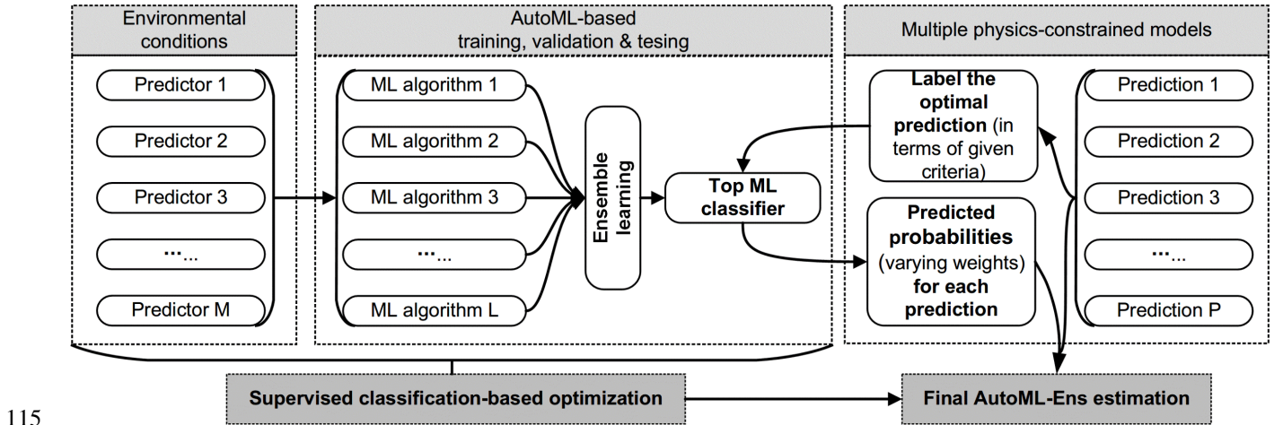
Figure 1. Procedures for building an AutoML-based ensemble framework (AutoML-Ens) to assemble geoscientific models.
