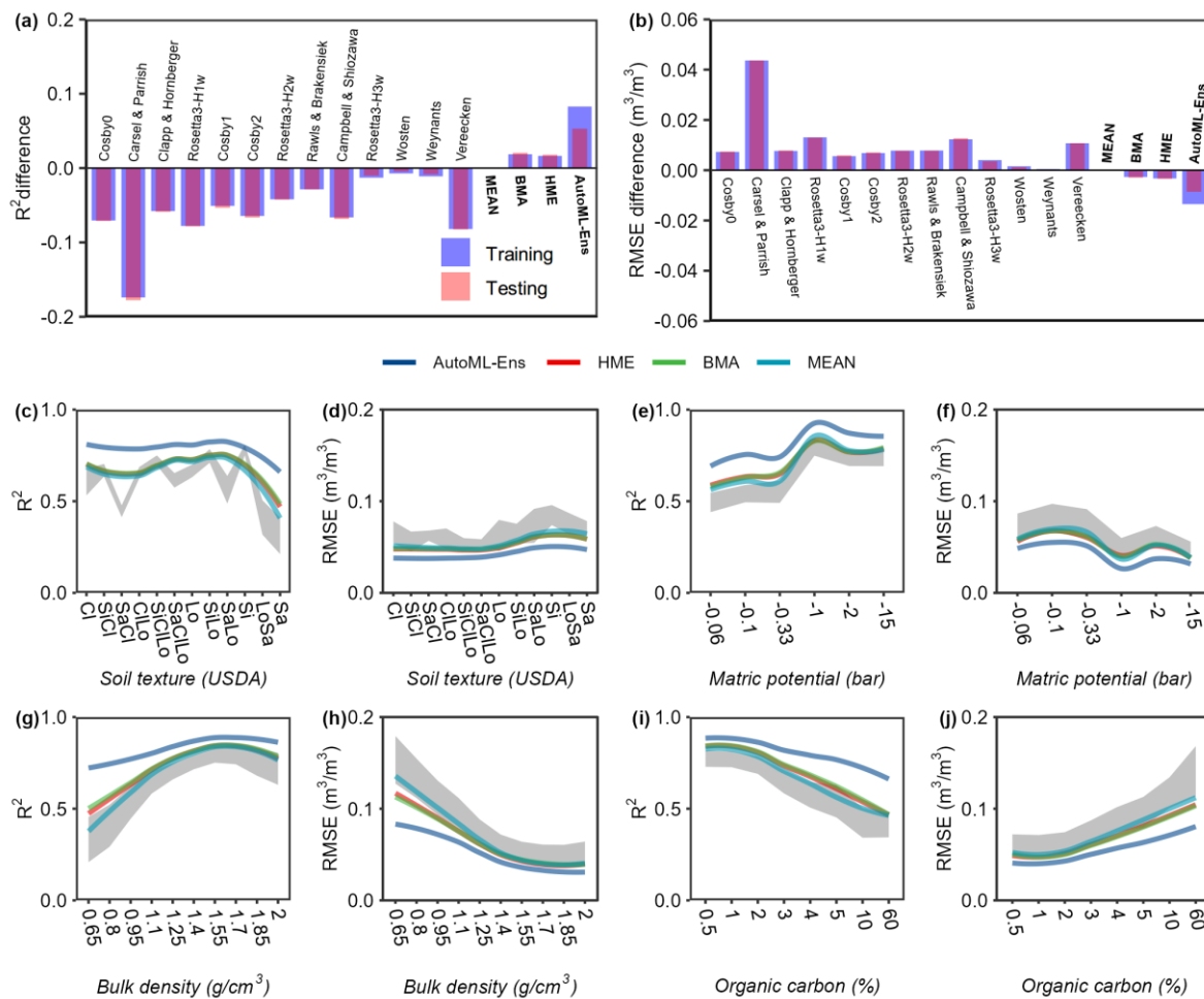
245 Figure 3. Difference in performance metrics ( R^2 (a) and RMSE (b)) between MEAN and all 17 models, including individual PTFs and model ensembles (in bold font) for training and testing data. A positive R^2 or negative RMSE difference means that the model yields a larger R^2 or smaller RMSE, indicating the better performance of the model than MEAN (considered as the benchmark). R^2 (c, e, g, i) and RMSE (d, f, h, j) when the moisture content estimates of different ensemble approaches were compared with observations (including all training and testing data) under various environmental conditions (6 variables, among which, the content of sand, silt, and clay was expressed together in terms of USDA soil texture classes) that were represented by predictors for AutoML-Ens. The gray band denotes the uncertainties calculated as the mean \pm standard deviation of the R^2 (or RMSE) values of the 13 selected PTFs. 250
