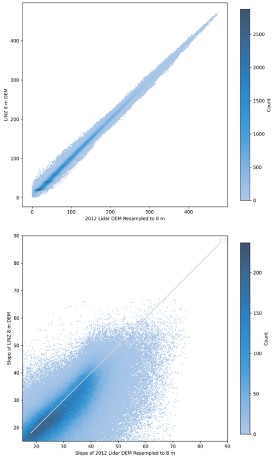
Figure A3. Relationship between LINZ 8 m DEM (LINZ, 2021a) and a 2012 Lidar DEM (LINZ, 2021c) in the top plot. The bottom plot shows the relationship between topographic slope derived from the same two datasets.
