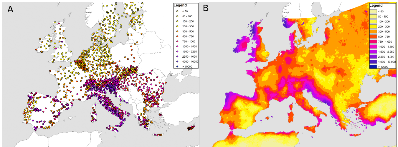
635 Figure 5: Comparison of gauge-derived erosivity estimates. Sub-figure A: R-values from the gauge-based REDES database (Panagos et al. 2015). Sub-figure B: R-values from the 30-minute IMERG derived estimates. The colour scheme for both datasets is the same, allowing for comparison of spatial results.
