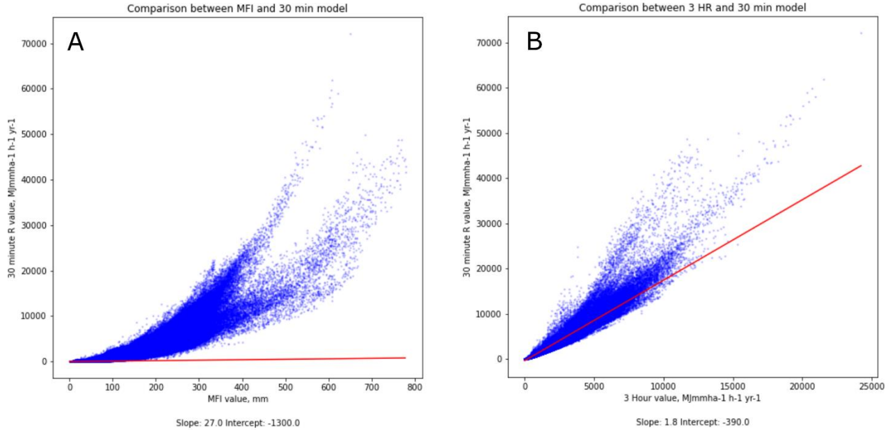
Figure 2: Comparison between cell-by-cell values of the 30-minute IMERG estimate of erosivity (y-axis) and the two other methods; (A) shows comparison between 30-minute IMERG estimate and MFI, while (B) shows the comparison between 30-minute IMERG estimate and the 3-hour IMERG data estimate. Note that the red lines in both figures show the 1:1 line, with values above that line indicating higher erosivity estimates in the 30-minute version. The 1:1 line in figure (A) does not have any physical meaning since MFI has different units, but is shown for illustrative purposes.
