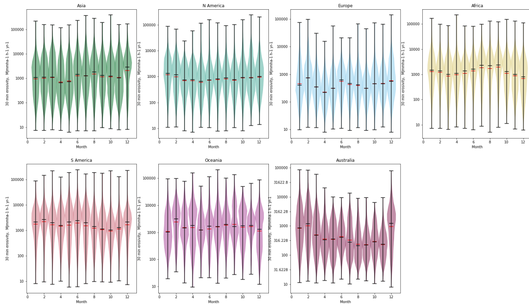
Figure 6: Monthly variability in erosivity calculated using IMERG 30-minute data, for each continent for the year 2020-2021.
