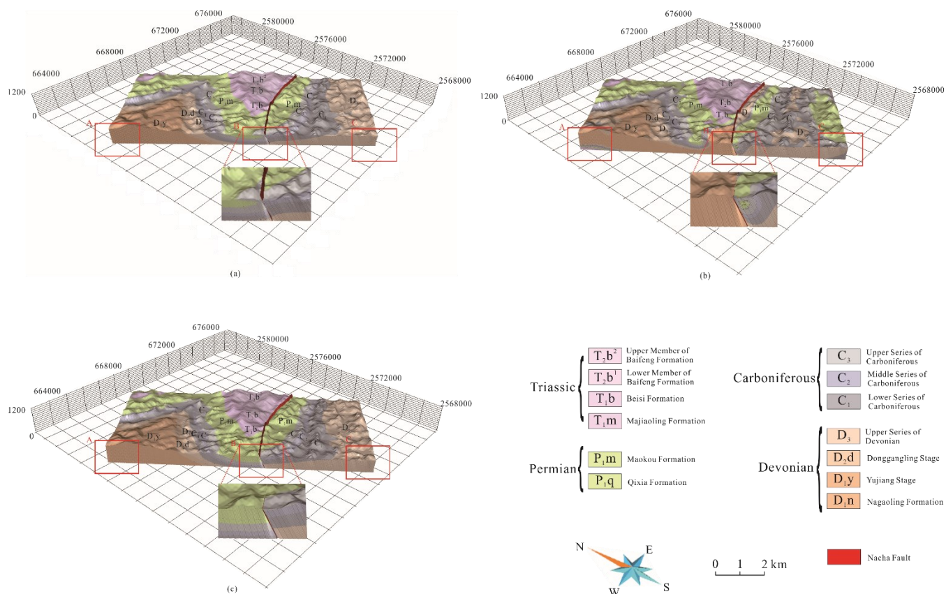
440 445 Figure 17. Three-dimensional stratigraphic models using (a) RBF without gradient constraint, (b) HRBF with unit gradient, and (c) AdaHRBF with optimized gradient magnitude. Many abnormal potential field values and additional unreasonable geological bodies were extracted from the model before optimization, especially in areas A, B, and C as shown in Figs. 17a and 17b. These abnormal potential field values lead to the occurrences of additional strata fragments that do not conform to the rule of sediments.
