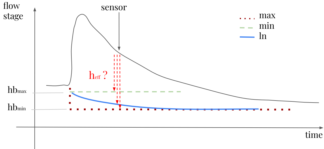
Figure 3. Assumptions on the bed level used to compute the efficient flow height in a natural cross-section: assumption max maximalizes the effective flow height, assumption min minimizes the effective flow height
