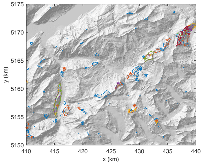
Figure 3. Simulated rockslide sites for a part of Switzerland. In addition to the outlines of the unstable areas, the respective triggering points are also shown for events with V \geq 10^5 \text{ m}^3 . Colors are just used for distinguishing overlapping outlines. Coordinates refer to UTM 32.
