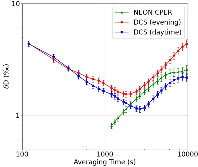
Figure 5: Allan analysis. The overlapping Allan deviation (OADEV) for open-path DCS data from 10/31/2021 when the atmosphere was well-mixed (5:20 am on 10/31/2021 to 3:30 pm on 10/31/2021) is shown with blue squares. The OADEV is 4 ‰ at 120 seconds and averages down with the square root of time to 1.1 ‰ at 3000 seconds. After 3000 seconds, the OADEV rises steeply, likely due to real atmospheric fluctuations. For comparison, the OADEV for the NEON CPER point sensor is shown for the same period (green triangles). The common upward trend in both indicates variation due to atmospheric fluctuations. Finally, the OADEV for a DCS measurement under more typical mixing conditions (from 3:30 pm on 10/31/2021 to 1:30 am on 11/1/2021) is shown with red dots and exhibits the expected higher instability at longer times due to greater atmospheric fluctuation.
