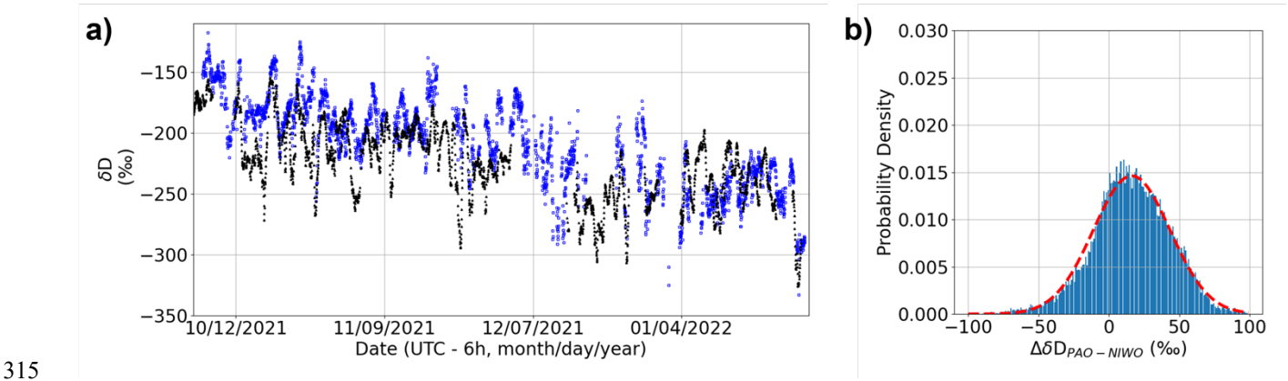
Figure 7: a) Time series of \delta D at PAO (blue) and NIWO (black). b) \Delta\delta D_{\text{PAO-NIWO}} histogram. Red dotted line: fit to Gaussian model (mean = 16 ‰, 1 \sigma width = 27 ‰).
