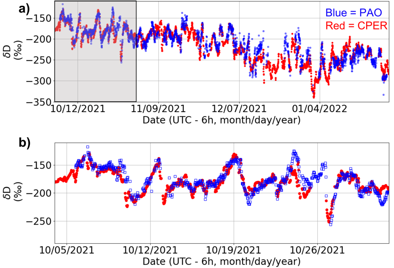
Figure 3: a) Time series of \delta D over the campaign. Blue squares: open-path DCS at PAO. Red dots: NEON point sensor at CPER. b): Zoom-in of time series of \delta D for October 2021 (section highlighted in grey in a)).
