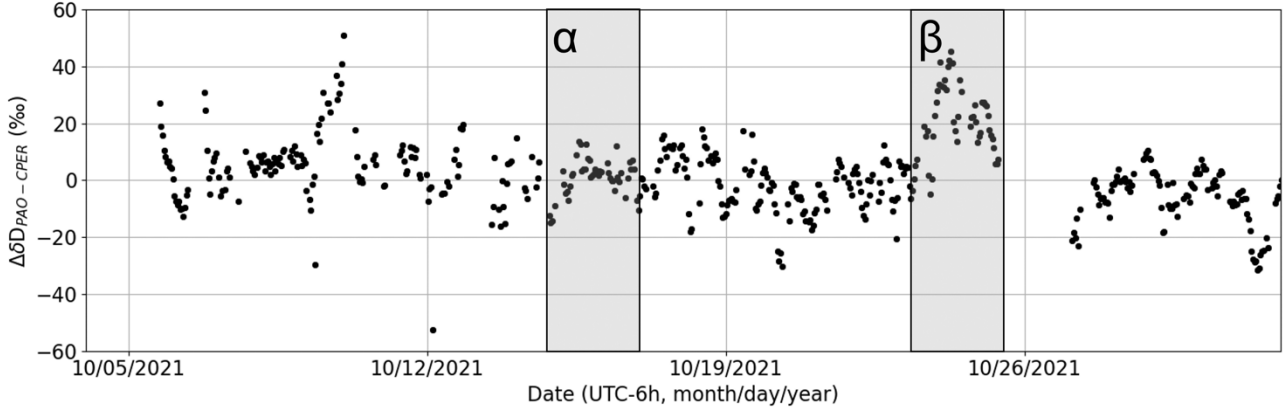
Figure 10: \Delta\delta D_{\text{PA0-CPER}} versus time. Very good agreement is observed during the period denoted \alpha (first grey band), while fairly strong disagreement is seen during the period denoted \beta (second grey band), reaching more than 20 ‰ for about a day.
