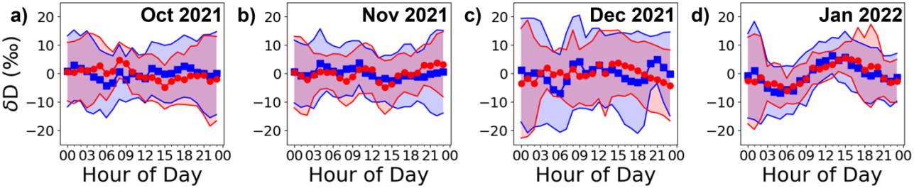
Figure 8: Stacked diurnal cycles for \delta D at PAO (blue) and CPER (red) with mean value subtracted. Shaded regions indicate standard deviation of values in each hourly bin. a) October 2021. b) November 2021. c) December 2021. d) January 2022.
