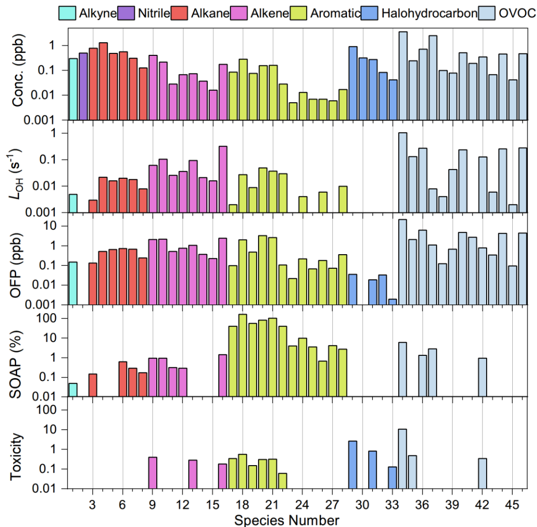
265 Figure 3: 46 VOCs tracers selected for source appointment for PMF analysis and their contribution to TVOCs, L_{OH} , OFP, SOAP and Toxicity if available. At least one tracer for typical VOC emission sources and one VOC tracers from each type of VOCs was included. These selected VOCs contribute to over 90% of TVOCs, L_{OH} , OFP, SOAP and Toxicity. Species number is referred in Table S1.
