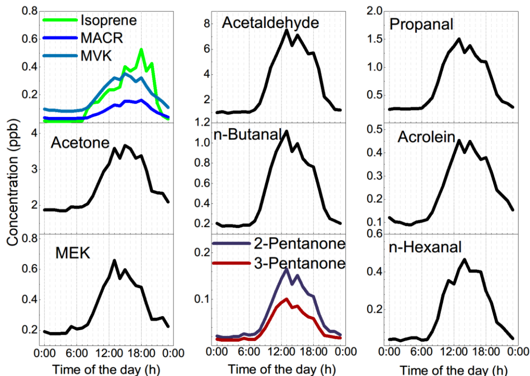
350 Figure 8. Concentration diel profiles of key tracers of the Plant and Secondary Generation.
