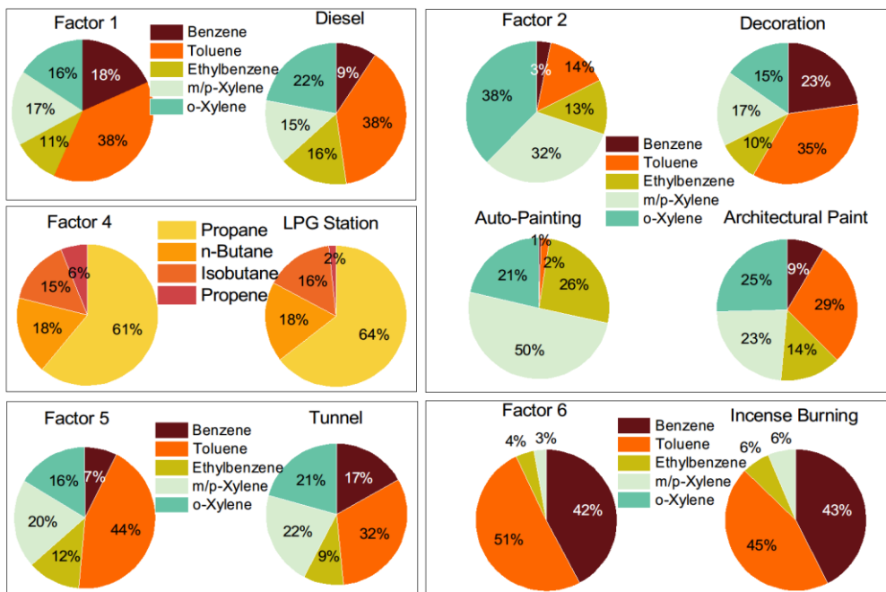
325 Figure 5: Comparison of source spectrums decomposed by PMF with typical source spectrum measured in our study and reported in literature. The data of Auto-Painting and Architectural Paint were from (Yuan et al., 2010).
