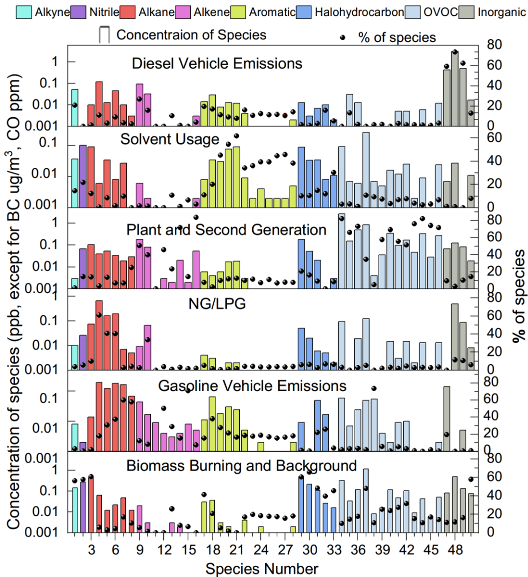
Figure 4: Source factors by PMF decomposition and source identity attribution for the 4 inorganic tracers and 46 VOC tracers. (The concentration units for BC and CO were ug/m 3 and ppm)
