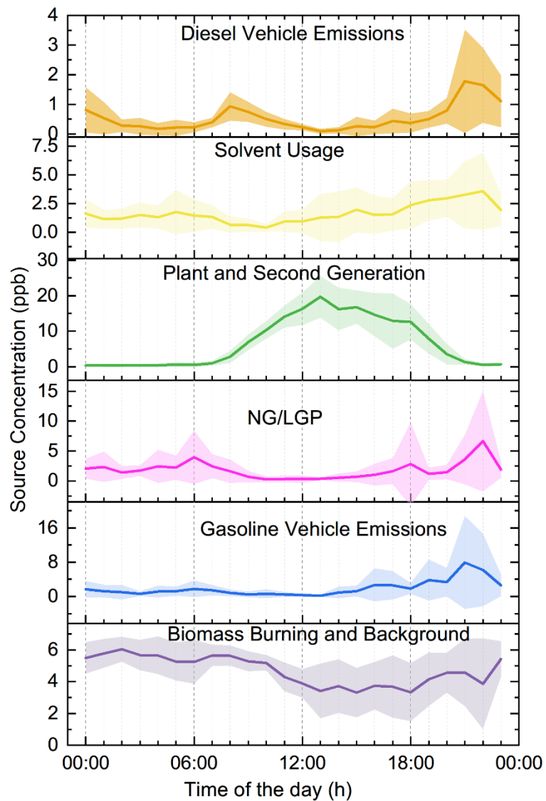
Figure 7: Diel profiles of six decomposed factors.
