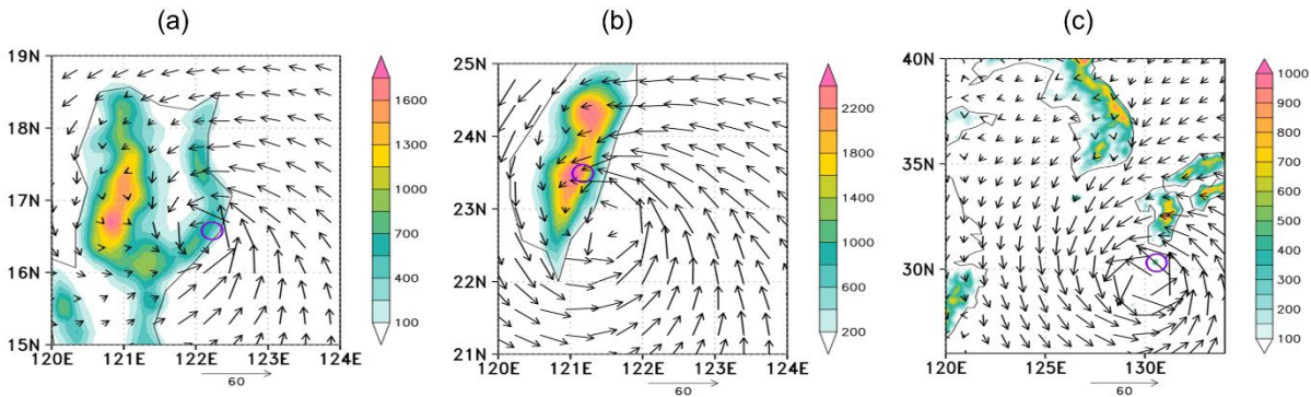
130 Fig. 1 Wind fields (m/s) at the lowest level before model crash from the cases with the initial starting time at a) 18Z 22 July 2020, b) 00Z 22 Sep. 2018 and c) 06Z 2 Sep. 2020. The shading is terrain height (unit: m). The open circles mark the location of the crash.
