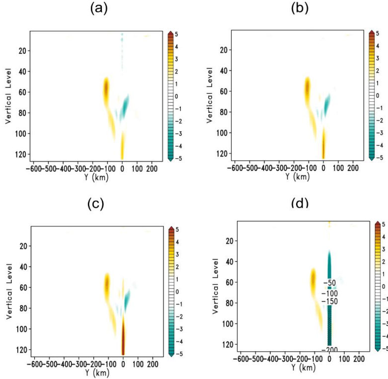
155 Fig. 2 Vertical section of vertical velocity (m/s) through the location of the crash along with the model y-directional grids before the crash for the case with the initial starting time 18Z 18 July 2020. A), b), c), and d) represent 4, 3, 2, and 1 acoustic time step before crash respectively. The y-axis represents the number of vertical levels, with level 1 being at the top of the model.
