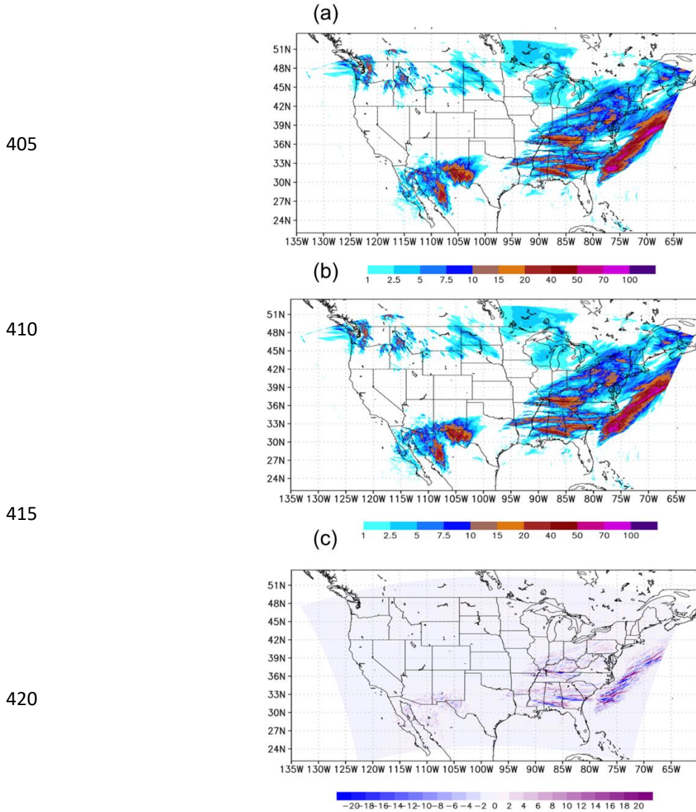
425 Fig. 9 24-hr precipitation (mm) from 12-36 hr in (a) the control and (b) the sensitivity run with zero- gradient BCs. c) is the precipitation difference between these two runs. The control run has the same configuration as the ensemble member one in RRFS with the initial starting time on 00Z March 2, 2020.
