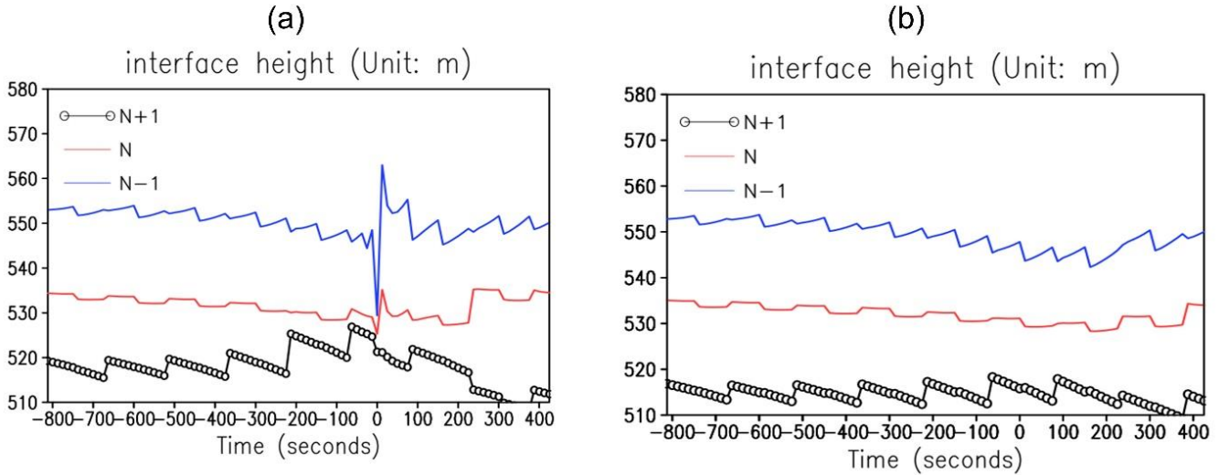
285 Fig. 6 The time series of the geopotential height at the model's three lowest interface layers (marked as N+1, N, N-1 respectively) after the advection at the original crash location in the sensitivity experiments with proposed fixes: a) increased dz_{min} from 2 to 4 and b) zero-gradient BCs for the case with the initial starting time 18Z 18 July 2020.
