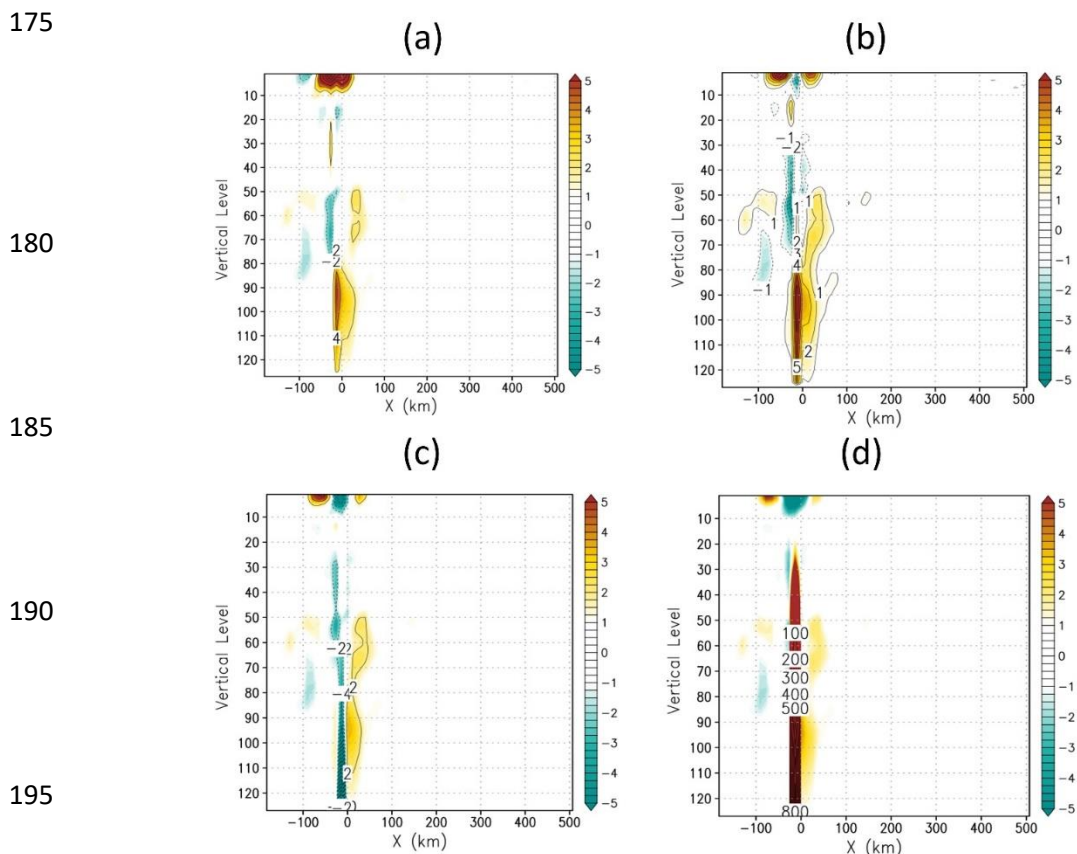
Fig. 3 As Fig. 2 except for the case with an initial starting time of 00Z 22 Sep. 2018 at each acoustic time step before the crash.
