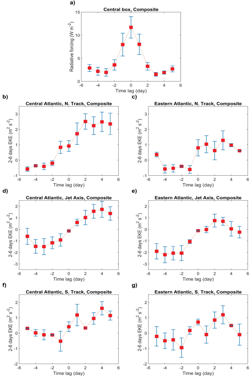
Figure S6 Same as Figure 5, but the dust domain in SAL is selected further downstream over 12^\circ to 22^\circ\text{N} and -38^\circ to -28^\circ\text{E} .
