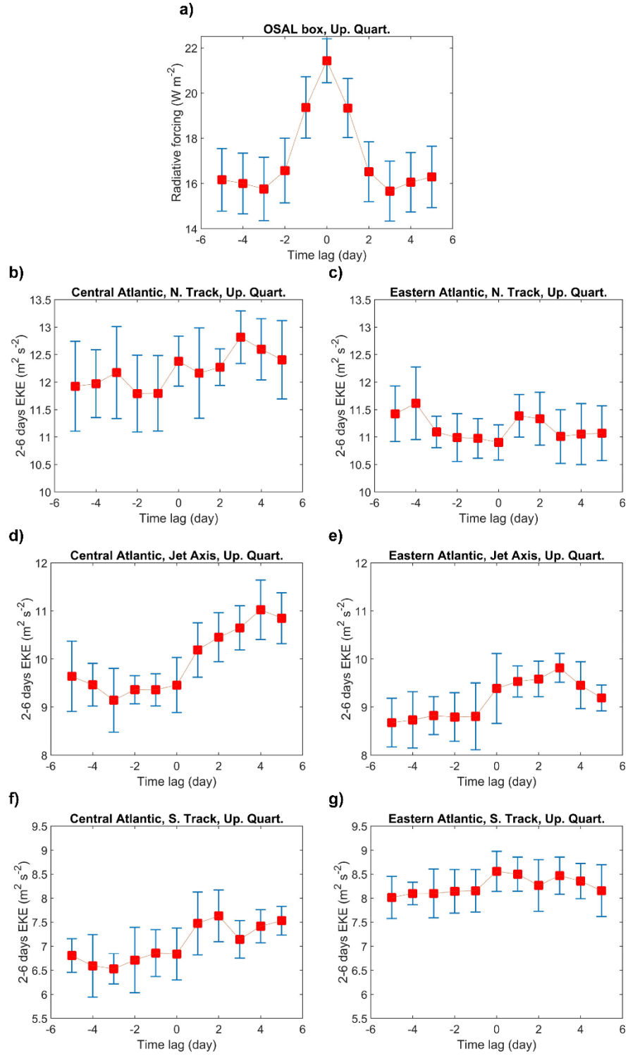
Figure S5 Same as Figure 5, but for the time series of the upper quartile aerosol radiative forcing.
