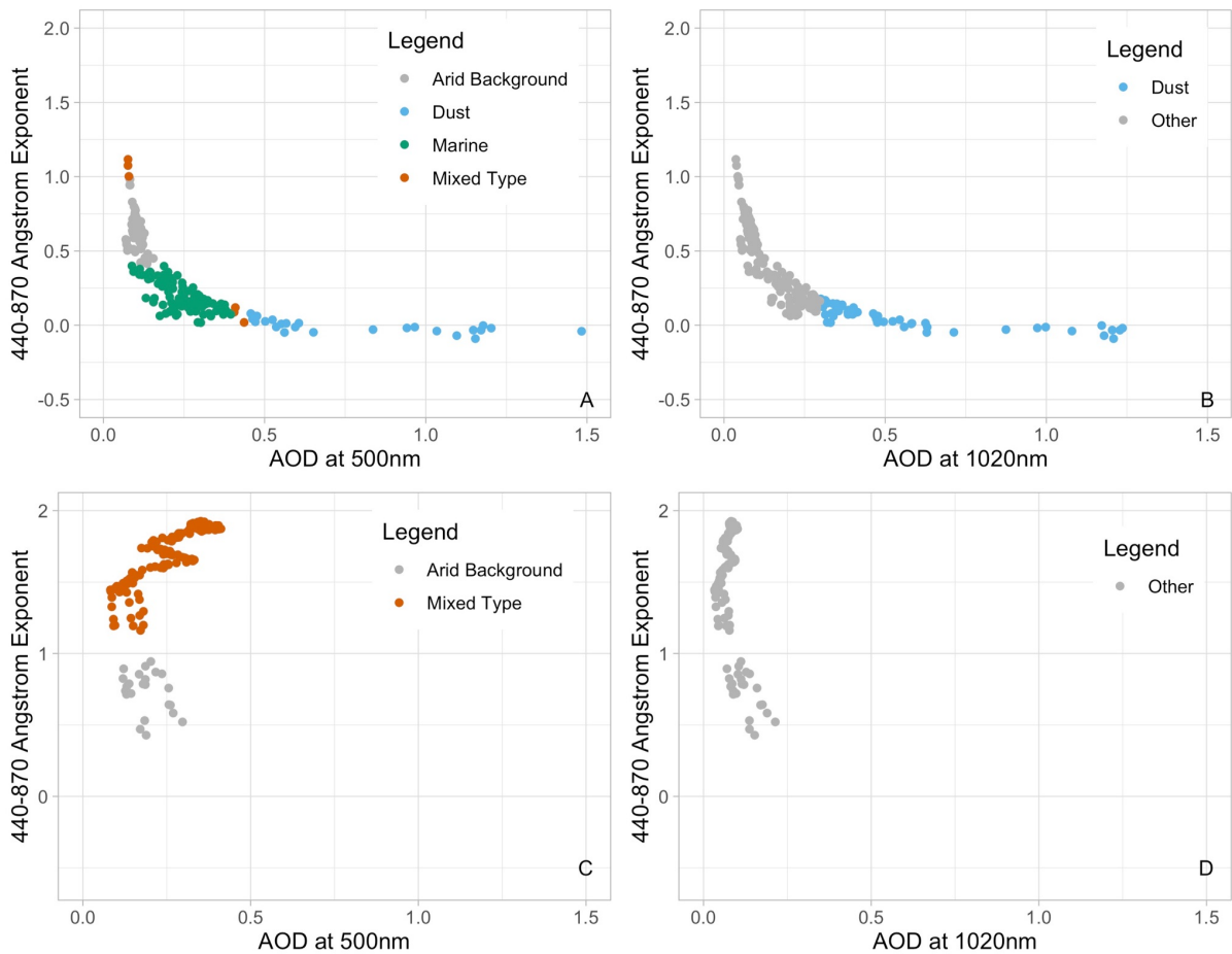
535 Figure 10. Aerosol compositions comparisons at Lhù'àn Mân on a DED - 24/05/2018 (A&B) and a non-dust event day- 23/07/2018 (C&D). Scatterplots A&C are at DQ 1.0 AOD at 500 nm with thresholds from Verma et al. (2015) for broad characterisation of aerosols present at the site. The scatterplots B&D are at DQ 1.0 AOD D with thresholds from Dubovik et al. (2002). In blue is the dust, grey is the arid background, green is marine aerosols, and mixed types are represented in orange.
