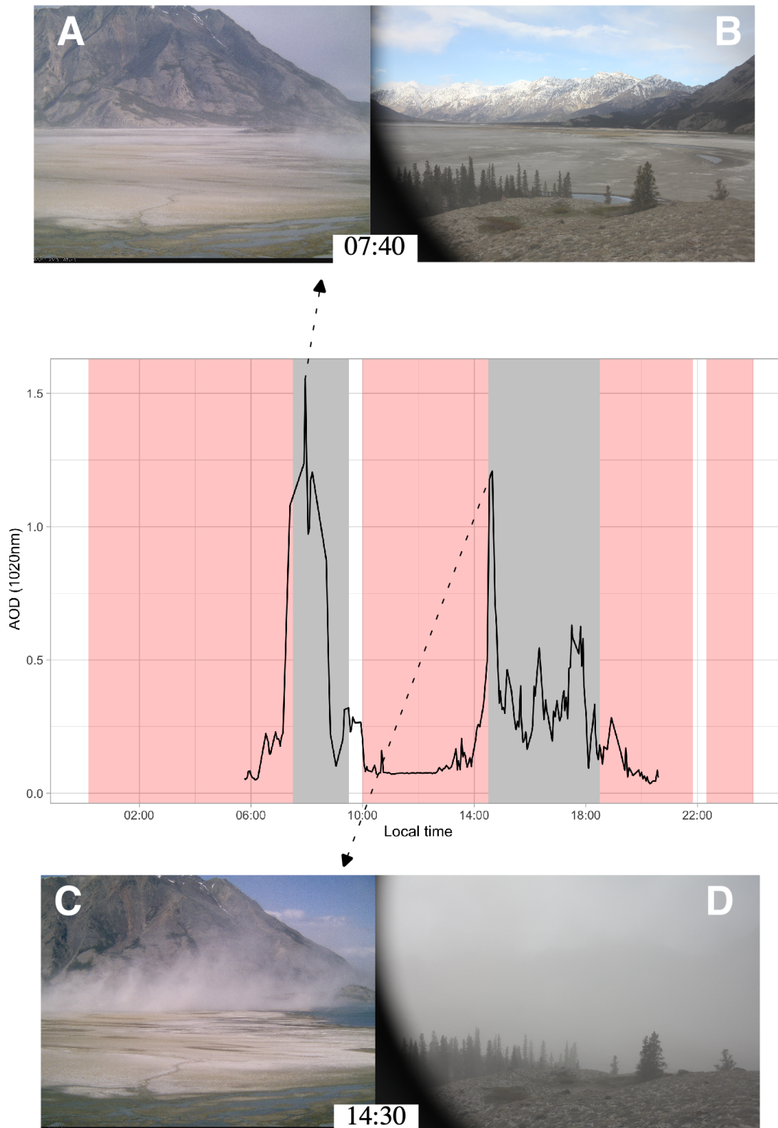
365 Figure 6. AOD D returns from the 24/05/2018 visualised with the corresponding oblique camera images during peak events. In the morning dust is in the southern section of delta. The distance to the mountain from the side camera (panels A&C) is ~5 km and the elevation of the small peak at the top-centre of the image frame is roughly 1100 m above the lake surface. As for the island camera (panels B&D), the closest set of mountains on the right of the frame that are snow-capped are 14 km away and 2270 m asl.
