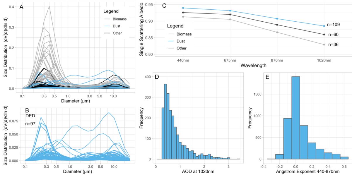
540 Figure 11. (a) Volume size distribution of aerosols at Lhù'àn Mân Recordings that were taken on a DED (DED definition from Dubovik et al. (2002) in the 1020 nm band) are in blue, and recordings taken when there were biomass burning (defined from Verma et al., 2015) events (smoke) are in grey. Any days where dust or smoke were not detected in AERONET are displayed in black. Models used to calculate volume size distribution are based on AERONET level 2.0 DQ with and AOD > 0.4. Dust event days are then pulled out 545 for (b) underneath to show the presence of trimodal dust size. (c) Single scattering albedo for the principal aerosol types recorded at the Lhù'àn Mân AERONET station for 2019 when AOD >0.4. Dust events are in green, biomass burning events are in pink, all other aerosol types are in blue. Models that calculate SSA are based on AERONET level 2.0 DQ. Frequency histograms of AOD (d) and Angstrom exponent (e) at Kluane Lake AERONET station in 2019.
