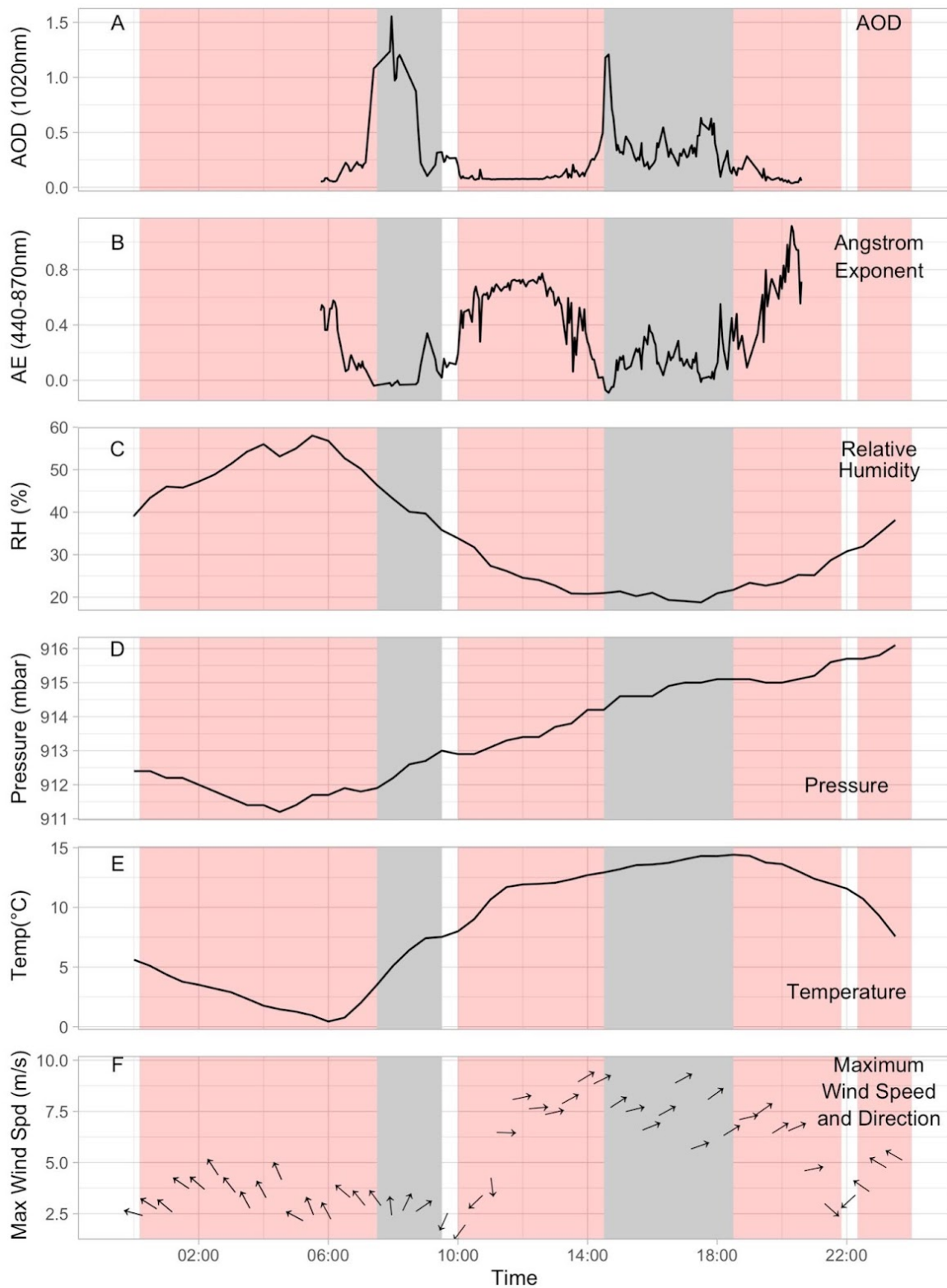
355 Figure 5. Aerosol spectral parameters and meteorological conditions for the 24 th May 2018. Dust events defined by the Dubovic et al. (2002) threshold are highlighted in grey, dust events evident on the oblique imagery are highlighted in pink. Panel (A) is AOD D , panel (B) is DQ 1.0 Angström exponent ( \alpha ) at 440- 870nm, panel (C) is Relative Humidity (%), panel (D) is half hourly pressure (mbar), panel (E) is half hourly temperature (°C) and panel (F) is maximum wind speed (m s -1 ) and direction (°). There are no AERONET 360 AOD returns in DQ 1.5 and 2.0 for this day.
