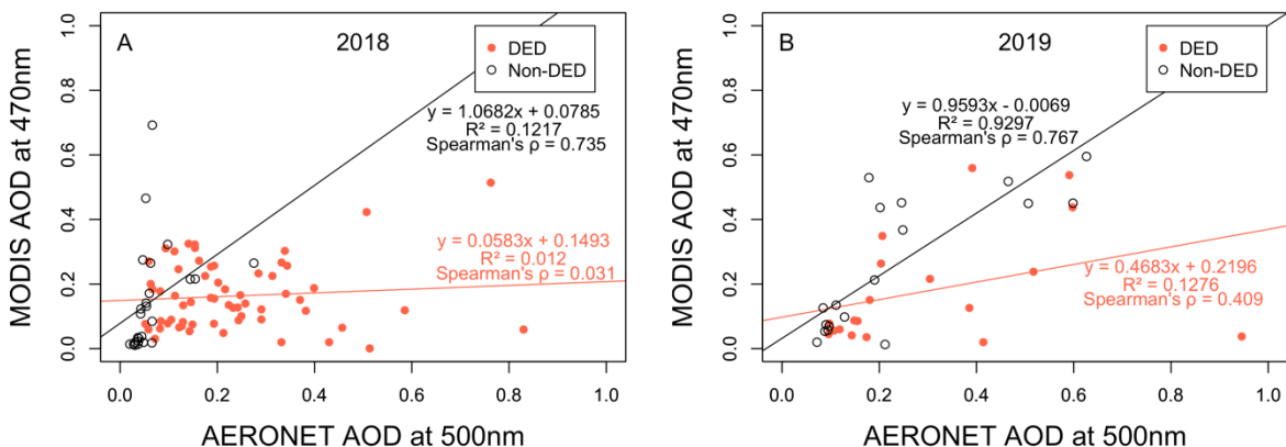
555 Figure 12. Evaluation of daily mean MAIAC v6 1km AOD at 470 nm against daily AERONET mean AOD at 500 nm at Lhù'àn Mân over 2018 (A) and 2019 (B). Note that MAIAC operates using AOD at two wavelengths, 470 nm and 550 nm. 470 nm was chosen due to its relative closeness AERONET AOD at
