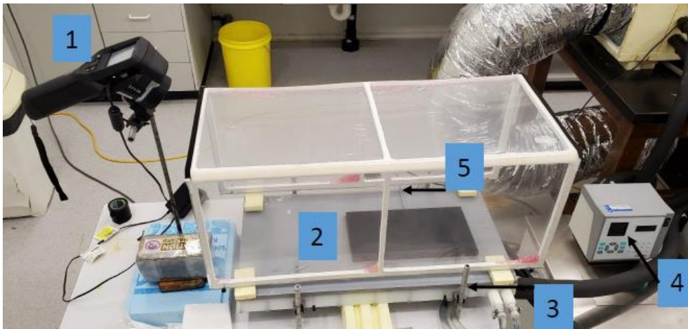
925 Figure B1: Experimental configuration for estimating bulk optical properties of the plastic film. Key numbers as follows: [1] Thermal camera (FLIR: Model E50); [2] Copper plate (painted black); [3] Heat exchanger connected to a [4] constant temperature water bath (Julabo: Model PP50); [5] temperature probe (HART Scientific: Model 1521).
