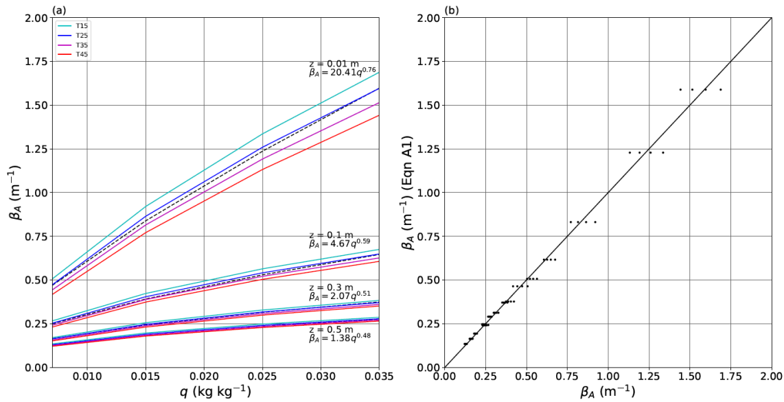
905 Figure A1: Dependence of moist air absorptivity on temperature, specific humidity and thickness of the moist air slab. (a) Moist air absorptivity as a function of specific humidity at different slab thicknesses ( z = 0.01, 0.1, 0.3, 0.5 \text{ m} ) and air temperatures ( T = 15, 25, 35, 45^\circ\text{C} ). Colours (see legend) indicate the temperature and the dashed lines show the indicated equation at each thickness. (b) Predicted moist air absorptivity using Eqn A1 compared with original data. Full line is 1:1. Linear regression is y = 0.997 x + 0.00 , R^2 = 0.99 , \text{RMSE} = 0.039 , n = 64 .
