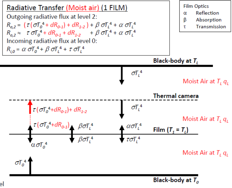
Figure 6: Longwave radiative transfer through one film between two black bodies at temperatures T_0 and T_L modified to account for moist air. The moist air is at the laboratory temperature T_L , with specific humidity q_L .
