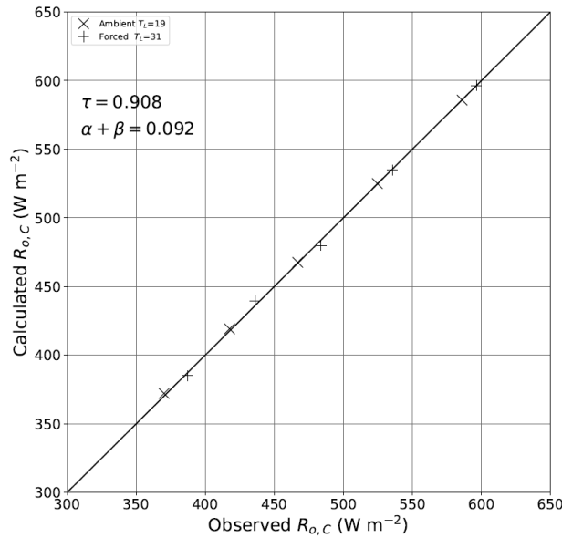
945 Figure B2: Experimental estimate of bulk transmission coefficient of the film. Plot shows calculated versus observed longwave radiation arriving at the thermal camera using least squares estimates for the bulk coefficients ( \tau = 0.908 , \alpha + \beta = 0.092 ) (Linear regression: y = 0.9941x + 2.9 , R^2 > 0.999 , n = 10 , \text{RMSE} = 2.0 \text{ W m}^{-2} ). Full line is 1:1.
