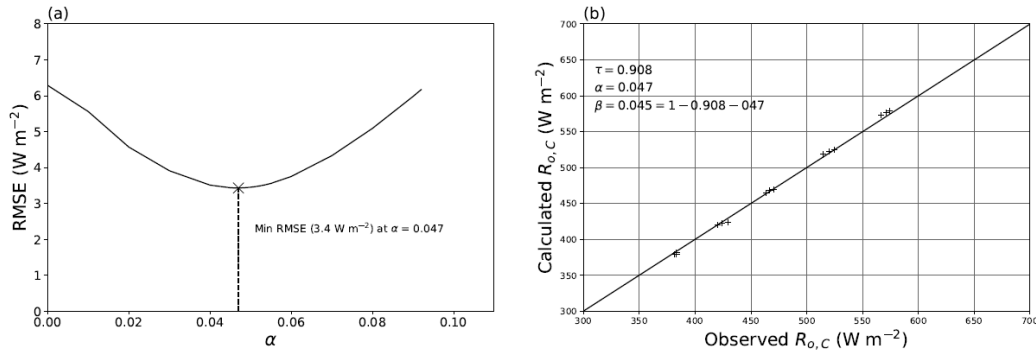
970 Figure B3: Experimental estimate of the bulk reflection ( \alpha ) and absorption ( \beta ) coefficients. (a) RMSE (Eqn B3) as a function of \alpha , and the (b) calculated versus observed longwave radiation arriving at the thermal camera based on the bulk optical properties (Linear regression: y = 1.0445x - 20.5 , R^2 > 0.999 , n = 15 , \text{RMSE} = 3.4 \text{ W m}^{-2} ). Full line is 1:1.
