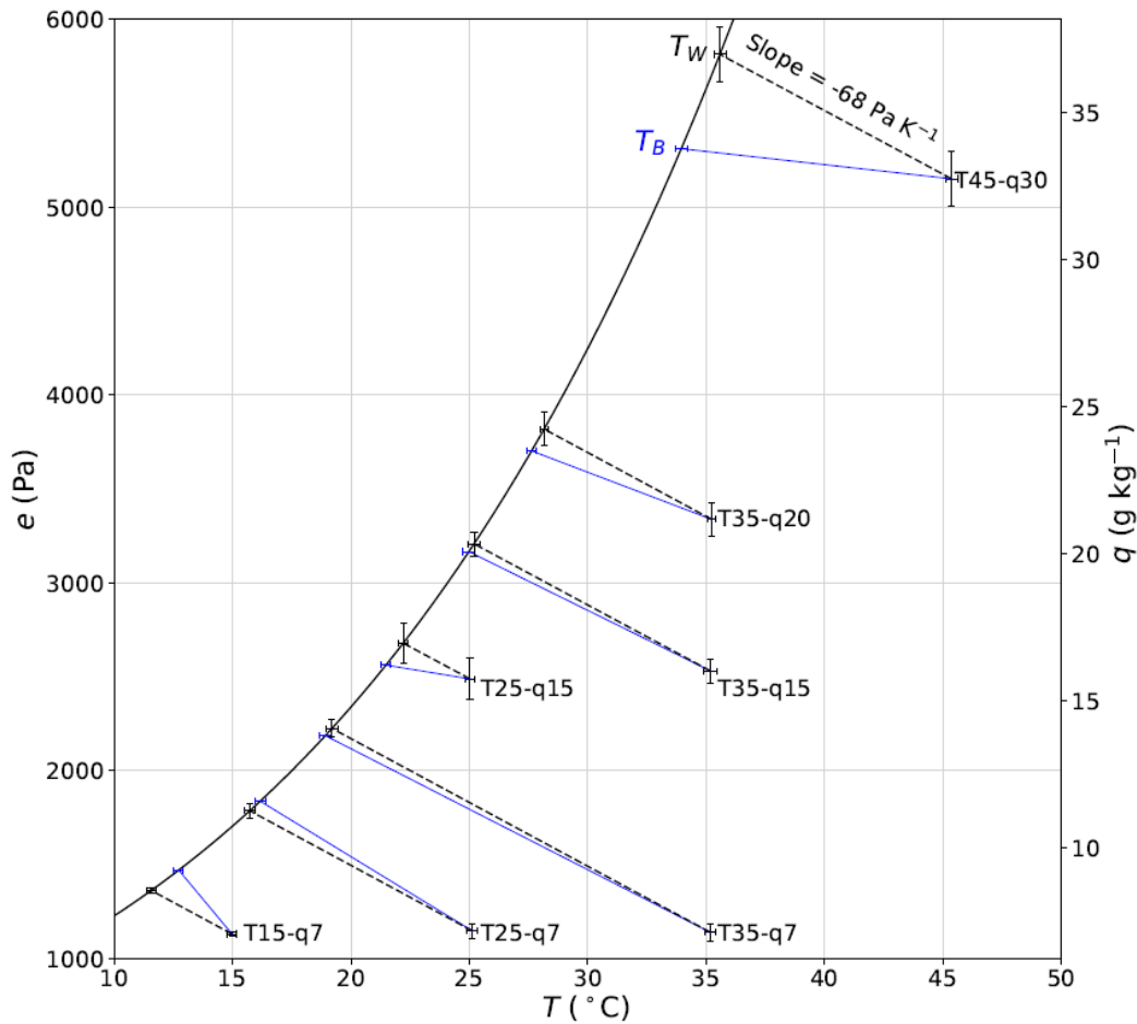
Figure 15: Comparison of observed water bath temperature ( T_B ) with the thermodynamic wet bulb temperature ( T_W ). Plot uses all experimental data at a wind speed of 2 \text{ m s}^{-1} under the ambient forcing ( n = 7 , T15-q7, T25-q7, T35-q7, T25-q15, T35-q15, T35-q20, T45-q30). The dashed black lines join the measured air properties ( T_A, q_A ) to the calculated wet bulb temperature ( T_W ). The full blue lines link with the measured bulk water temperature ( T_B ). The error bars denote \pm 2\text{sd} (i.e., 95% confidence interval). Note that we use the same error bars for T_W as for T_A .
