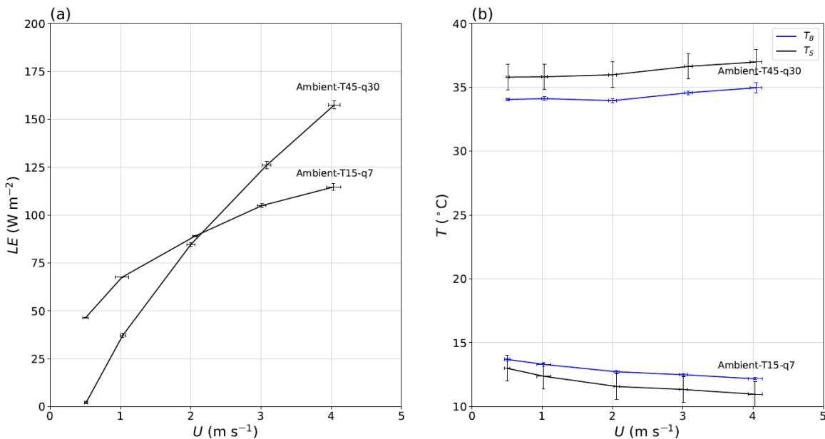
Figure 14: Response of the steady state (a) latent heat flux ( LE ) and (b) water temperature ( T_S , T_B ) to wind speed ( U ) in two typical evaporation experiments. The error bars denote \pm 2\text{sd} (i.e., 95% confidence interval).
