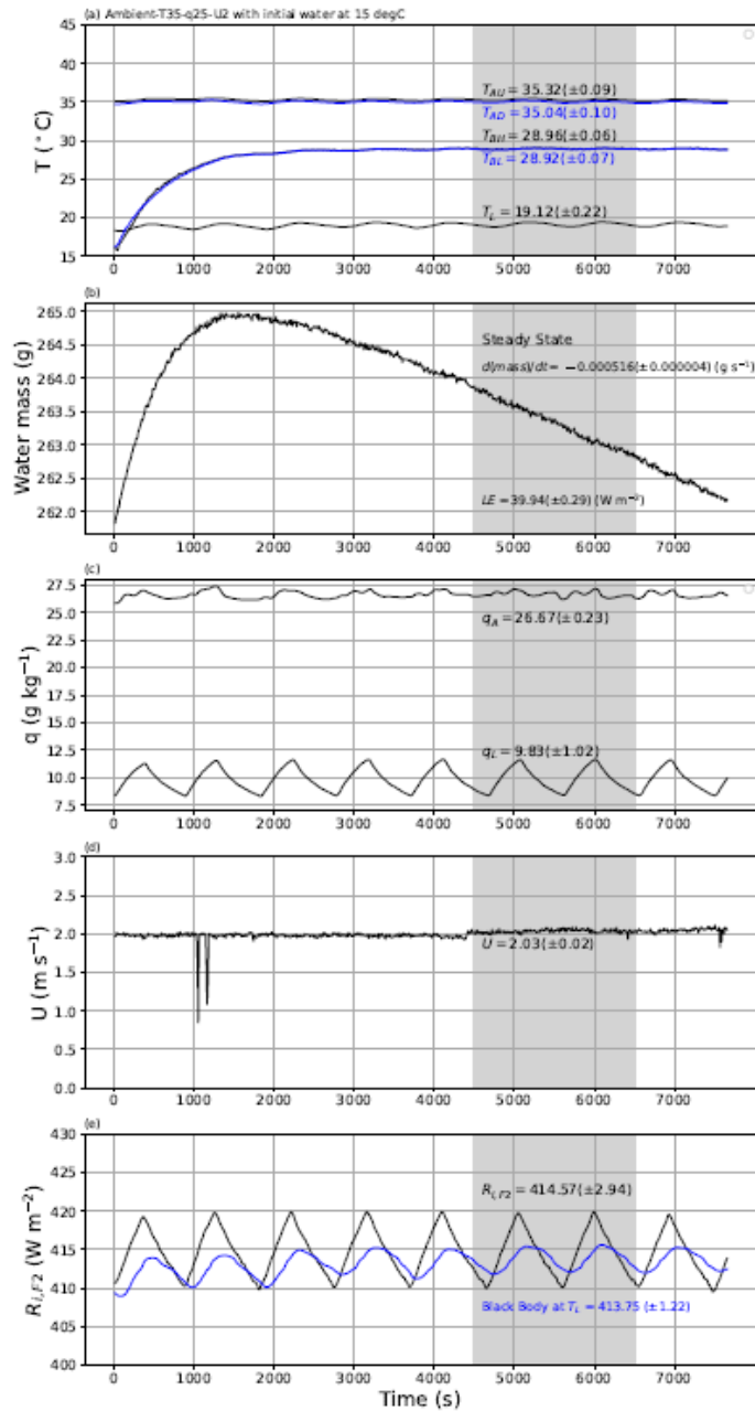
545 Figure 10: An experimental demonstration of the approach to steady state. The experiment began with water at 15°C in the shallow water bath ( T_{BH} , T_{BL} in (a)) with target conditions for air in the tunnel set to Ambient-T35-q25-U2. The plots document the approach to steady state (4500-6500 s) for the evolution of (a) temperature of air in the tunnel ( T_{AU} (black), T_{AD} (blue)), temperature of water in the shallow water bath ( T_{BH} (black), T_{BL} (blue)) and temperature of air in the laboratory ( T_L ), (b) mass of water in shallow water bath with calculated rate of change (via linear regression) and the associated latent heat flux ( LE ), (c) specific humidity of air in the tunnel ( q_A ) and in the laboratory ( q_L ), (d) wind speed ( U ) 550 and (e) the measured incoming longwave radiation at the top of tunnel ( R_{i,F2} ) compared with theoretical black body radiation at laboratory air temperature ( T_L , blue). The numbers on each panel indicate the steady state averages ( \pm 1\text{sd} ).
