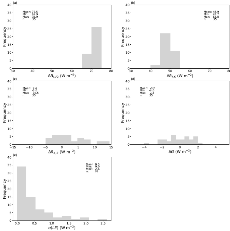
720 Figure 17: Magnitude and uncertainty for the key experimental fluxes. Difference between the forced and ambient paired experiments (n=35) in the incoming longwave radiation (a) at the top of the film ( \Delta R_{i,F2} ), (b) at the water surface ( \Delta R_{i,S} ), (c) outgoing longwave radiation from the water surface ( \Delta R_{o,S} ) and the (d) rate of enthalpy storage in the water bath ( \Delta G ). (e) Steady state standard deviation of the latent heat flux measurements \sigma(LE) taken over all 70 evaporation experiments.
