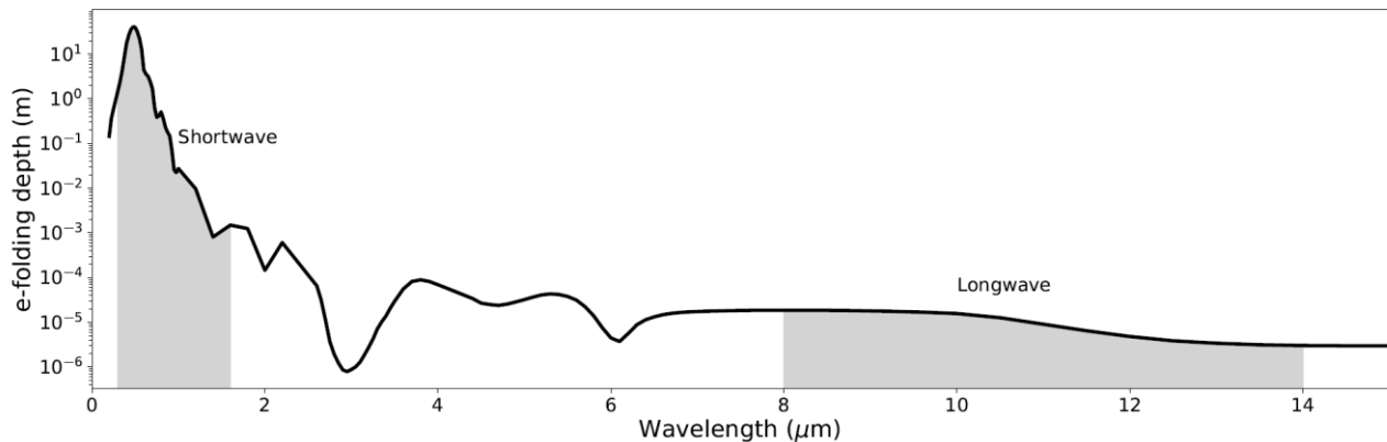
35 Figure 1: Characteristic penetration depth of radiation into liquid water at different wavelengths (Irvine and Pollack, 1968; Hale and Query, 1973). Shaded regions highlight the shortwave (here taken as 0.3-1.6 \mu\text{m} ) and longwave (here taken as 8-14 \mu\text{m} ) regions of the electromagnetic spectrum. Note the log-scale (y-axis).
