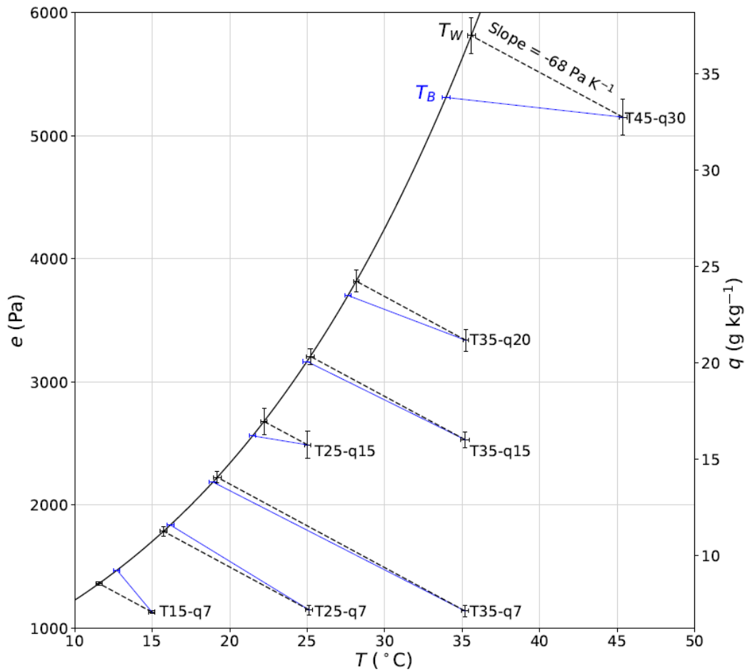
680 Figure 15: Comparison of observed water bath temperature ( T_B ) with the thermodynamic wet bulb temperature ( T_W ). Plot uses all experimental data at a wind speed of 2 \text{ m s}^{-1} under the ambient forcing ( n = 7 , T15-q7, T25-q7, T35-q7, T25-q15, T35-q15, T35-q20, T45-q30). The dashed black lines join the measured air properties ( T_A, q_A ) to the calculated wet bulb temperature ( T_W ). The full blue lines link with the measured bulk water temperature ( T_B ). The error bars denote \pm 2\text{sd} (i.e., 95% confidence interval). Note that we use the same error bars for T_W as for T_A .
