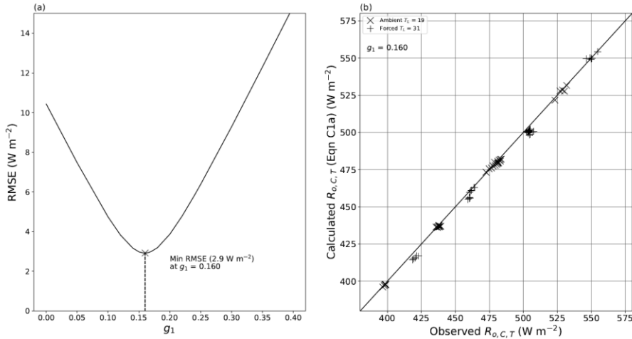
990 Figure C1: Experimental estimate of the geometric parameter g_l . (a) RMSE (Eqn C1a) as a function of g_l highlighting the identified minimum value. (b) Comparison of observed and calculated outgoing longwave radiation arriving at the thermal camera from the calibration spot using the optimal value for g_l ( = 0.160 ) (Linear regression: y = 1.002 x - 2.9 , R^2 = 0.997 , RMSE = 2.9 W m^{-2} , n = 70 ). Full line is 1:1.
