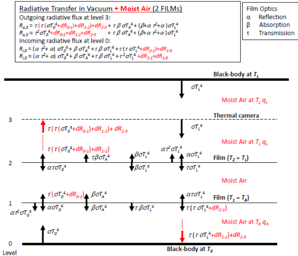
410 Figure 7: Longwave radiative transfer through two films between two black bodies at temperatures T_0 and T_L . The intervening space is occupied by moist air in the tunnel ( T_A, q_A ) or the laboratory ( T_L, q_L ) with the assumed temperature of each film as noted.
