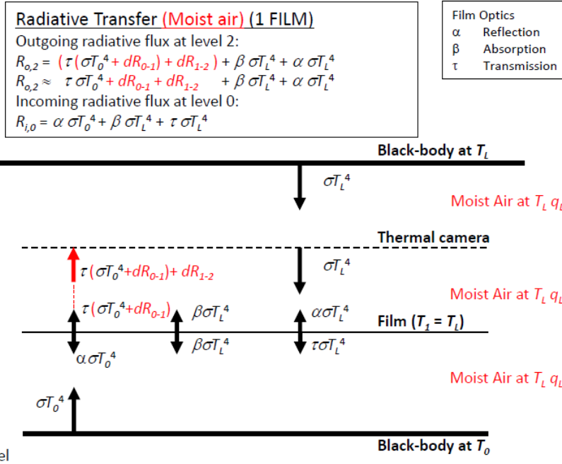
360 Figure 6: Longwave radiative transfer through one film between two black bodies at temperatures T_0 and T_L modified to account for moist air. The moist air is at the laboratory temperature T_L , with specific humidity q_L .
