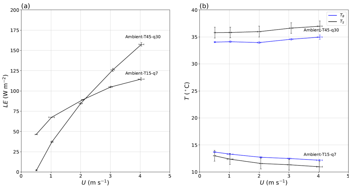
Figure 14: Response of the steady state (a) latent heat flux ( LE ) and (b) water temperature ( T_S , T_B ) to wind speed ( U ) in two typical evaporation experiments. The error bars denote \pm 2sd (i.e., 95% confidence interval).
