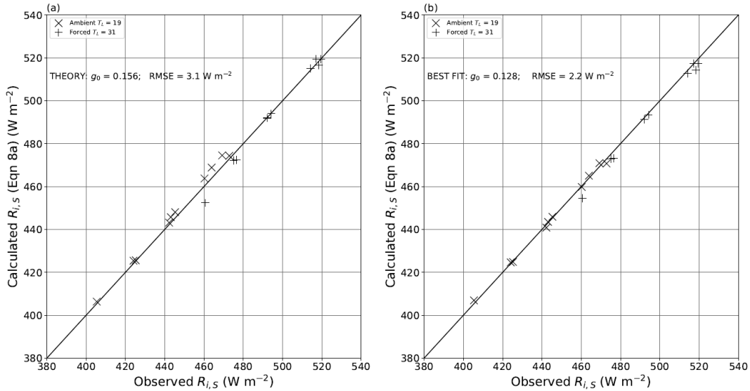
465 Figure 9: Comparison of theoretical (Eqn 8a) and observed incoming longwave radiation at the water surface. (a) Uses g_0 = 0.156 as per theory (Linear regression: y = 0.9855x + 7.3 , R^2 = 0.991 , \text{RMSE} = 3.1 \text{ W m}^{-2} , n=20 ). (b) Tuned to locate the value of g_0 (=0.128) with the lowest RMSE (Linear regression: y = 0.9772x + 9.7 , R^2 = 0.997 , \text{RMSE} = 2.2 \text{ W m}^{-2} , n=20 ). Full lines are 1:1.
