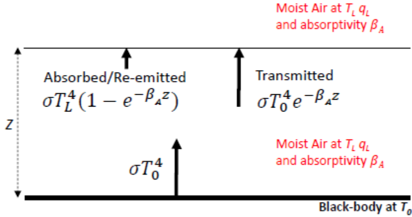
Figure 5: Underlying principle of the moist air correction ( dR ). The fate of the emitted black body flux ( \sigma T_0^4 ) passing through a slab (thickness z ) of moist air (at T_L, q_L ) having longwave absorptivity \beta_A .
