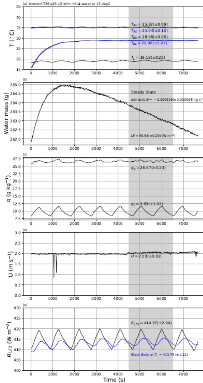
Figure 10: An experimental demonstration of the approach to steady state. The experiment began with water at 15°C in the shallow water bath ( T_{BH} , T_{BL} in (a)) with target conditions for air in the tunnel set to Ambient-T35-q25-U2. The plots document the approach to steady state (4500-6500 s) for the evolution of (a) temperature of air in the tunnel ( T_{AU} (black), T_{AD} (blue)), temperature of water in the shallow water bath ( T_{BH} (black), T_{BL} (blue)) and temperature of air in the laboratory ( T_L ), (b) mass of water in shallow water bath with calculated rate of change (via linear regression) and the associated latent heat flux ( LE ), (c) specific humidity of air in the tunnel ( q_A ) and in the laboratory ( q_L ), (d) wind speed ( U ) and (e) the measured incoming longwave radiation at the top of tunnel ( R_{i,F2} ) compared with theoretical black body radiation at laboratory air temperature ( T_L , blue). The numbers on each panel indicate the steady state averages ( \pm 1\text{sd} ).
