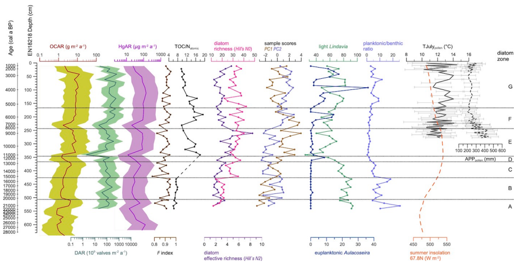
Figure 8: Biogeochemical variables and statistical diatom indices since the Late Pleistocene from Lake Rauchagytygn sediment core EN18218. OCAR, organic carbon accumulation rates; DAR, diatom accumulation rates; HgAR, mercury accumulation rates; F index, diatom valve preservation index; TOC/TN atomic , total organic carbon to total nitrogen ratio; diatom species richness based on Hill numbers; PC1-3, main axes sample scores from the principal component analysis; light 'cyclotelloid' Lindavia and euplanktonic Aulacoseira as sum percentages; planktonic to benthic species ratios; paleoclimate information from published literature at the right. Reconstructed July temperatures and precipitation
