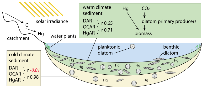
880 Figure 11: Schematic drawing of the long-term processes leading to accumulation of diatom valves (DAR), organic carbon (OCAR), and mercury (HgAR) in Lake Rauchagytygn. Pearson correlation coefficients indicated by r in black when correlation was significant ( p < 0.05 ), and in red italic when p > 0.05 (insignificant).
