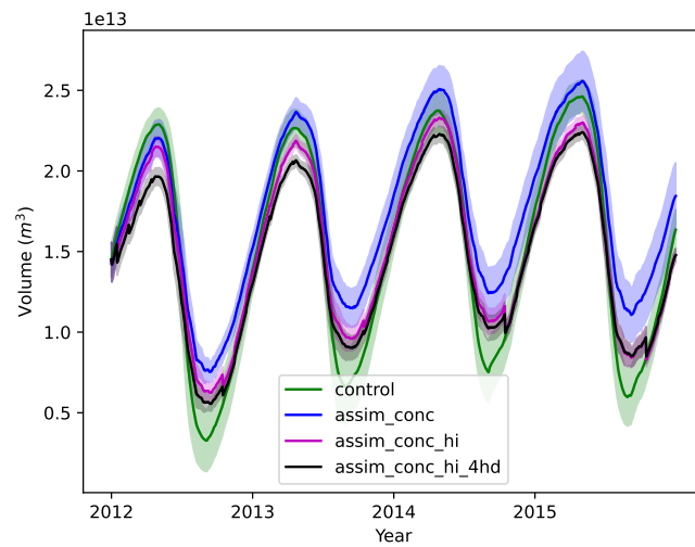
Figure 11. Pan-Arctic sea ice volume from 2012-2015 in four different CICE-PDAF runs. Solid lines show observations or ensemble mean and the shading shows observation error or ensemble spread (one standard deviation).
