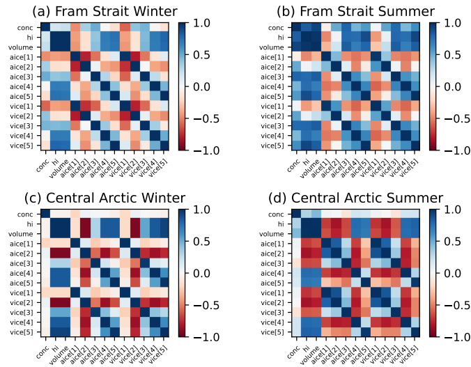
Figure 4. Correlation matrices of CICE state variables: fraction of ice in category n (aice[n]), volume of ice per unit grid cell in category n (vice[n]), as well as the total sea ice concentration (conc), grid cell mean ice thickness (hi) and total grid cell sea ice volume (volume) in January 2012 and July 2012 in the Fram Strait and the Central Arctic.
