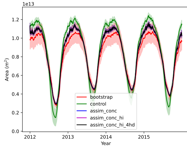
Figure 10. Pan-Arctic sea ice extent from 2012-2015 from Bootstrap observations and four different CICE-PDAF runs. Solid lines show observations or ensemble mean and the shading shows observation error or ensemble spread (one standard deviation)
