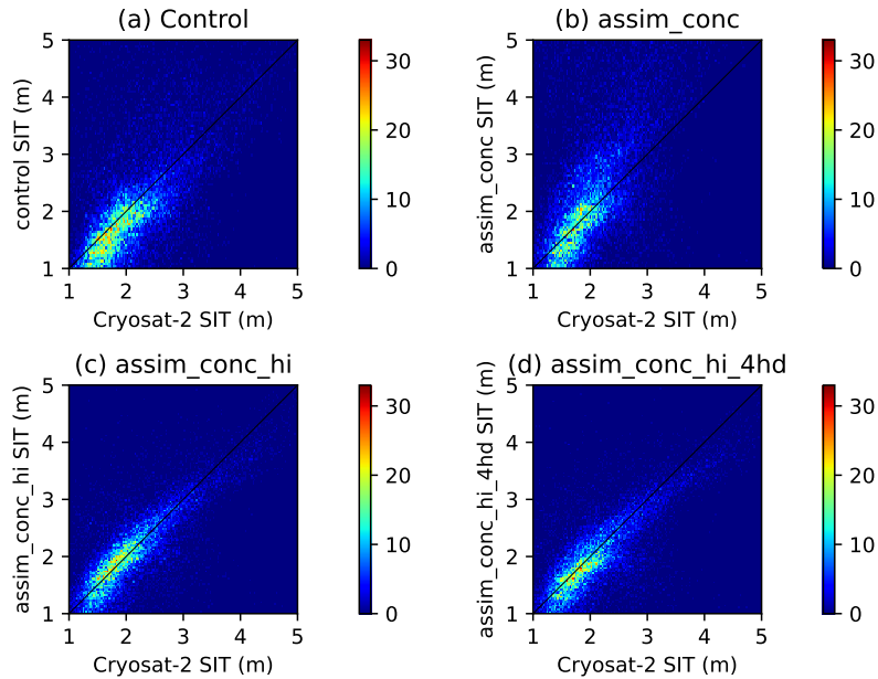
Figure 7. 2d histogram plots of sea ice thickness estimates in CICE-PDAF against the Cryosat-2 CryoSat-2 evaluation data for four CICE-PDAF experiments.
