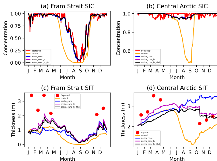
Figure 5. Sea ice concentration and mean sea ice thickness in one grid cell in the Fram Strait and the Central Arctic in CICE-PDAF, Bootstrap and Cryosat-2 CryoSat-2 in 2012.
