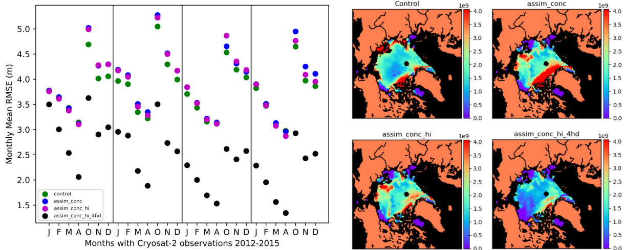
Figure 8. LHS: RMSE of Category 5 sea ice thickness between 2012 and 2015 for January, February, March, April, October, November and December for the control and CICE-PDAF assimilation runs, against CryoSat-2 sea ice thickness evaluation data. RHS: Maps of category 5 sea ice volume RMSE in December 2013 for four CICE-PDAF runs against CryoSat-2 evaluation data. Clockwise from the top left map: control run, assim_conc, assim_conc_hi_4hd and assim_conc_hi.
