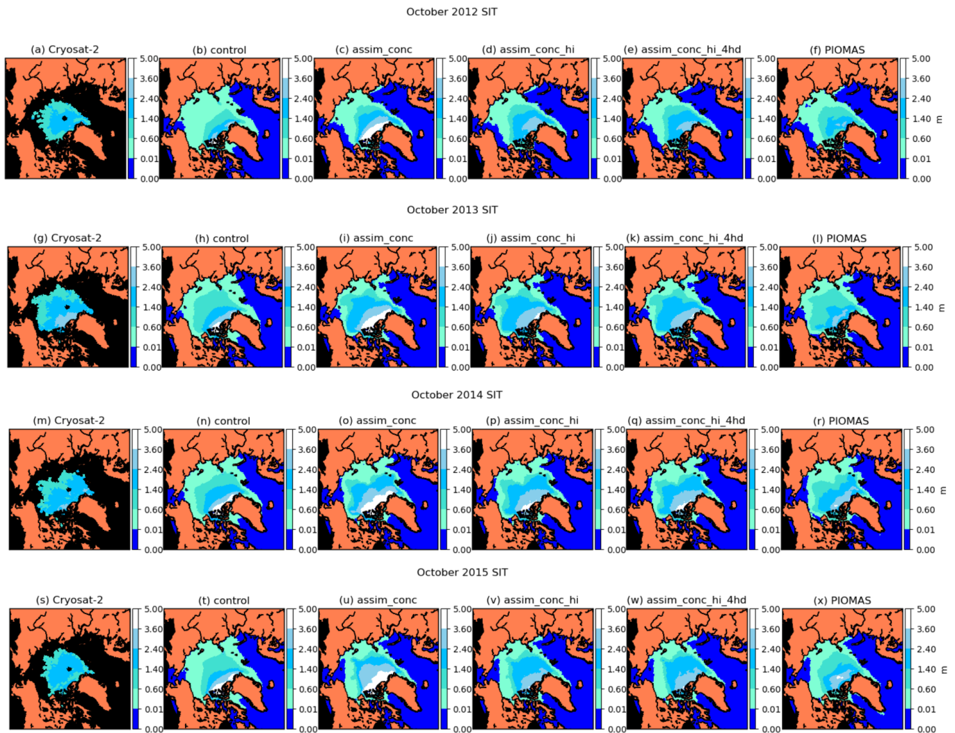
Figure 12. Monthly mean sea ice thickness (in metres) in October 2012, 2013, 2014 and 2015 in Cryosat-2 CryoSat-2 and our CICE-PDAF experiments (ensemble mean) and PIOMAS.
