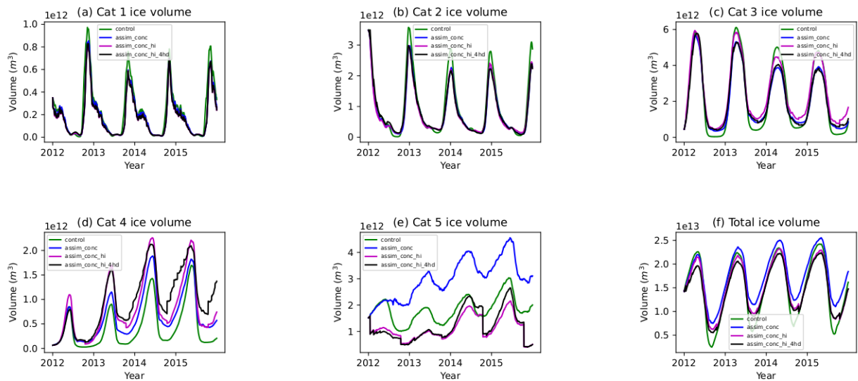
Figure 14. Volume of ice in each thickness category and the total volume for each of the CICE-PDAF experiments (ensemble mean).
