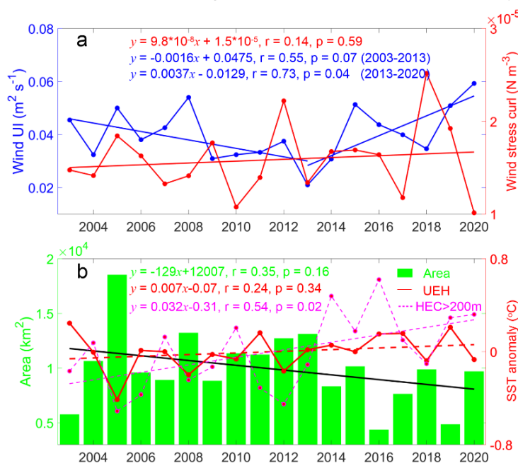
Figure 4. Time series of Upwelling index (UI) and upwelling characteristics. (a) Time series of mean
