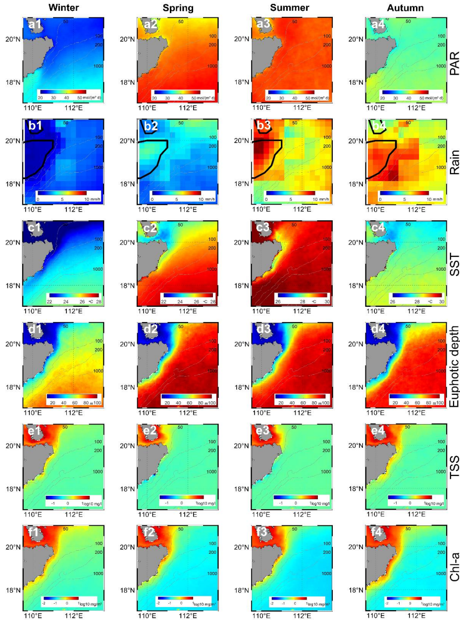
217 218 Figure 3. Seasonal climatological (a1–a4) PAR, (b1–b4) rainfall, (c1–c4) SST, (d1–d4) euphotic 219 depth, (e1–e4) TSS, and (f1–f4) Chl-a. The columns correspond to winter, spring, summer and 220 autumn. The unit of the numbers on the isobaths is meters.
