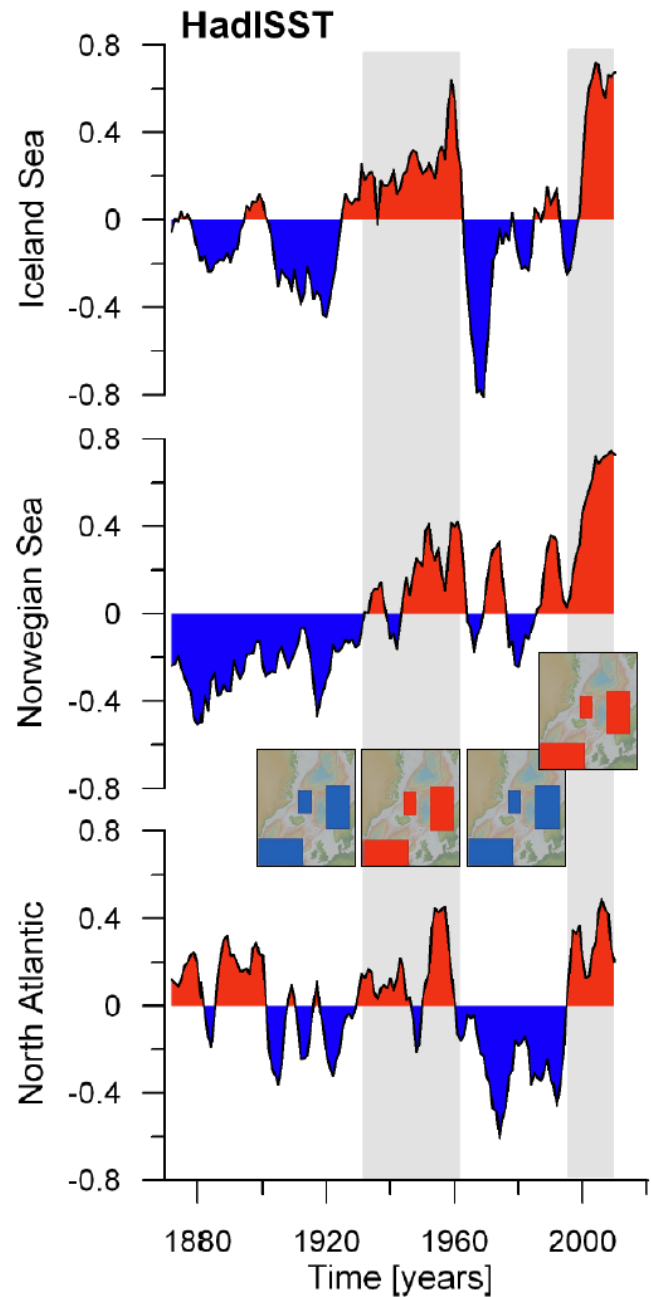
Figure 6 Annual SST anomalies for the North Atlantic, Norwegian and Iceland Seas based on HadISST data. SSTs have been averaged over the three box regions before calculating the anomalies: 49-57°N and 14-35°W (North Atlantic), 62.5-73°N and 0-16°E (Norwegian Sea), 66-72°N and 10-18°W (Iceland Sea). A running mean with a 5-year window has been applied on the time series and the anomalies are shown relative to the mean of the 5-year running mean filtered time series (1870-2012). The map inserts provide a conceptual representation of the results, with blue (red) boxes representing cold (warm) SST anomalies for the North Atlantic, Norwegian and Iceland Seas. The grey bars highlight the periods with positive spatially coherent SST anomalies. The base for the map inserts is made with GeoMapApp ( www.geomapapp.org ) / CC BY / CC BY (Ryan et al., 2009)).
