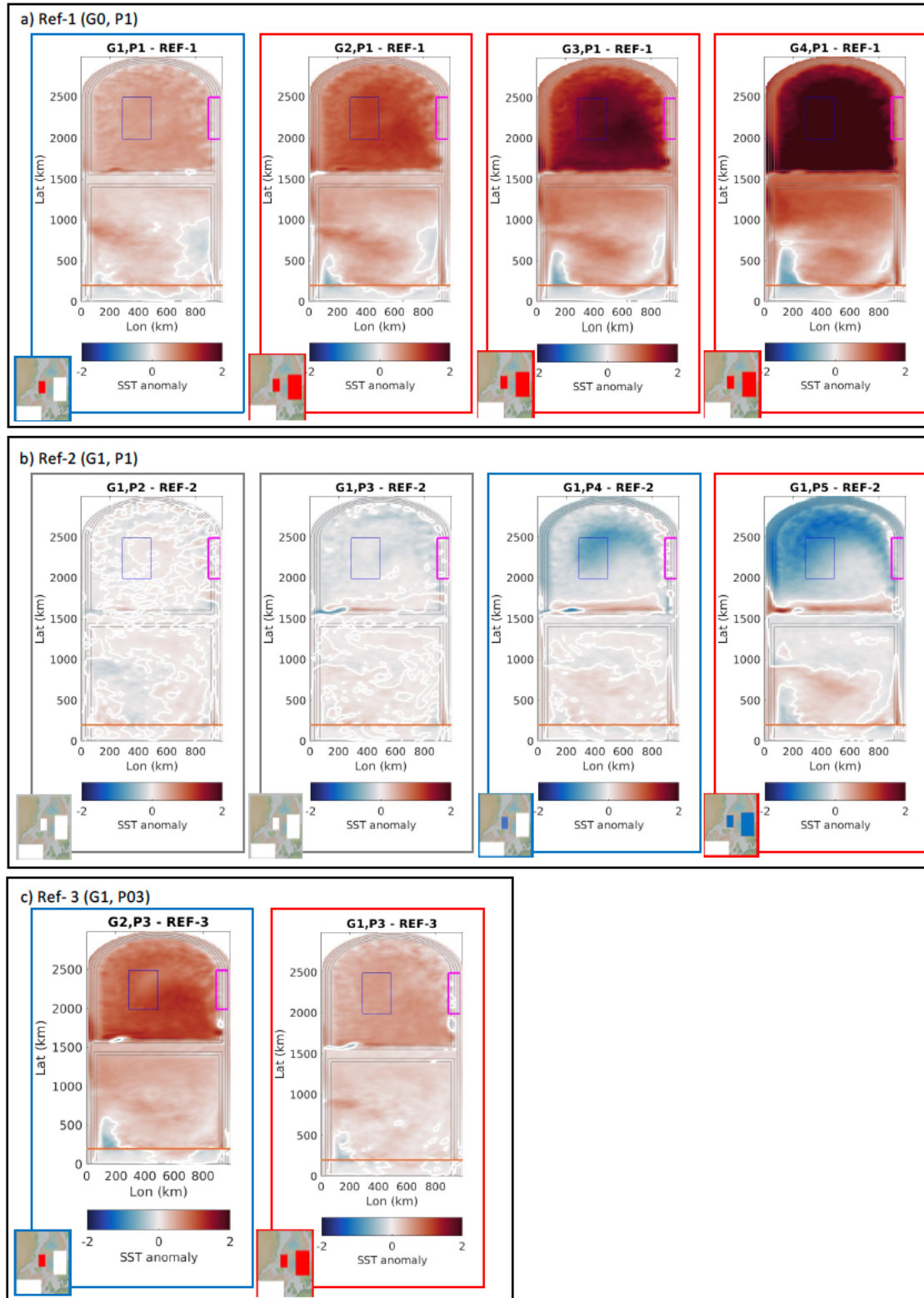
Figure 9 SST anomalies seen in MITgcm idealized experiments. White mark the zero-contour line. a) SST anomalies relative to REF-1, where freshwater is kept constant at P1 while SAT is gradually increased (G1-G4). b) SST anomalies relative to REF-2, where SAT is kept constant at G1 while freshwater is gradually increased (P2-P5). c) SST anomalies relative to REF-3, where freshwater is kept constant at P3 while SAT is increased (G1 and G2). Surrounding blue boxes represent an Iceland Sea SST anomaly spatially incoherent with the North Atlantic and the Norwegian Sea anomalies. The SST anomaly seen in the Iceland Sea exceeds 2 \times \text{std} of the relevant reference experiment. Surrounding red boxes represent a North Atlantic SST anomaly spatially incoherent with the Norwegian and Iceland Seas anomalies. The SST anomalies seen in the Norwegian and Iceland Seas exceeds 2 \times \text{std} of the relevant reference experiment. Surrounding grey boxes represent spatially coherent SST anomalies between the three regions (none of the SST anomalies exceeds 2 \times \text{std} of the relevant reference experiment). Conceptualized representation of the resulting SST
