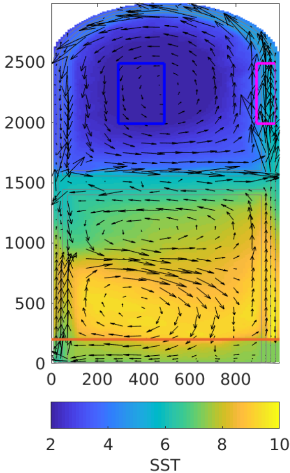
Figure 5 Example of SSTs (colours) and upper 500 m ocean circulation (black arrows) for the MITgcm experiments. The indicated boxes show the areas used to calculate the SSTs of the Norwegian Sea (pink) and the Iceland Sea (blue) used in Table 1. The domains are set for the results to be comparable to the reconstructions, observations and CMIP6 results. Since the MITgcm is idealized the domains can, however, not be identical to the domains defined in Section 2.1. The North Atlantic restoring region equals the area south of the red line in.
