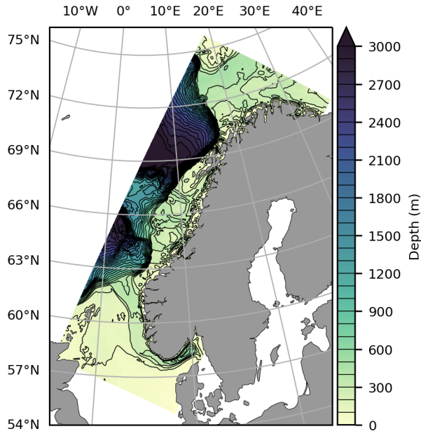
Figure 1. Bathymetry of the model region covering the shelf seas and shelf break off Norway.
