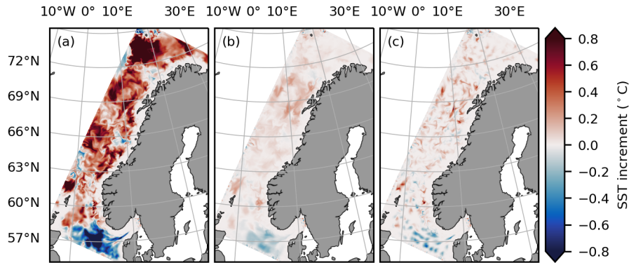
Figure 7. SST increments at the last time step in the first assimilation window. Increments of experiments (a) PMW1 and (b) PMW2. (c) increments if PMW1 assimilates observations thinned in the same way as the observations used in PMW2.
