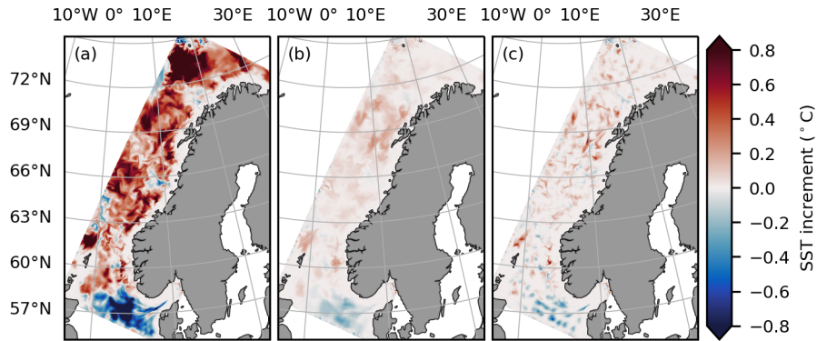
Figure 7. SST increments at the last time step in the first assimilation window. Increments of experiments (a) PMW1 and (b) PMW2, and (c) increments if PMW1 assimilates observations thinned in the same way as the observations used in PMW2 PMW1-thinned.
