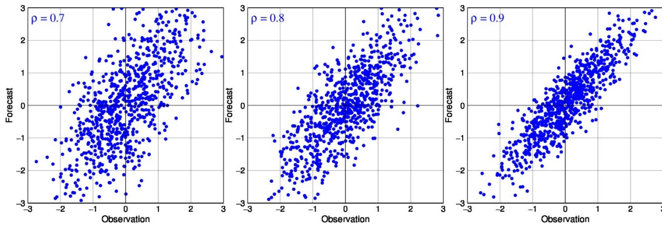
Figure 1: Joint probability distributions of forecasts and observations with different values of \rho under the additive error model.
