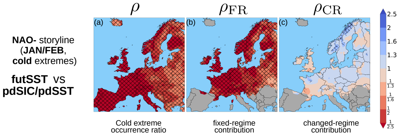
Figure 9. Similar to Fig. 6, but comparing the pdSIC/pdSST reference simulation and the futSST sensitivity simulation. Blue indicates more frequent cold extreme occurrences, and red indicates less frequent cold extreme occurrences in futSST. Analyzed are cold extremes in January/February and a NAO- storyline is assumed here. \rho_{FR} and \rho_{CR} are only plotted for regions where statistically significant preferred winter cold extreme occurrences during NAO- days were identified in Fig. 3c.
