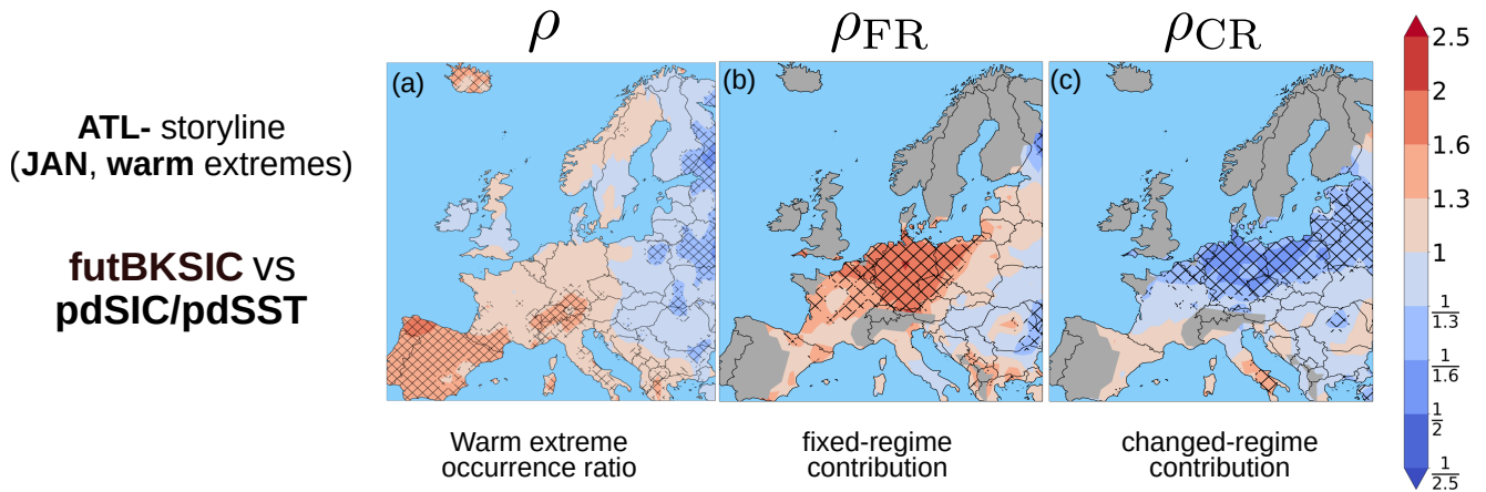
Figure 7. Same as in Fig. 6 (futBKSIC vs. pdSIC/pdSST simulation) but for January warm extremes and along a ATL- regime storyline. Compared to Fig. 6 the color bar is reversed, such that red indicates more frequent warm extreme occurrences, and blue indicates less frequent warm extreme occurrences in futBKSIC. Occurrence ratio of ATL- regime occurrence in January is given as \rho_{\text{circ}} = 0.8 . Thus, the ATL- occurs less frequent in the futBKSIC simulation (see also Fig. S2i). \rho_{\text{FR}} and \rho_{\text{CR}} are only plotted for regions where statistically significant preferred winter warm extreme occurrences during ATL- days were identified in Fig. 3i.
