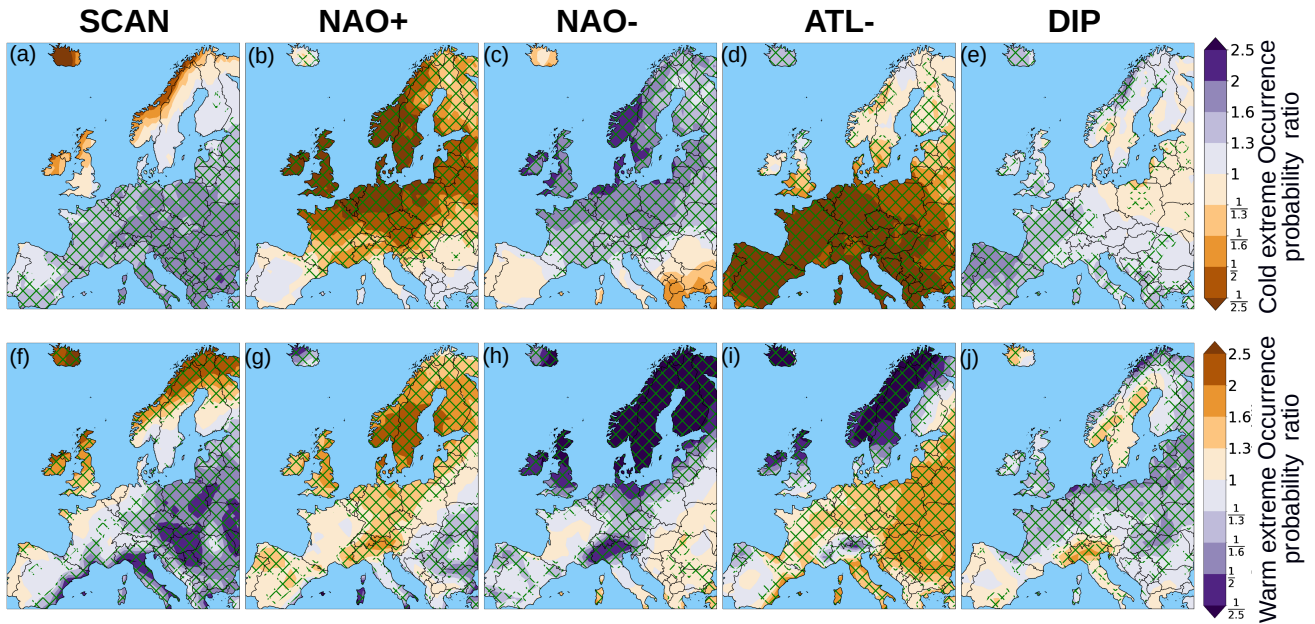
Figure 3. Temperature extreme occurrence probability ratios averaged over the extended winter season for different circulation regimes plotted over the European domain using the ECHAM6 PAMIP pdSIC/pdSST simulation. Upper row a-e: cold days, bottom row f-j: warm days. The plotted ratio compares the occurrence probability of an extreme day given a certain circulation regime to the unconditioned probability of an extreme occurrence. Thus, for instance violet values greater than one in a–e indicate a preferred cold extreme occurrence at a specific grid point during the presence of a certain regime compared to the overall extreme occurrence. Note, that the color bar is reversed for warm extremes in f–j. Hatched areas indicate ratios that are significantly different from unity based on a moving bootstrap.
