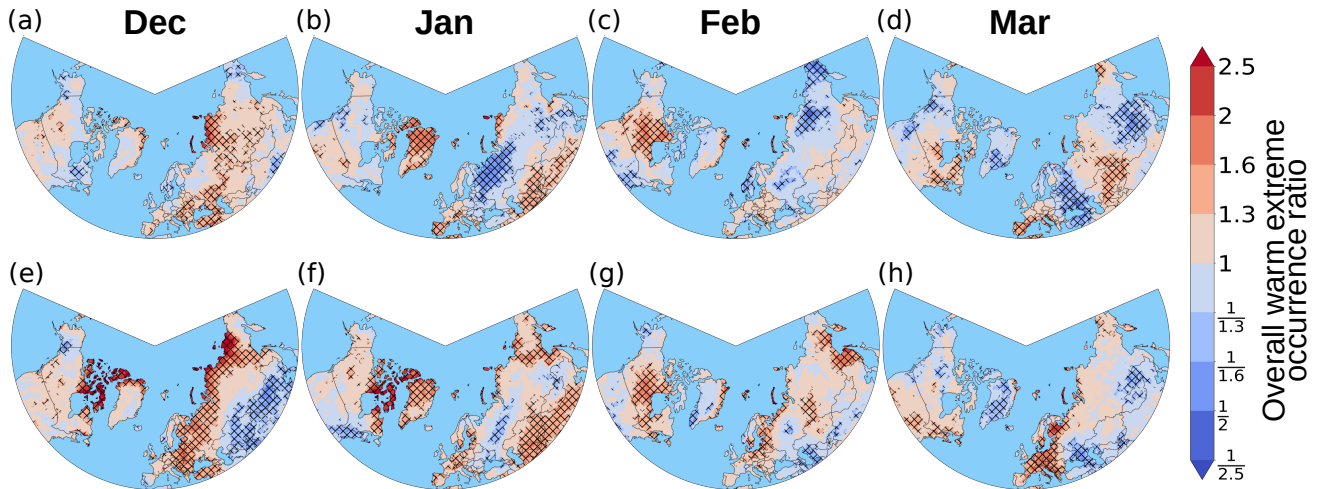
Figure 5. Same as in Fig. 4 but for warm extremes. Note that the colorbar is reversed compared to Fig. 4, such that red indicates more frequent warm extreme occurrences, and blue indicates less frequent warm extreme occurrences in the sensitivity experiments.
