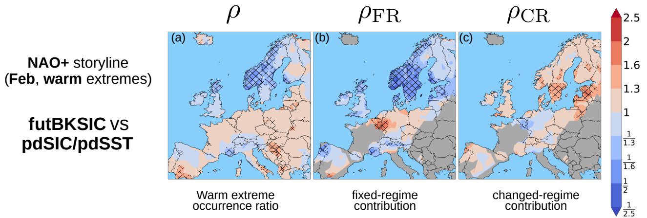
Figure 8. Same as in Fig. 6 (futBKSIC vs. pdSIC/pdSST simulation) but for February warm extremes and assuming a NAO+ regime storyline. Here, red indicates more frequent warm extreme occurrences, and blue indicates less frequent warm extreme occurrences in futBKSIC. Occurrence ratio of NAO+ regime occurrence in February is given as \rho_{\text{circ}} = 0.8 . Thus, the NAO+ regime occurs less frequent in the futBKSIC simulation (see also Fig. S2g). \rho_{\text{FR}} and \rho_{\text{CR}} are only plotted for regions where statistically significant preferred winter warm extreme occurrences during NAO+ days were identified in Fig. 3g.
