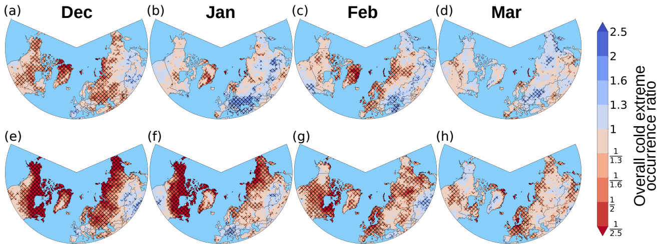
Figure 4. Cold extreme occurrence ratio for December, January, February and March in ECHAM6. The occurrence probability of northern hemispheric continental cold extremes are compared between the sensitivity experiments vs. the pdSIC/pdSST reference simulation. Upper row (a)–(d): futBKSIC sensitivity run. Bottom row (e)–(h): futArcSIC sensitivity run. Blue indicates more frequent cold extreme occurrences, and red indicates less frequent cold extreme occurrences in the sensitivity experiments. Hatching indicates regions where the ratio differs significantly from unity based on a moving block bootstrap.
