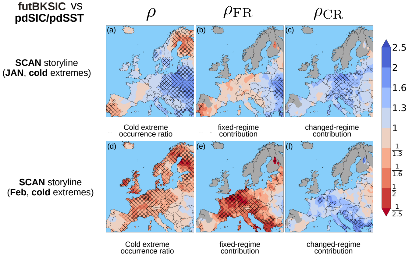
Figure 6. Conditional extreme event attribution framework for European cold extremes assuming a SCAN-storyline. Compared are the the futBKSIC sensitivity and the pdSIC/pdSST reference simulations. Blue indicates more frequent cold extreme occurrences, and red indicates less frequent cold extreme occurrences in futBKSIC. Upper row: January with \rho_{circ} = 1.26 . Bottom row: February with \rho_{circ} = 1.23 . \rho_{circ} greater than unity means that the SCAN regime occurs more frequent in the futBKSIC simulation for both months (see also Fig. S2f). The first column shows the overall cold extreme occurrence ratio \rho = \rho_{FR} \cdot \rho_{CR} between both simulations, the second column shows the fixed-regime contribution \rho_{FR} , the third one shows the changed-regime contribution \rho_{CR} . Hatching indicates regions where the ratios significantly differ from unity based on a moving block bootstrap. \rho_{FR} and \rho_{CR} are only plotted for regions where statistically significant preferred winter cold extreme occurrences during SCAN days were identified in Fig. 3a.
