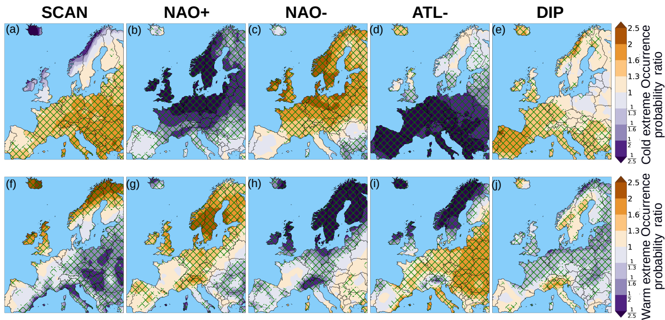
Figure 3. Temperature extreme occurrence probability ratios (DJFM) for different circulation regimes plotted over the European domain using the ECHAM6 PAMIP pdSST/pdSIC simulation. Upper row a-e: cold days, bottom row f-j: warm days. The plotted ratio compares the occurrence probability of an extreme day given a certain circulation regime to the unconditioned probability of an extreme occurrence. Thus, values greater than one at a specific grid point indicate preferred extreme occurrence during the presence of a certain regime compared to the overall extreme occurrence. Dotted areas indicate ratios that are significantly different from unity based on a moving bootstrap.
