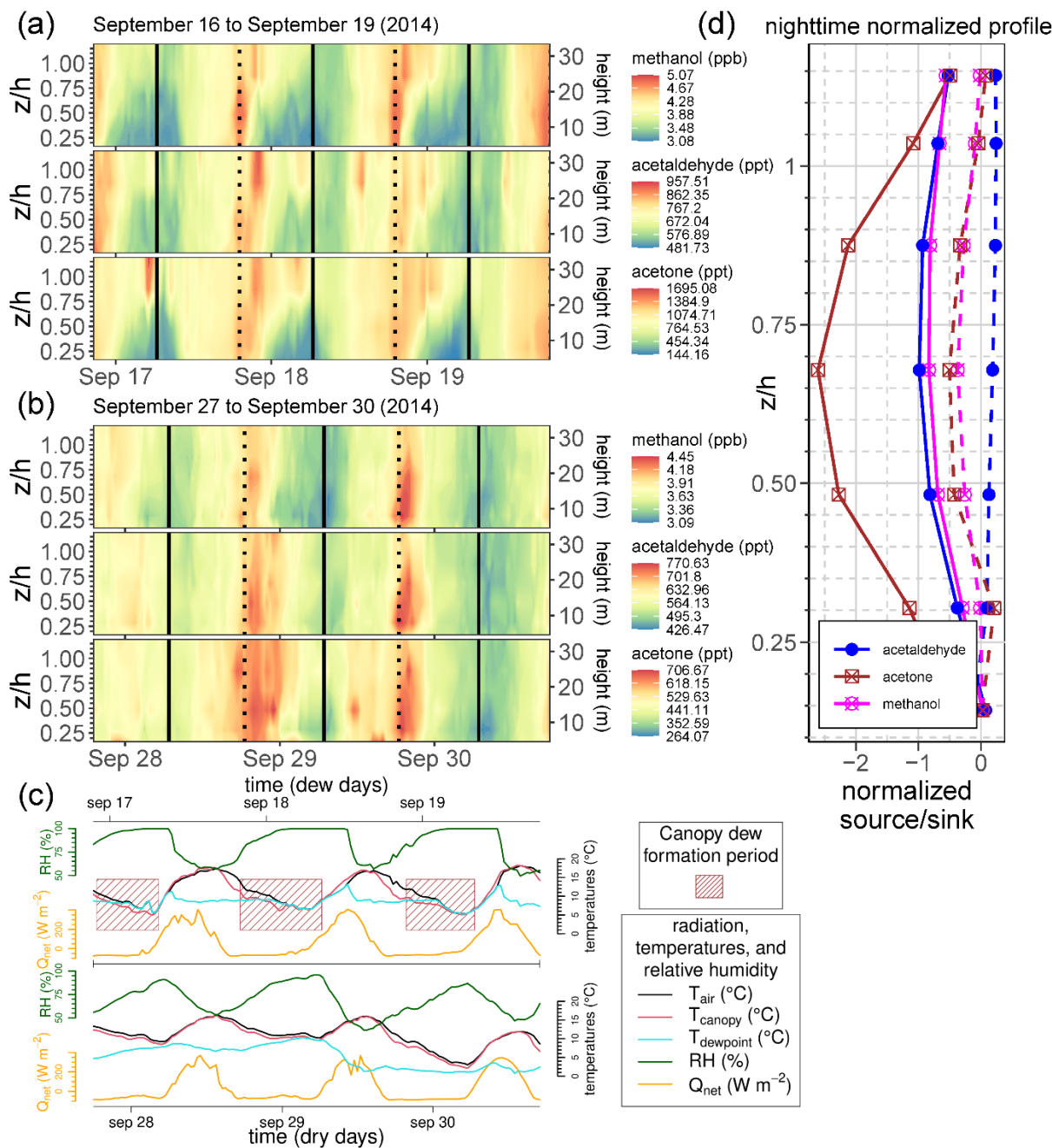
445 Figure 11: Nighttime dew effects on water-soluble BVOCs in forest canopy. (a) Methanol concentration profile from Sept. 16 th to 19 th , during conditions where nighttime dew is assumed to have formed in the forest canopy. (b) Methanol concentration profile two weeks later, from Sept. 27 th to 30 th , during dry conditions. In a) and b), sunrise (solid vertical line) and sunset (dotted vertical line) are indicated. (c) 3-day time-series for meteorological conditions during the “dry” period from Sept. 27 th to 30 th (bottom-of-panel) and during the “dew” periods from Sept. 16 th to 19 th (top-of-panel). The meteorological values shown are air temperature (black) in the canopy (at 28 m), IR-measured canopy surface temperature (red), dewpoint temperature (cyan) in the canopy (at 28 m), relative humidity (green), and net radiation (orange). Relative humidity is measured at 28 m. Time periods when dew is expected to have formed in the forest canopy during the “dew” periods are indicated in panel (c) with brown boxes. (d) 450
