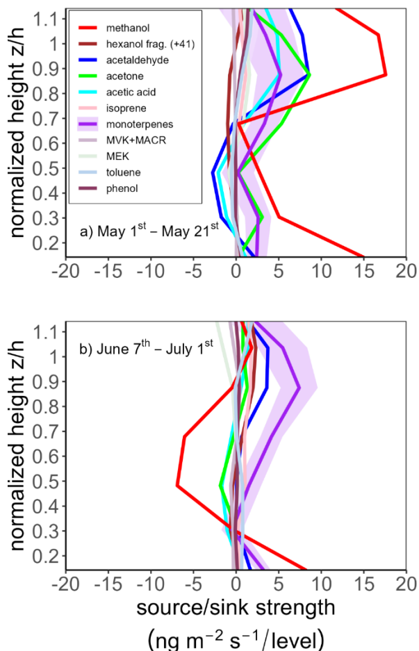
435 Figure 10: 2016 BVOC inversion results for the canopy source and sink profile distribution. Data shown represent the average of daytime concentrations (from 1.5 h after sunrise to 1.5 h before sunset) for (top panel) May 1 st to May 21 st and (bottom panel) June 7 th to July 1 st , 2016. Shaded region for monoterpenes indicates \pm standard error. The flux tower air temperature and PAR during these time periods are shown in the top panel of Figure 8.
