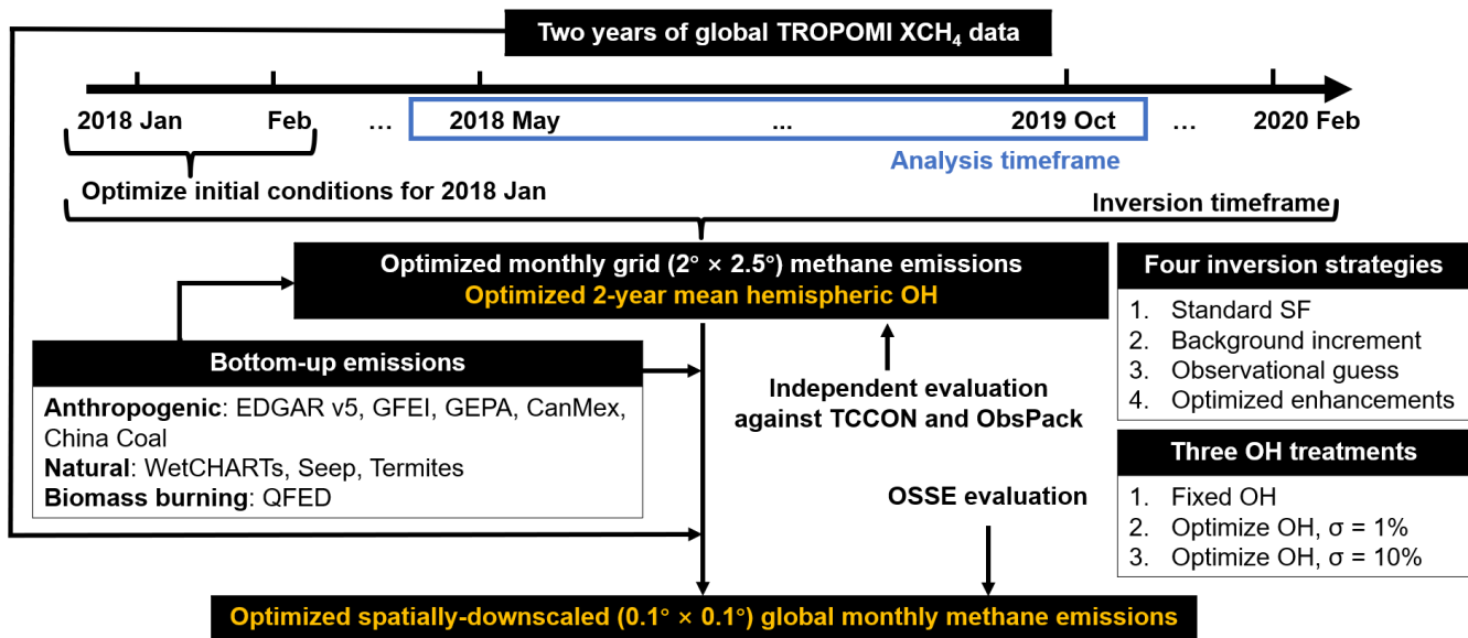
Figure 1. Flow chart showing the TROPOMI methane inversion methodology.
