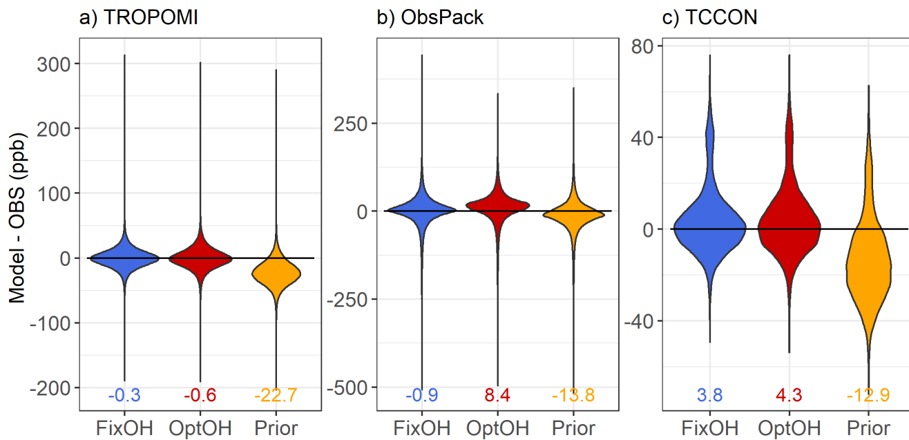
1070 Figure 3. Evaluation of the prior and optimized methane simulations (05/2018–10/2019) against a) TROPOMI XCH 4 observations, b) ObsPack in-situ methane measurements, and c) TCCON ground-based methane column observations. Numbers inset indicate the mean model-observation bias (unit: ppb).
