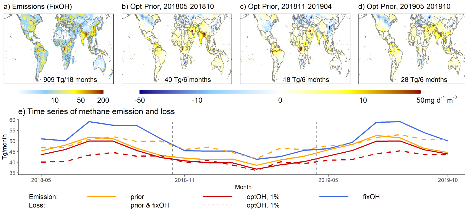
1075 Figure 4. a) Optimized global methane emissions based on the fixOH inversion ensemble. b)–d) Seasonal fixOH emission corrections. Dots indicate missing sources where the EE and BI inversions point to positive corrections that the SF inversion misses. e) Time series of prior and optimized methane sources and sinks.
