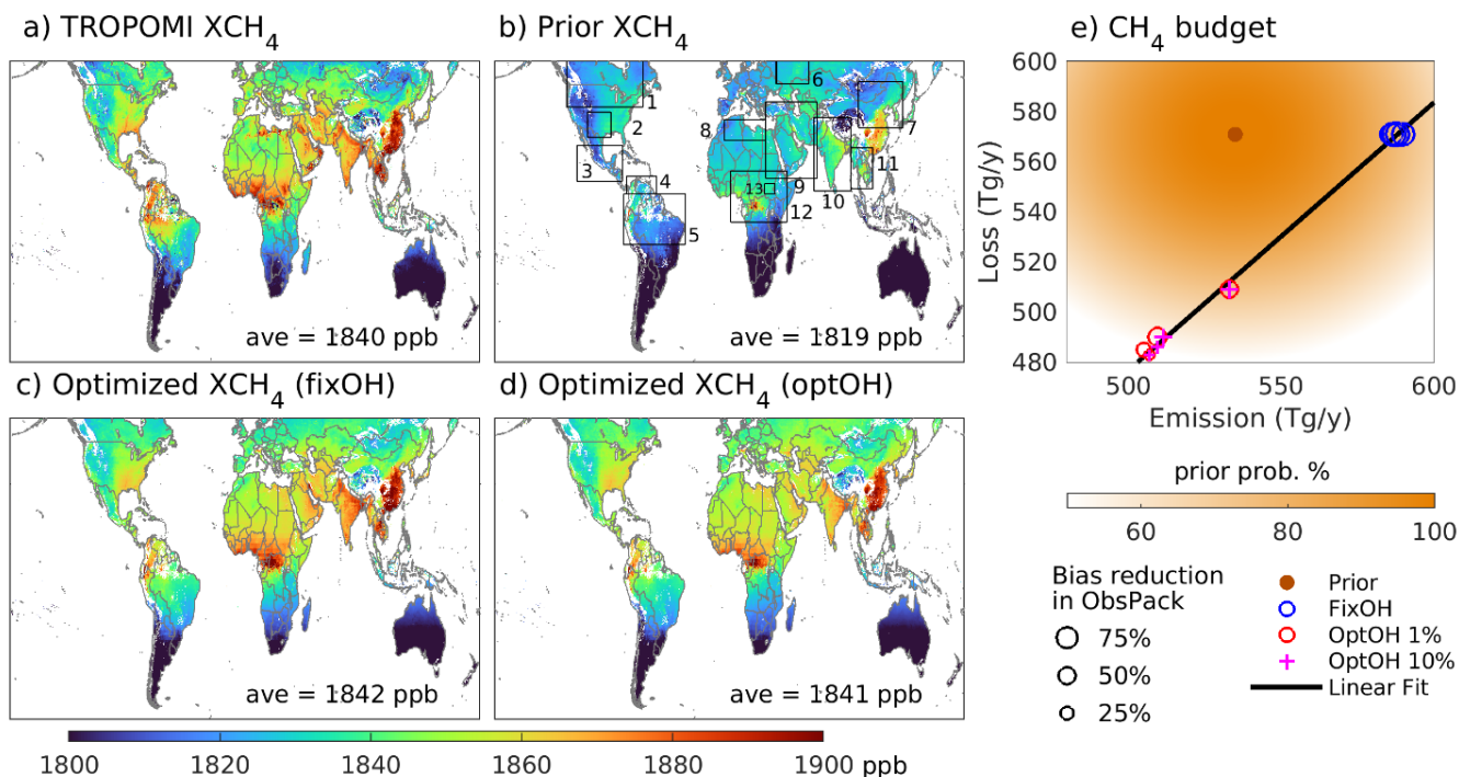
1060 Figure 2. Observed and simulated methane distributions for 03/2018–02/2020. a) TROPOMI methane column (XCH 4 ) observations oversampled to 0.1^\circ \times 0.1^\circ . b) Methane column distribution predicted by the prior model sampled according to the TROPOMI observation operator with numbered regions described in-text. c) Same as panel b but for the fixOH optimized ensemble mean. d) Same as panel b but for the optOH optimized ensemble mean. e) Prior and optimized methane budgets. Prior probabilities (orange) equate one standard deviation to 25% of the bottom-up range from Saunio et al. (2020), following Hoze et 1065 al. (2005). Black line shows a linear fit to the solution, \text{emission} = 0.93 \times \text{loss} + 55.26 (units: Tg/y). Symbol sizes indicate the mean bias reduction against ObsPack independent measurements. Annual values are for 11/2018–04/2019 plus the average of 05– 10/2018 and 05–10/2019.
