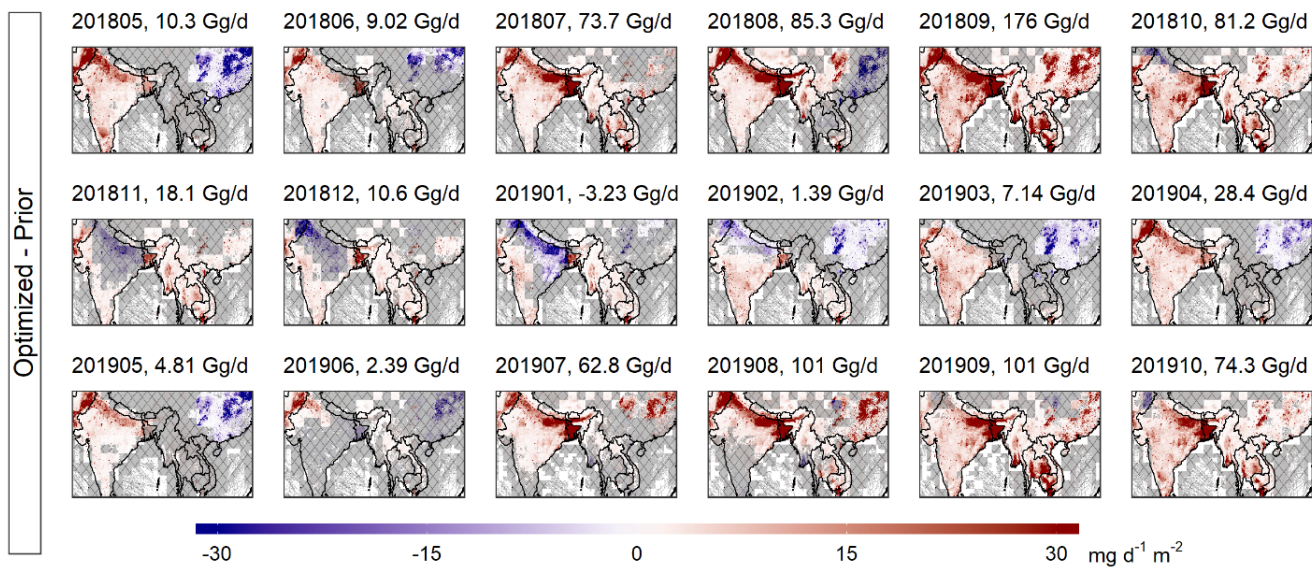
1085 Figure 6. TROPOMI-derived emission corrections over South and East Asia based on the fixOH ensemble mean. Shading indicates areas where corrections are not distinguishable from zero (i.e., inversion ensemble includes both positive and negative adjustments).
