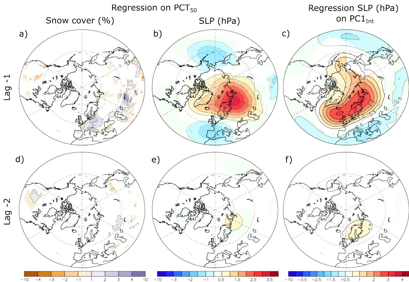
165 Figure 16: Regression of the (a,d) snow cover, in % , and sea level pressure (SLP; b,e) anomalies, in hPa , onto the January polar cap (north of 60°N) 50-hPa temperature anomalies in LMDZOR6. (c,f) Regression of the sea level pressure (SLP) anomalies, in hPa , onto the First PC of the snow cover internal atmospheric variability, PC1_{Int} , in January and LMDZOR6. The lag indicated is negative and given in month, indicating that the polar cap 50-hPa geopotential height or the PC1_{Int} lags. The color shades are masked if the local statistical significance is above 5%.
