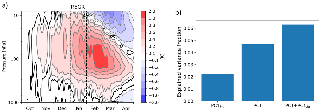
Figure 15: (a) Regression of the daily air temperature anomalies over the polar cap (north of 60^{\circ}N ), in ^{\circ}C , onto the First PC of the snow cover internal atmospheric variability, PC1_{Int} , in January and in LMDZOR6. The black line indicates the local statistical significance at the 5% level. The vertical dashed black line shows the days corresponding to January. (b) Explained variance fraction of the Arctic Oscillation defined as the first EOF of the sea level pressure north of 20^{\circ}N , for a regression using PC1_{Int} , PCT_{50} and both PCT_{Int} and PCT_{50} as predictors. The explained variance fraction is significant at the 5% level in the three cases.
