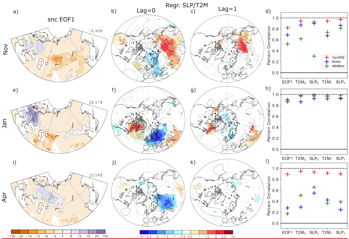
105 Figure 10: (First column from left) First EOF of the detrended Eurasian snow cover in ERA5-Land, shown as the regression of the the snow cover, in %, onto the first PC. (Second column) Regression of the observed (color shade and grey contours) surface air 110 temperature, in °C, and (black contour; contour interval 1 hPa) sea level pressure in hPa on PC1 at lag=0, and (third column) at lag = 1, i.e. for PC1 leading by one month the atmospheric fields. (Fourth column) Pattern correlation of the EOF1s and of the regressions of surface air temperature or sea level pressure on the Eurasian snow cover PC1 between ERA-Land and other snow cover datasets. T2M 0 and SLP 0 designate the pattern correlation of the regressions at lag = 0; T2M 1 and SLP 1 designate the pattern correlation at lag = 1. The first row is for November, the second row for January and the third row for April. In the second and third columns, color shadings indicate p-value below 5% for the surface air temperature regression.
