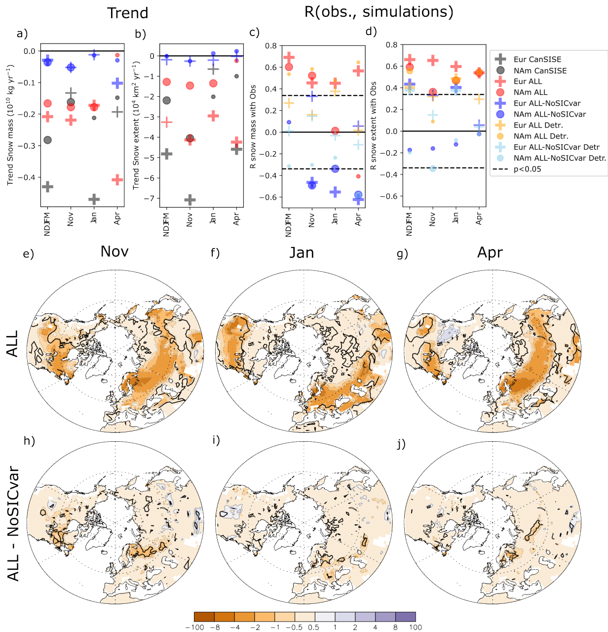
Figure 5: Trend in Northern Hemisphere (trend in a) snow mass over extent and (b) snow extent mass. Correlation between with ERA5-Land and simulated values for (c) snow mass over extent and (d) snow extent mass. Red (blue) symbol denotes the simulation ALL (-ALL minus NoSICvar/NoSIC) for 1979-2014. Grey symbol denotes the CanSISE observations for 1979-2010. Orange (blue sky) symbol is for the simulation ALL (ALL minus NoSICvar/NoSIC) when using linearly detrended fields. Northern Hemisphere trend in snow cover, in % per decade 1 , for the multi-model mean of simulations (e-g) ALL and (h-j) the difference of (h-j) ALL minus NoSICvar/NoSIC; in (e) (h) November (f) (i) January and (g) (j) April. In (a-d), the size of the symbol is large (small) if the significance of the trends is below (above) 5%. In (e-j), black contours indicate where the p-values are lower than 5%.
