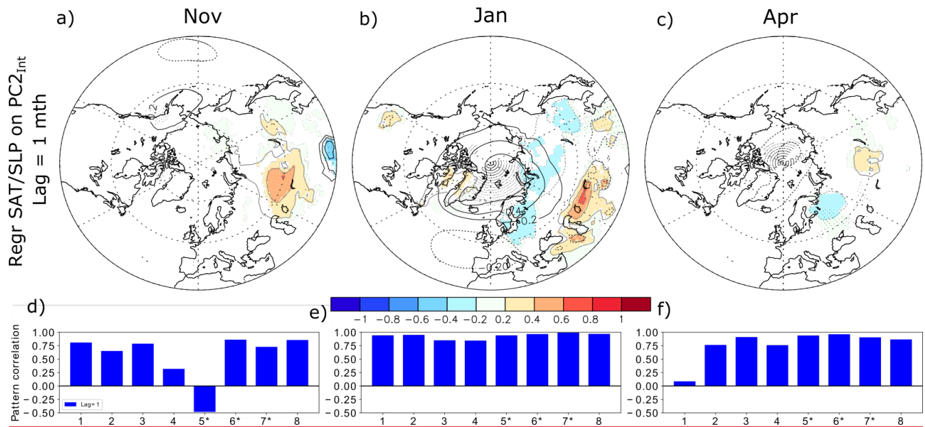
Figure 14: Same as Fig. 12a-c12, but using PC2_{Int} instead of PC1_{Int} at lag = 1 month, when the atmosphere follows by one month the (a) (d) November, (b) (e) January and (c) (f) April snow cover. The last row shows the spatial pattern correlation north of 20^{\circ}N between the SLP regression obtained from each model and that of the model average. The blue bar shows the results at lag 1. The numbers on the x-axis designate each model (see Table 1 for the corresponding model names). The symbol star indicates when 30 members are available for both ALL and NoSICvar; for (g) November, (h) January and (i) April.
