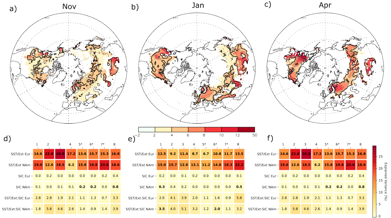
65 Figure 6: Variance fraction (in %) of the interannual snow coverwater equivalent anomalies explained by SST, external forcing and sea ice concentration; for (a) November, (b) January and (c) April. The thick black curve indicates where the p-value of the ANOVA test is lower than 5% for at least 5 models out of 8. Variance fraction (in %) of the snow cover area over Eurasia (Eur) and North America (NAM) calculated for each model separatelyseparaty for (d) November, (e) January and (f) April. The number from 1 to 8 designates the model (see table 1 for correspondence with model name). The symbol star indicates when 30 members are available for both ALL and NoSICvar. The effect of the factor t , representing the influence of SST and external forcings, is referredreferred to as SST/ext. The effect of the factor e , representing the influence of SIC on the time mean snow, is referredreferred to as SIC. The effect of the factor t:e , representing the influence of SIC on the time-varying snow, is referredreferred to as SST/Ext:SIC. Numbers are given in bold font if the ANOVA test has a p-value below 5%. 70
