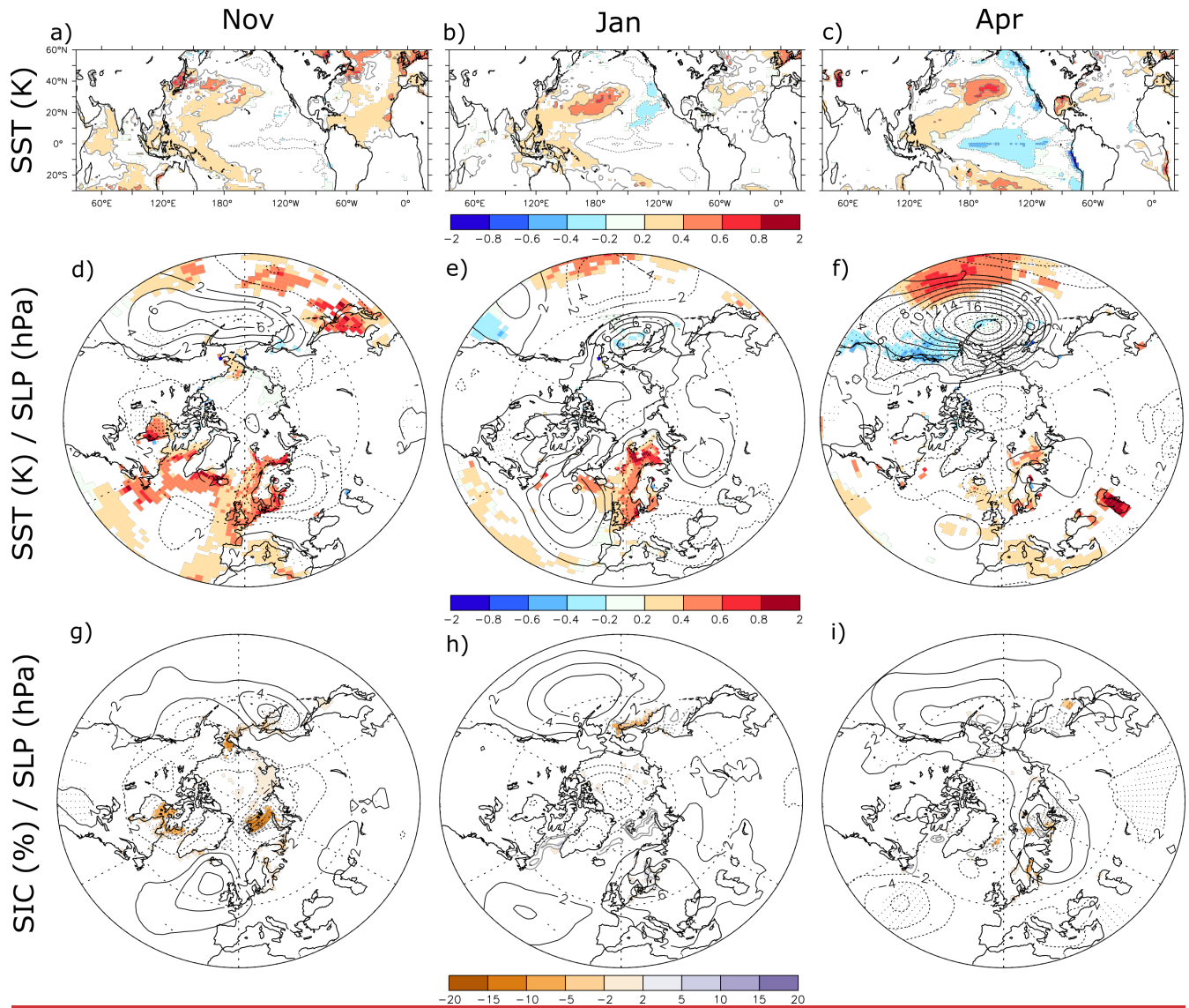
Figure 9: (a) (b) (c) Regression of the SST, in ^{\circ}\text{C} (gray contours and color shade) on \text{PC1}_{\text{BC}} ; (d) (e) (f) Regression of the SST, in ^{\circ}\text{C} (color shade) and sea level pressure, in hPa (black contour, contour interval 2 hPa; dotted contours for negative values), on \text{PC1}_{\text{BC}} . (g) (h) (i) Regression of the SIC, in % (gray contours and color shade), and sea level pressure, in hPa (black contour, contour interval 2 hPa; dotted contours for negative values), on \text{PC1}_{\text{SIC}} . In all panels, color shade indicates p-value below 5% for the regression of the SST or SIC. Dots indicate indicates p-values below 5% for the SLP regression in panels (d)-(i). Left panels are for November. Center panels are for January. Right panels are for April.
