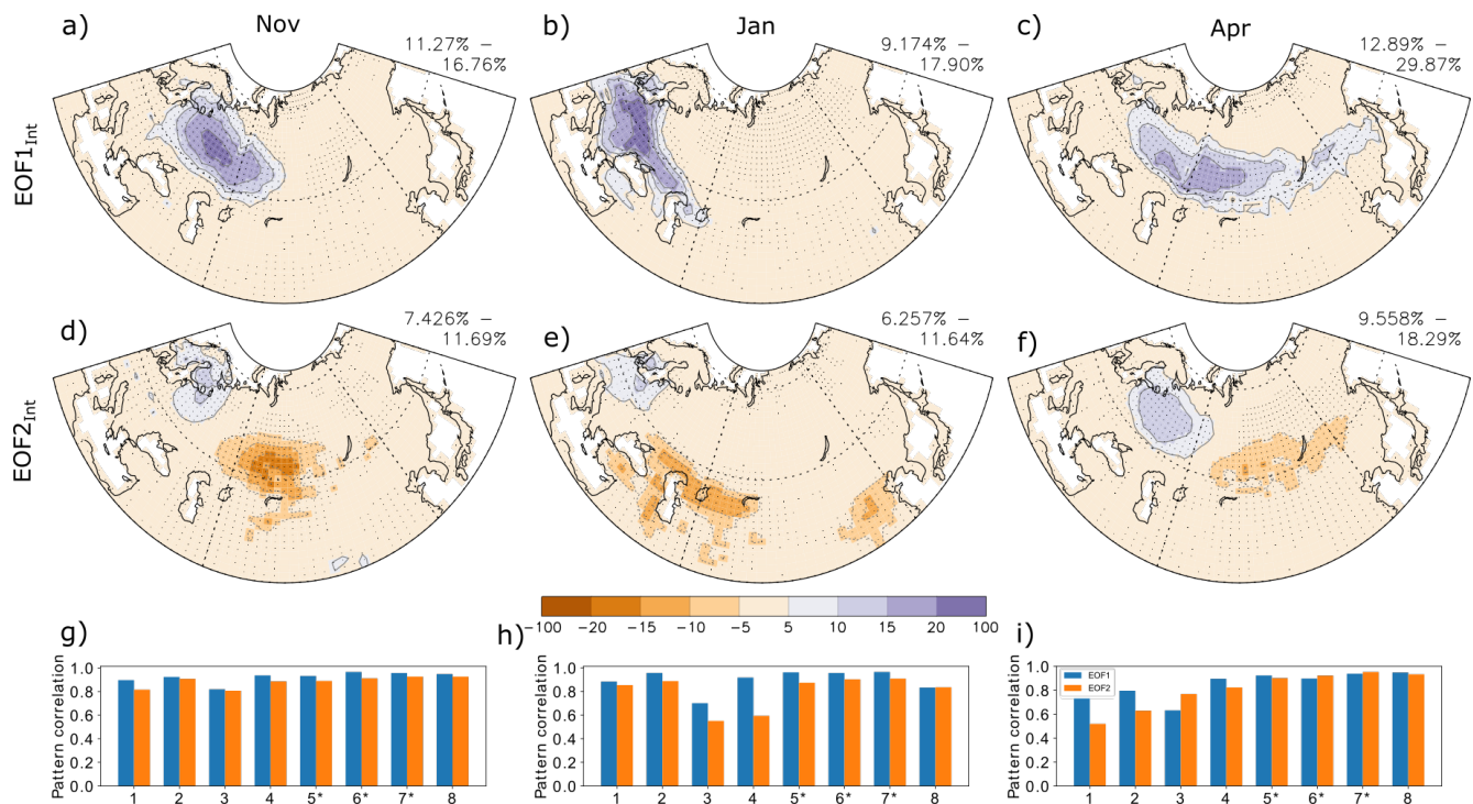
Figure 11: (First row) First and (second row) second EOF int of the Eurasian snow cover, in %, associated with internal atmospheric variability in the simulations ALL and NoSICvar NoSIC . The patterns are the average patterns of the eight models. The numbers displayed on top are the minimum and maximum variance explained by that EOF among the eight models. Dots indicate the locations where 7 models out of 8 have EOF int anomalies with the same sign. (Last row) Spatial pattern correlation between the EOF int obtained from each model and that of the model average. The blue (orange) bar shows the results when using the first (second) EOF. The numbers on the x-axis designates designates each model (see Table 1 for the corresponding model names). The symbol star indicates when 30 members are available for both ALL and NoSICvar NoSIC ; for (left column) November, (center column) January and (right column) April.
