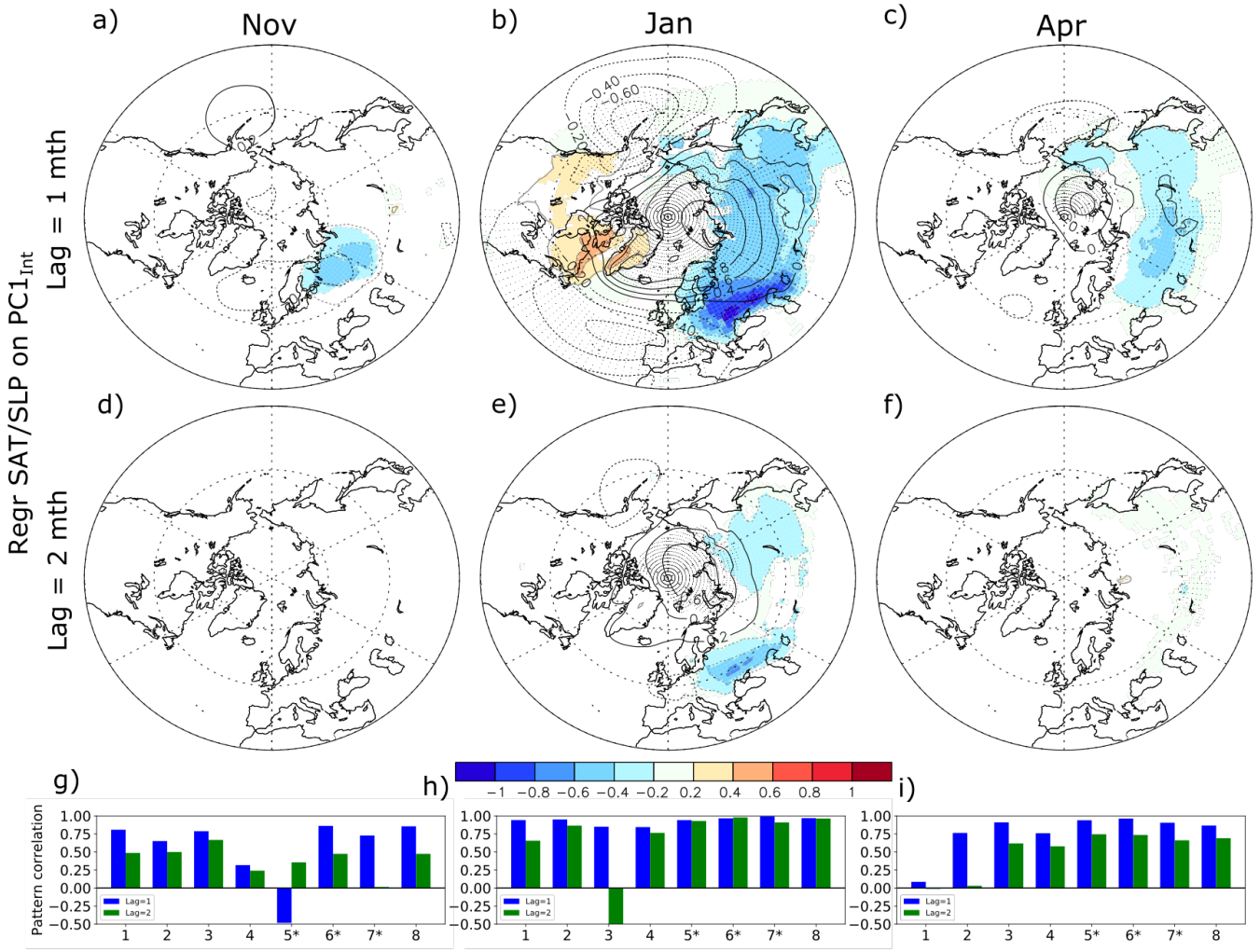
Figure 13: Same as Fig. 12a-c+2, but at (a) (b) (c) lag 1 and (d) (e) (f) lag 2, when the atmosphere follows by one month the (left) November, (center) January and (right) April snow cover index, as provided by PC1 int . The last row shows the spatial pattern correlation north of 20°N between the SLP regression obtained from each model and that of the model average. The blue (green) bar shows the results at lag 1 (2). The numbers on the x-axis designate each model (see Table 1 for the corresponding model names). The symbol star indicates when 30 members are available for both ALL and NoSICvar; for (g) November, (h) January and (i) April.
