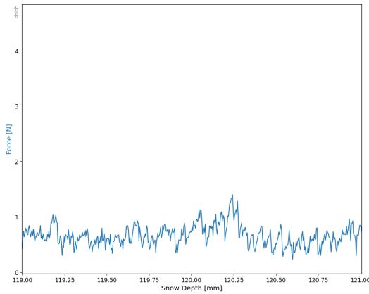
(g) A snow micro penetrometer signal showing a typical tooth-like signal for depth hoar (DH).
