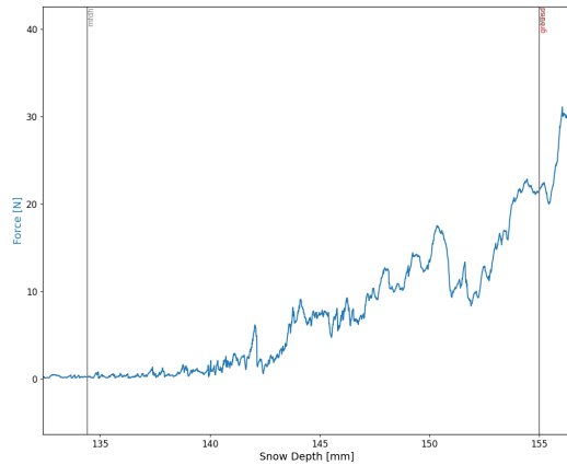
(c) A snow micro penetrometer signal showing a typical increase in force at the snow-sea ice interface. This signal is typical for a remnant surface scattering layer, named melt form, depth hoar (MFdh) in this study. This signal typically has a force range of 5 – 30 N.
