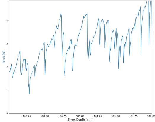
(e) A snow micro penetrometer signal showing a typical tooth-like signal for indurated depth hoar (DHid) with a force between 2 – 6 N.
