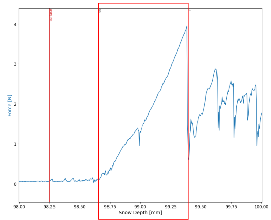
(b) A snow micro penetrometer signal showing a typical signal for ice formations (IF) with a sharp singular peak at a maximum of 4 N between approximately 98.6 mm and 99.3 mm.
