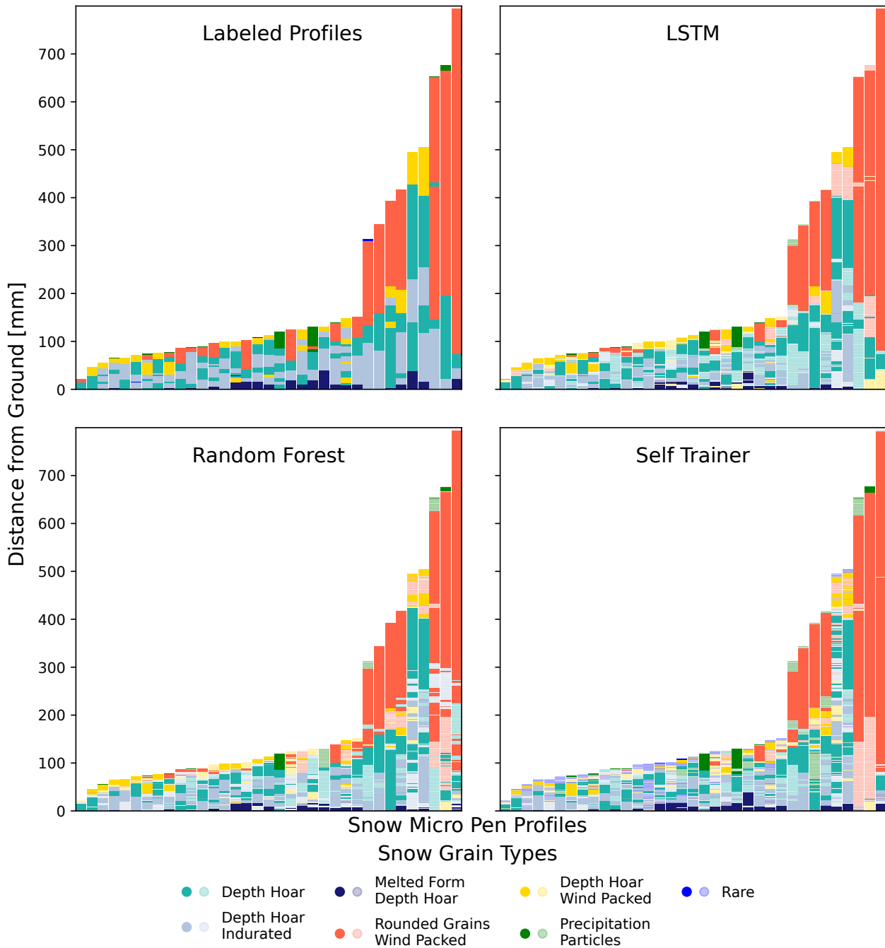
Figure 2. Predictions on the test dataset of the LSTM, random forest, and self-trainer. The upper left panel shows the labeled data. In the other panels, the correct predictions are shown with more intense colours and the wrong predictions with less intense colours. The LSTM has the highest rate of correct predictions and imitates the smoothness of the labeled data very well. The random forest does well but provides more segmented predictions. The self-trainer immensely overestimates rare classes.
