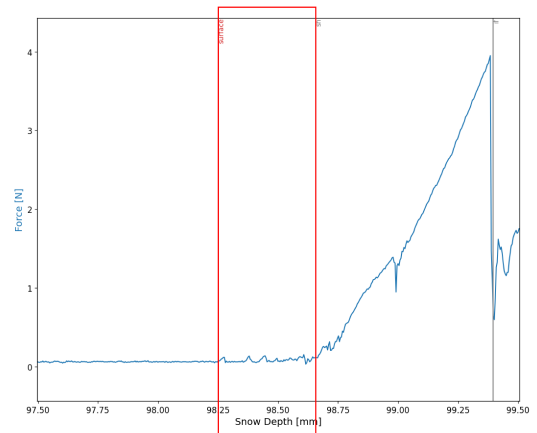
(d) A snow micro penetrometer signal showing a typical signal for surface hoar (SH) at the surface of the profile with a tooth-like structure with a low force signal.
