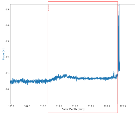
(a) A snow micro penetrometer signal showing a typical signal for decomposing and fragmented precipitation particles (DF) with a force remaining under 0.1 N between approximately 111 mm and 121 mm.
