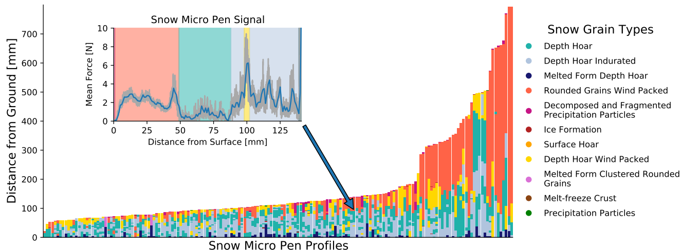
Figure 1. All 164 labeled SnowMicroPen (SMP) profiles used for training, validation (80%), and testing (20%). Each bar represents one SMP profile. The colours encode the different snow types. The top of each bar is the air-snow interface and the bottom is the profile’s snow-ground interface. The in-picture figure illustrates the force signal (grey) and the mean force signal (blue) of a single SMP profile (S31H0368). The snow-air interface is on the left, and the bottom of the profile is on the right. The background shading in the inset panel and the colors in the main panel represent the labeling of the profiles.
