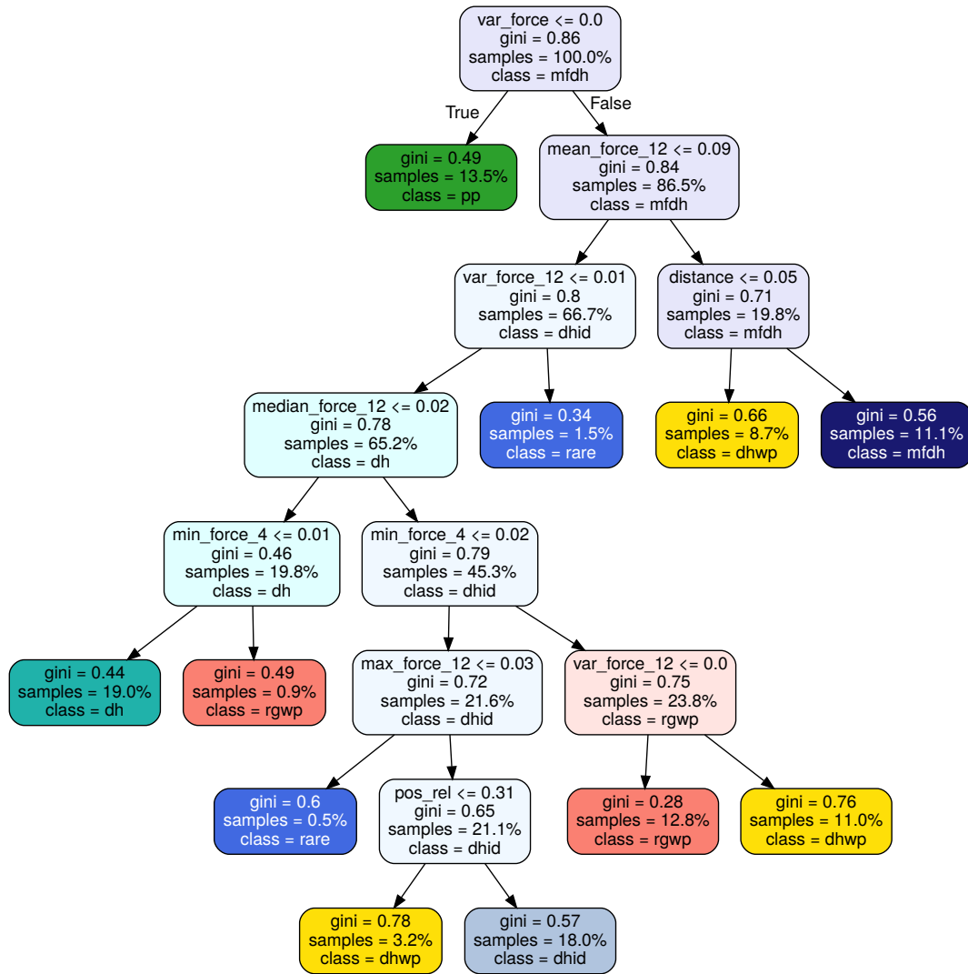
Figure G1. Pruned decision tree extracted from the random forest. See Appendix C1 to understand the features that the nodes represent. Decision trees encode the decision rules for predicting snow type labels. This approach helps to explain the model’s decisions, a property that is often asked for by domain experts. At each leaf node, a labeling decision is made. All the other nodes encode the labeling rules that are used to classify each point. Take the root node as an example: If the variance of the force is smaller or equal to zero, the point is labeled as “Precipitation Particles”. Else it has to be one of the other labels. The Gini index encodes how well separable the subsets of data points are (the bigger the number the better), and the sample’s number shows how much percent of the complete data can be found in this subset.
