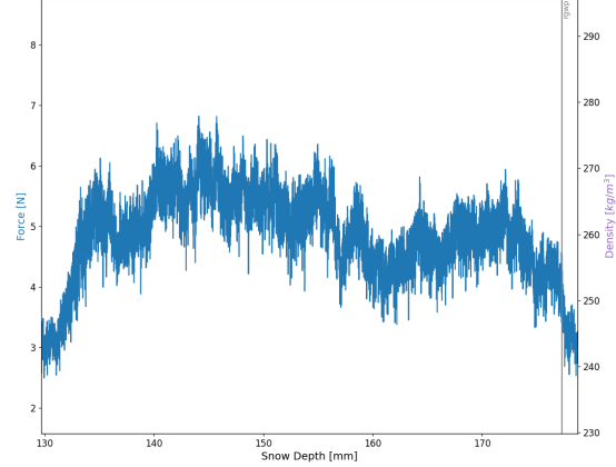
(f) A snow micro penetrometer signal showing a typical wavy force signal for rounded grains, wind packed snow (RGwp).
