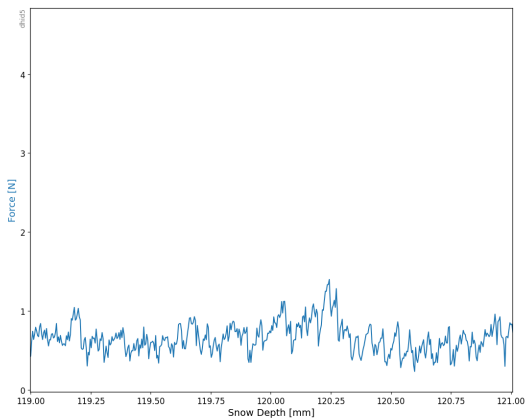
(g) A snow micro penetrometer signal showing a typical tooth-like signal for depth hoar (DH).
