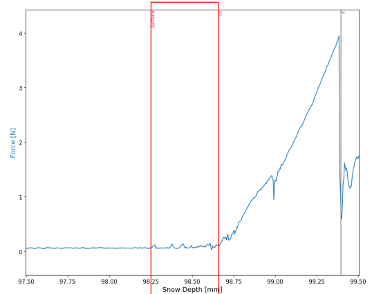
(d) A snow micro penetrometer signal showing a typical signal for surface hoar (SH) at the surface of the profile with a tooth-like structure with a low force signal.
