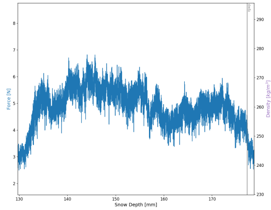
(f) A snow micro penetrometer signal showing a typical wavy force signal for rounded grains, wind packed snow (RGwp).
