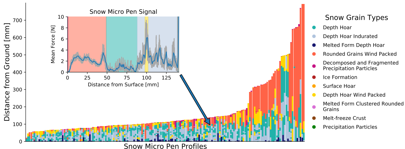
Figure 1. All 164 labelled SnowMicroPen (SMP) profiles used for training, validation (80%), and testing (20%). Each bar represents one SMP profile. The colours encode the different snow grain types. The top of each bar is the air-snow interface and the bottom is the profile’s snow-ground interface. The in-picture figure illustrates the force signal (grey) and the mean force signal (blue) of a single SMP profile (S31H0368). The snow-air interface is on the left, and the bottom of the profile is on the right. The background shading represents the ground-truth labelling of the profile.
