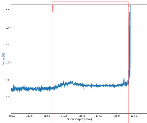
(a) A snow micro penetrometer signal showing a typical signal for decomposing and fragmented precipitation particles (DF) with a force remaining under 0.1 N between approximately 111 mm and 121 mm.
