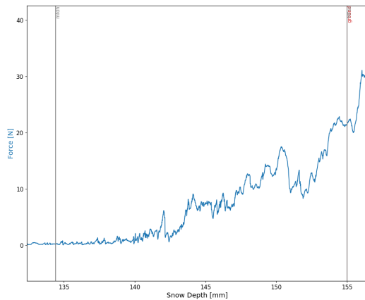
(c) A snow micro penetrometer signal showing a typical increase in force at the snow-sea ice interface. This signal is typical for a remnant surface scattering layer, named melt form, depth hoar (SHMFdh) at the surface of the profile with a tooth-like structure with in this study. This signal typically has a low-force signal range of 5 – 30 N.
