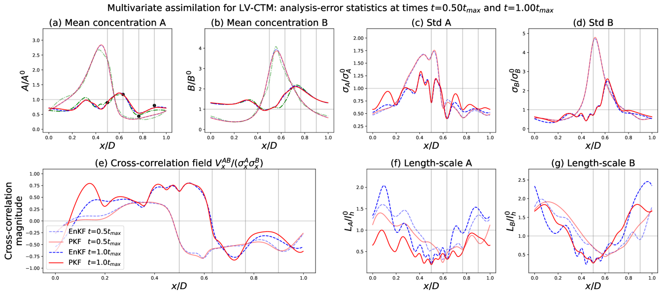
Figure 13. Results of the data assimilation numerical experiment. Nature run ( solid dash dotted green lines, only on panels (a) and (b) ), PKF errors statistics (solid red lines) and EnKF diagnosed error statistics (dashed blue lines) at times t = [0.50, 1.00]t_{max} . These times correspond approximately to t=23\text{h}45\text{min} and t=47\text{h}40\text{min} . At time t = 0.5t_{max} , two analysis steps have already been performed. At time t = 1.00t_{max} , the fifth analysis step is being realized, the generated observations are represented by black dots on panel (a). The vertical grey lines correspond to the sensors locations.
