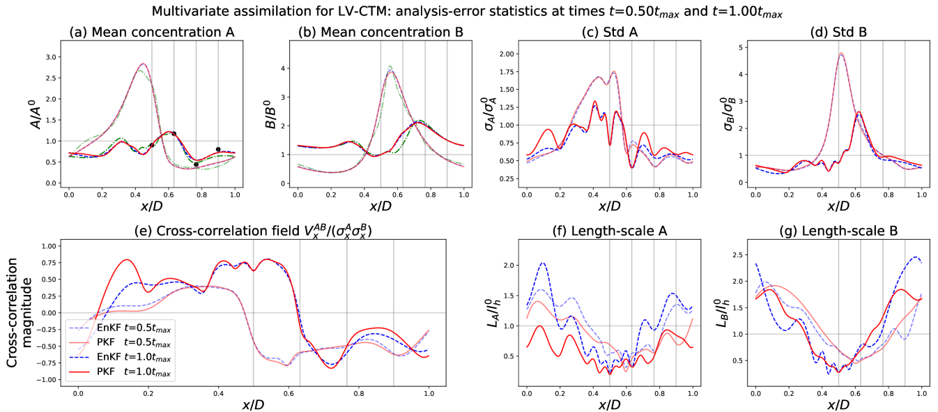
Figure 13. Results of the data assimilation assimilation numerical experiment. Nature run ( solid dash dotted green lines, only on panels (a) and (b) ), PKF errors statistics (solid red lines) and EnKF diagnosed error statistics (dashed blue lines) at times t = [0.50, 1.00]t_{max} . These times correspond approximately to t=23\text{h}45\text{min} and t=47\text{h}40\text{min} . At time t = 0.5t_{max} , two analysis steps have already been performed. At time t = 1.00t_{max} , the fifth analysis step is being realized, the generated observations are represented by black dots on panel (a). The vertical grey lines correspond to the sensors locations.
