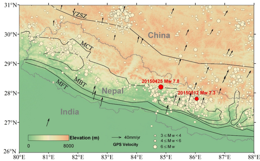
Figure 1: The distribution of earthquakes with magnitude greater than 3.0 in and nearby Nepal from 1912 to 2022 (from USGS). GPS velocity field refers to Su et al. (2015). Black arrows indicate the average velocities and directions of ground movement in 1990-2015 110 from GNSS observations (Kreemer et al., 2014; Zheng et al., 2017).
