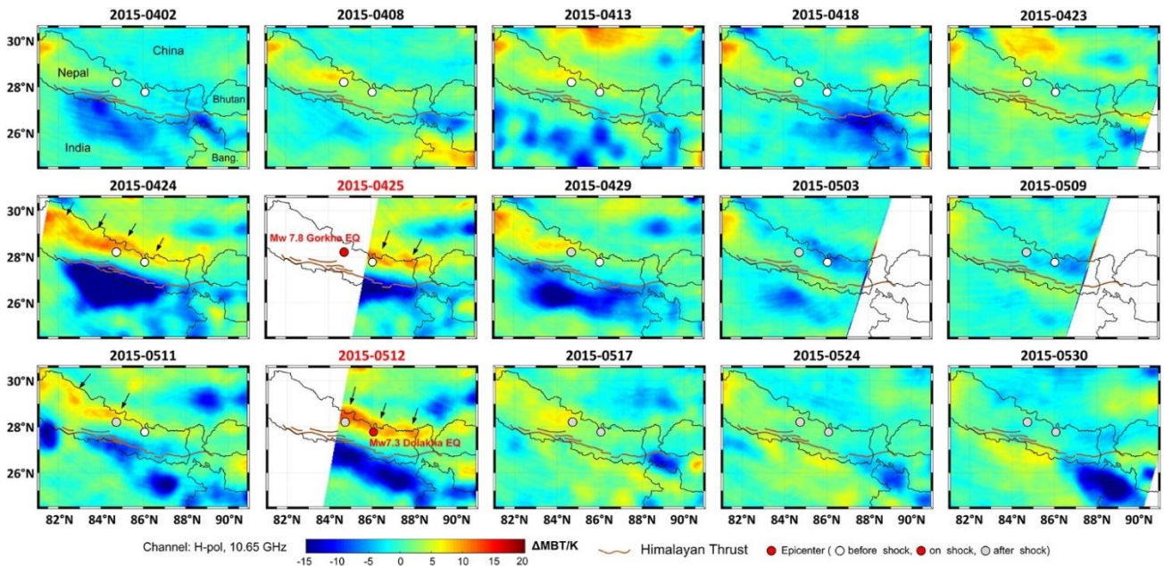
Figure 1: The spatio-temporal evolution of MBT anomalies before, during and after the 2015 Nepal earthquake sequence.
