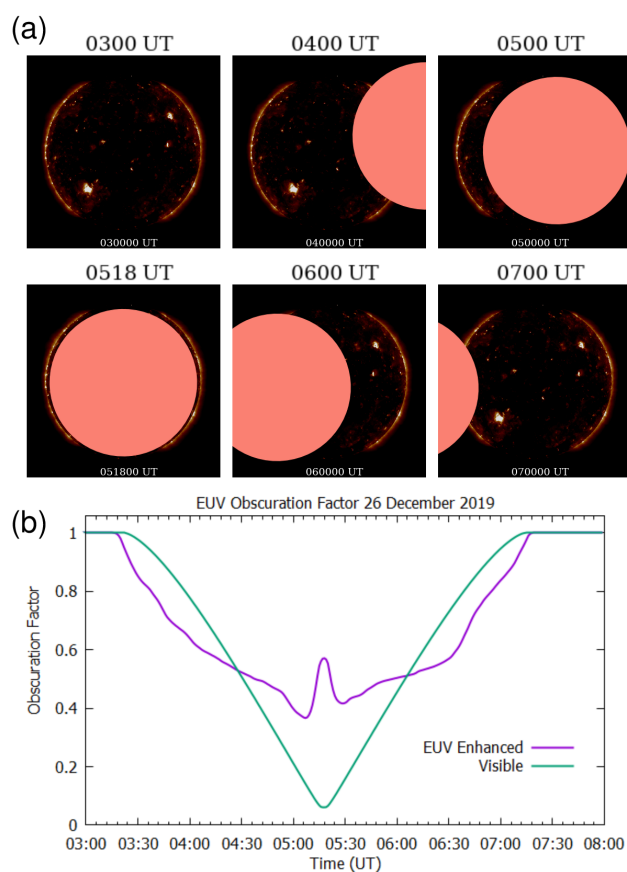
Figure 4. (a) Sample sequence of digitally masked 193 Å (19.3 nm) solar AIA images on 26 December 2019 to estimate the level of solar obscuration at a given point on the Earth's surface during the course of the solar eclipse. (b) Time series variation of the obscuration of solar irradiance at various wavelengths during the 26 December 2019 annular solar eclipse over Siak, Riau Province (1.01°N 102.25°E), calculated using this computational masking method.
