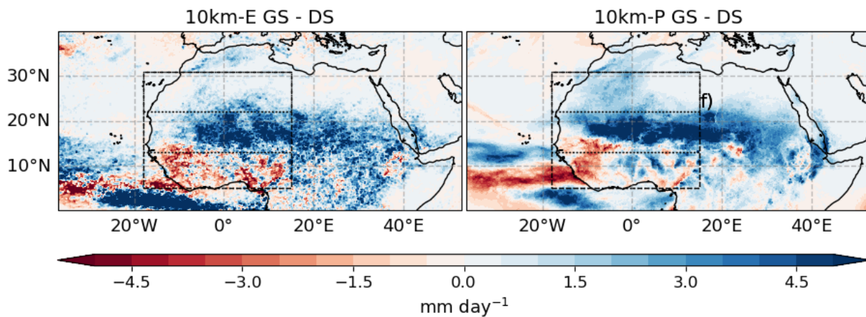
Figure B5. JAS-mean difference in precipitation rate between the GS and DS simulation for the 10km-E (a) and the 10km-P (b) experiment, respectively. The dashed box indicates the WA-analysis domain.
