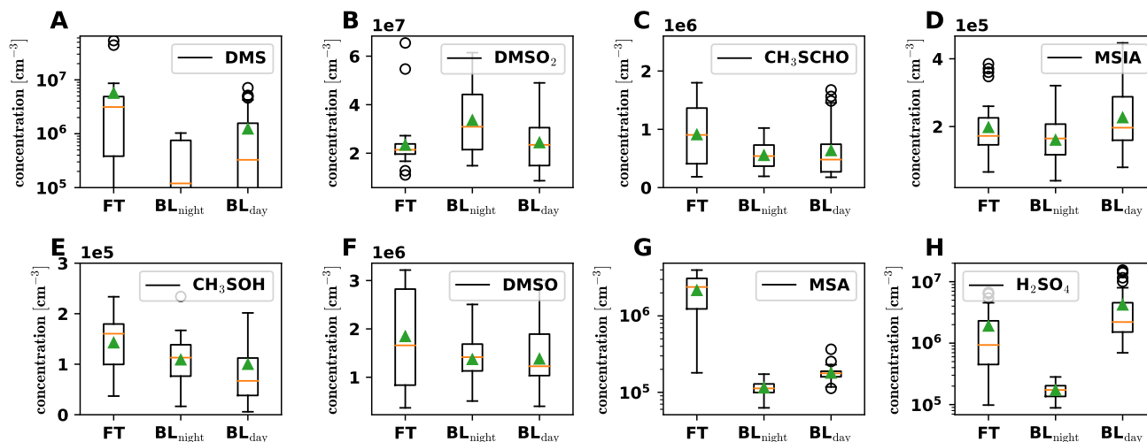
Figure 6. Boxplots of gas phase DMS oxidation products, detected by PTR3 and nitrate-CIMS in the FT (free troposphere without boundary layer influence), BL night (within boundary layer during night time), BL day (within boundary layer during day time) air masses, respectively. The plots are based on 32 data points from averaged 30-minute intervals each, with nighttime and daytime boundary layer conditions chosen to be as close in time as possible to FT periods with the same prevailing wind direction (horizontal air mass origin) for optimal comparison. The orange line shows the median, the green triangle the mean value of the data.
