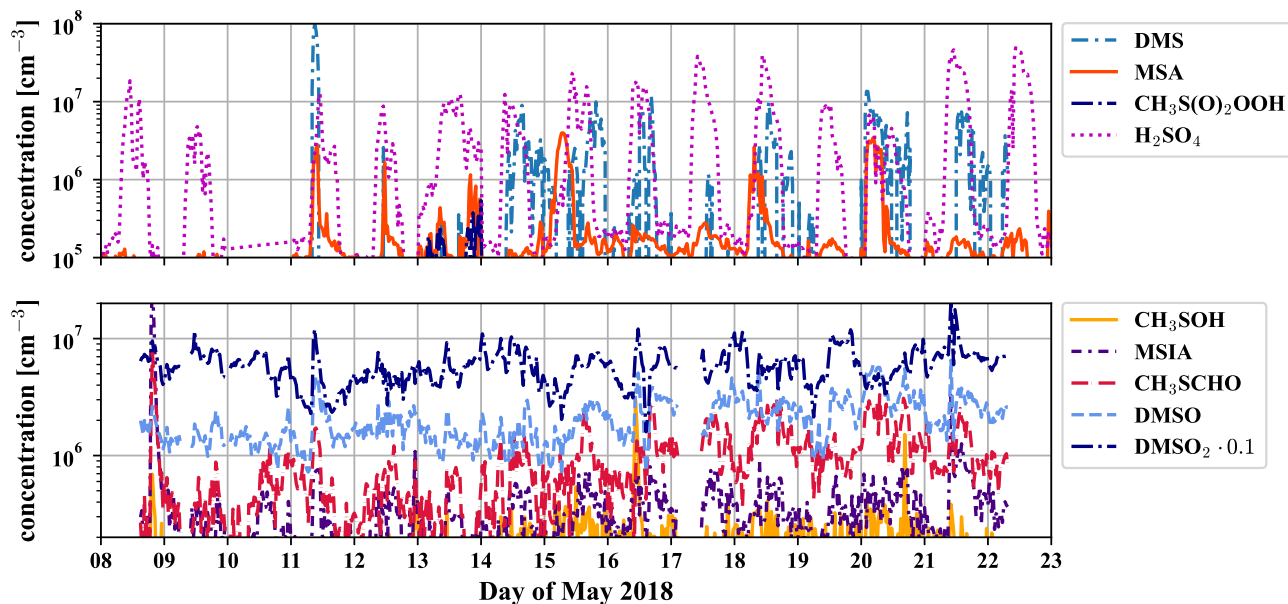
Figure D1. Time series of all detected compounds (measured by PTR3 and nitrate-CIMS) that belong to the DMS oxidation scheme during two weeks of May 2018.
