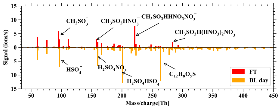
Figure D3. Spectra of the nitrate-CIMS, showing the difference FT - BL_{day} on the positive axis and BL_{day} - FT on the negative axis. Only very few compounds are larger in FT than BL_{day} : The positive spectrum is dominated by clusters of the primary ions with MSA.
