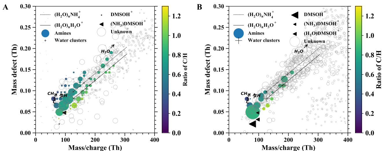
Figure E1. The mass defect for airborne ions in the continental boundary layer (A) and the free troposphere (B). The data are averaged over 1 hour.
