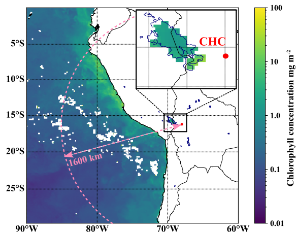
Figure 1. The location of the Chacaltaya GAW station (CHC) with a focus on potential DMS emission hotspots in the region. The color code shows the average Chlorophyll concentration in the Pacific Ocean and Lake Titicaca for May 2018 as obtained from satellite data (AQUA/Modis). All lagoons, also those for which no Chlorophyll data are available, are marked with darkblue outlines. The horizontal extent of the model domain for Lagrangian backward calculations (see sec. 2.4 for details) is depicted as a dashed, pink line.
