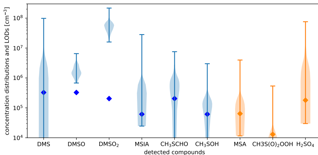
Figure C3. Observed gas-phase organosulfur compounds from PTR3 (blue) and nitrate-CIMS (orange) with their (lower limit) concentration distributions (violins) and limit of detections (LODs, diamonds)
