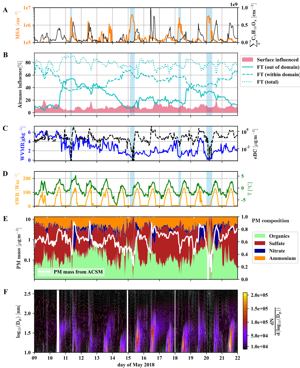
Figure 3. Overview of two weeks of data for the identification of free tropospheric periods. Methanesulfonic acid (MSA) and summed C_8H_{10}O_x (A), the influence of surface ( < 500 m a.g.l.) and free tropospheric air masses ( > 1500 m a.g.l.) according to FLEXPART, with free tropospheric (FT (total)) air masses shown additionally divided into the air from within and without the FLEXPART domain (B), water vapor mixing ratio (WVMR, solid) and equivalent black carbon mass (eBC, dashed) (C), short wave radiation (SWR) and temperature (T) (D), particle matter (PM) mass and composition from Q-ACSM (E) and particle number distribution ( \frac{dN}{d\log_{10}(D_p)} ) (F) versus local time. Lightblue shaded areas mark times that we consider dominated by free tropospheric air masses due to the low particle load and water vapor mixing ratio.
