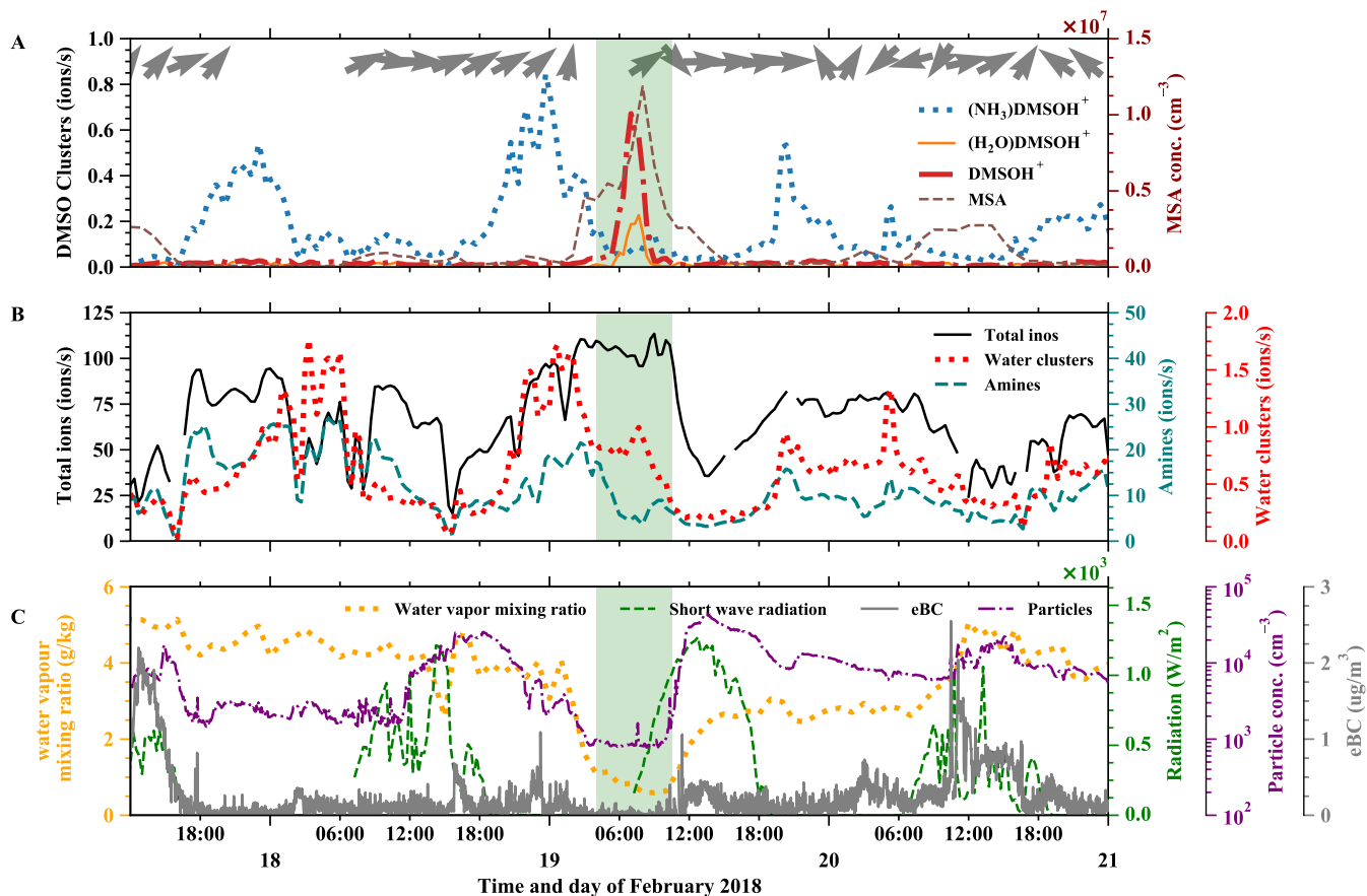
Figure 5. Time evolution of positive ions before, during, and after an FT event (green shaded). A) (\text{NH}_3)\text{DMSOH}^+ , \text{DMSOH}^+ and (\text{H}_2\text{O})\text{DMSOH}^+ clusters, with arrows representing the wind direction on top B) Total positive ions (left axis), amines, and water–ammonia clusters (right axis) from positive APi-TOF. C) Water vapor mixing ratio (left axis), radiation, temperature, and equivalent black carbon (eBC) (right axes).
