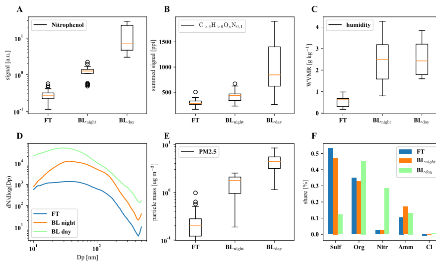
Figure D2. The first row shows Nitrophenol (A), total organics C_{>4}H_{>6}O_xN_{0,1} (B) and water vapor mixing ratio (C), the second row summarizes particle size distribution (D), total PM_{2.5} mass (E), and composition (F). The plots are based on 32 data points from averaged 30-minute intervals each, with nighttime and daytime boundary layer conditions chosen to be as close in time as possible to FT periods with the same prevailing wind direction (horizontal air mass origin) for optimal comparison.
