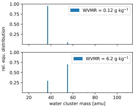
Figure C1. Calculated equilibrium (equ.) primary ion distribution in the PTR3 at the minimum and maximum water vapor mixing ratio (WVMR) inside the PTR3 during the sampling period.
