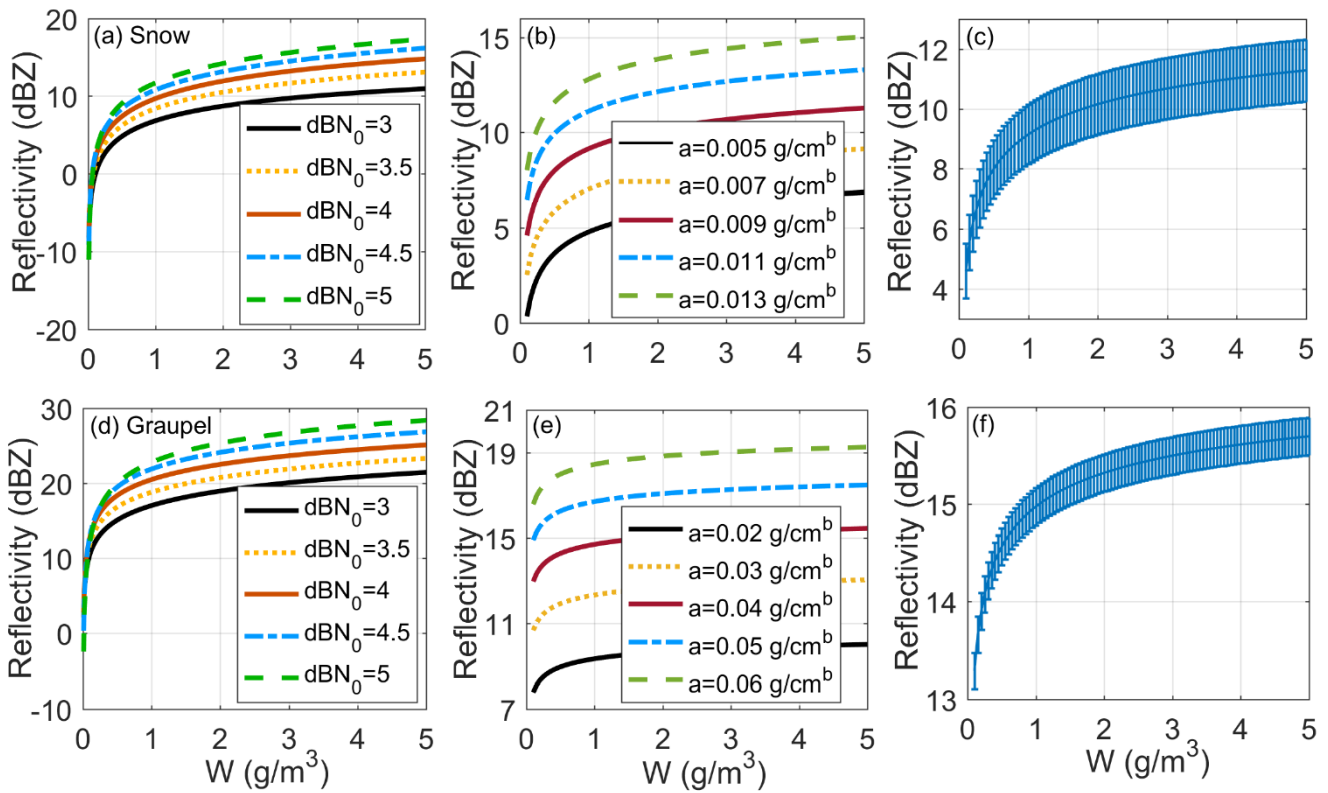
875 Figure 4: Impact of PSD parameters on radar reflectivity for snow and graupel. Variation in reflectivity for snow at (a) \log_{10}(N_0) dBN_0 values of 3, 3.5, 4, 4.5, and 5 with a mean mass-diameter relationship of m = 0.009D^{2.1} , where D is in cm and m is in g; (b) prefactor a in mass-diameter relationship of 0.005, 0.007, 0.009, 0.011, and 0.013 \text{g/cm}^b , with exponent b of 2.1 and N_0 assumed to be 3 \times 10^3 \text{ m}^{-3} \text{ mm}^{-1} ; (c) mean value \pm standard deviation of b , where the mean is 2.1 and standard deviation (SD) is 0.28, with a assumed to be 0.009. The vertical bars represent the SD of the reflectivity change caused by deviation from the mean value of b . 880 Variation in reflectivity for graupel at (d) dBN_0 \log_{10}(N_0) values of 3, 3.5, 4, 4.5, and 5 with a mean mass-diameter relationship of m = 0.04D^{2.6} , where D is in cm and m is in g; (e) prefactor a in mass-diameter relationship of 0.02, 0.03, 0.04, 0.05, and 0.06 \text{g/cm}^b , with exponent b of 2.6 and N_0 assumed to be 4 \times 10^3 \text{ m}^{-3} \text{ mm}^{-1} ; and (f) mean value \pm standard deviation of b , where the mean is 2.6 and standard deviation is 0.16, with a assumed to be 0.04. For a and b we took literature values from list of studies and calculated 885 the mean, and the standard deviation of b for snow and graupel are calculated according to the range and average of Gaussian distribution. The value range in a and b and the mean value are obtained from literatures, and the standard deviation of b are calculated according to the range and average of Gaussian distribution.
