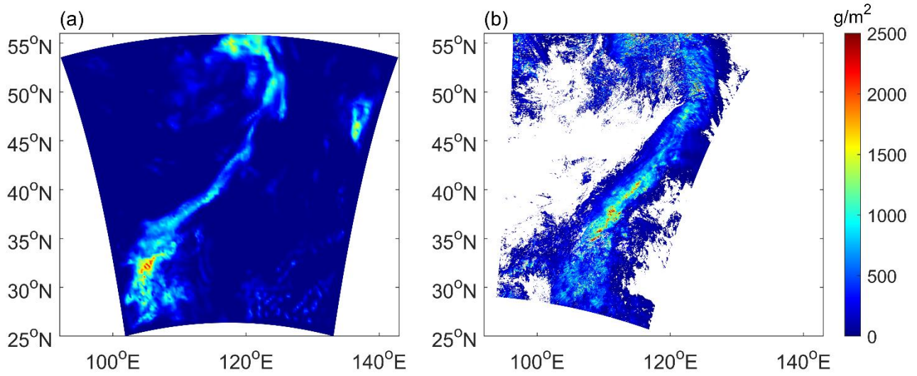
955 Figure A1: Comparison of CWP between the WRF model result and MODIS data for the stratiform case. (a) CWP from the WRF simulation at 03:30 UTC, (b) CWP from MODIS observation at 03:35 UTC, 25 September 2012.
