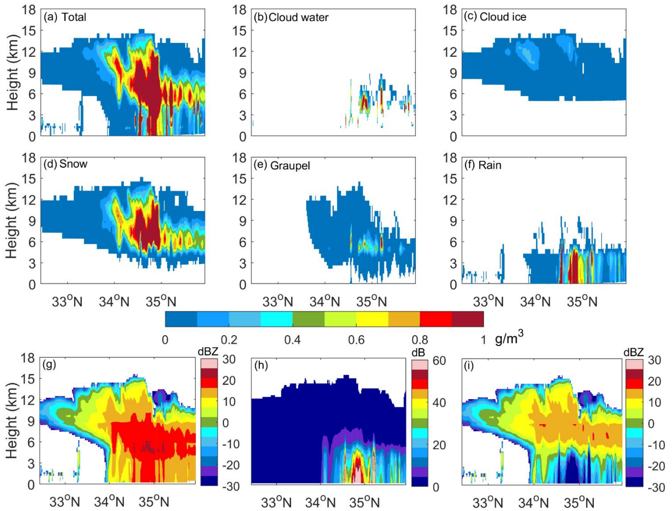
Figure 4.12: Latitude-height cross-section of the hydrometeor of the convective case simulated by the WRF for: (a) total hydrometeors, (b) cloud water, (c) cloud ice, (d) snow, (e) graupel, (f) rain. (g) Simulated unattenuated radar reflectivity with the total hydrometeors, (h) two-way attenuation, and (i) attenuated radar reflectivity.
