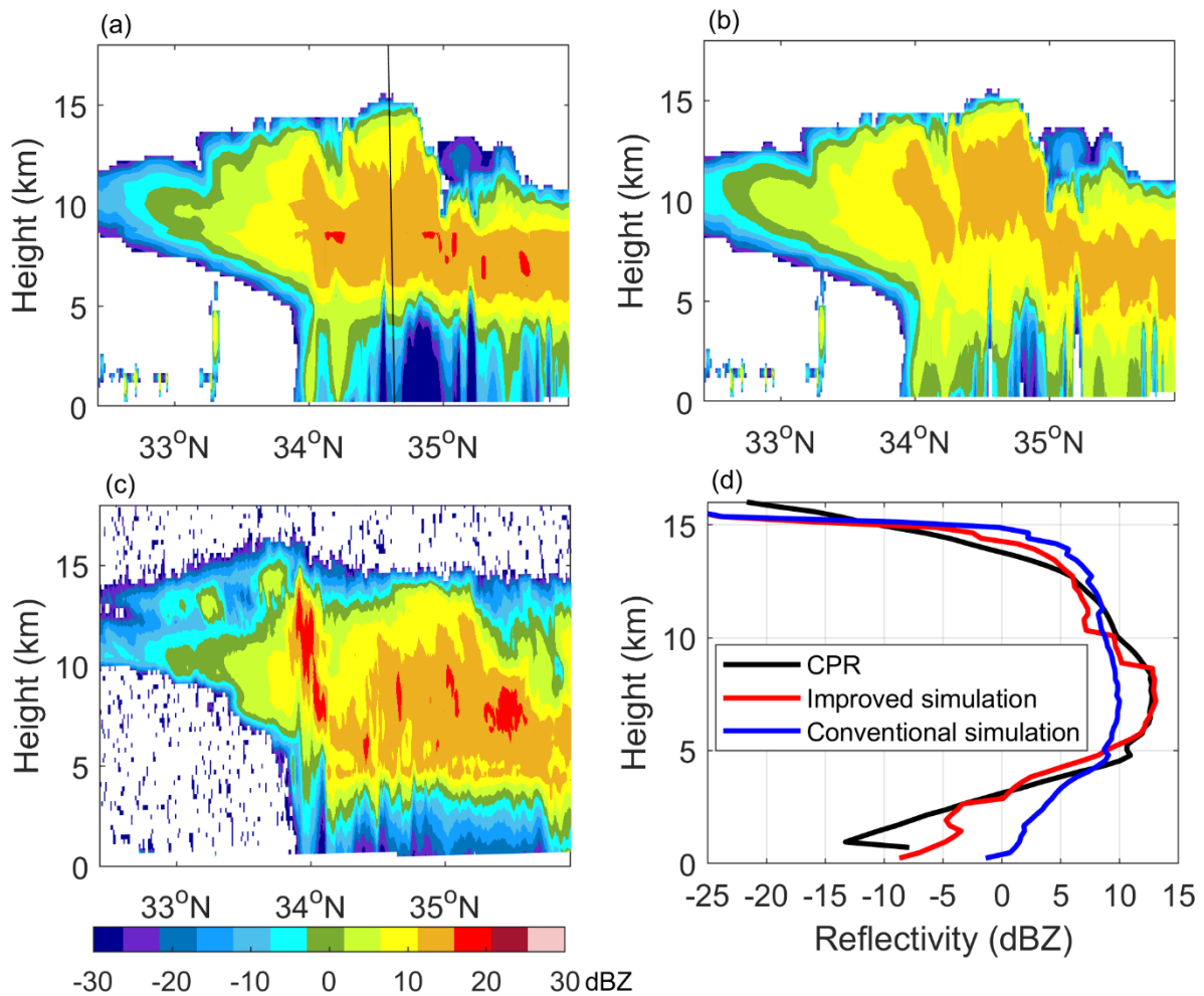
Figure 1213: Radar reflectivity comparison between the simulation results and CloudSat CPR observation data for the convective case. (a) Cross-section of the simulation result with the improved settings, (b) cross-section of the simulation result with the conventional settings using a fixed particle density, and (c) cross-section of the CloudSat CPR observation data. (d) Vertical profiles of the average reflectivity in (a)–(c), where the red line represents the simulation result with the improved settings, blue line represents the simulation results with the conventional settings, and black line represents the result of the CPR observation. The varying prefactor of density relations of snow and graupel due to the effect of riming was considered in the improved simulation. The echo structure and intensity between the improved simulation and CloudSat observation showed good agreement.
