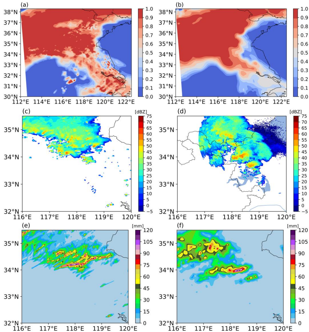
Figure A2: Comparison between the WRF model result and observation data for the convective case. (a) Fraction of cloud cover from the WRF model, (b) fraction of cloud cover from the ERA5 data, (c) radar reflectivity from the WRF model at 04:00 UTC, (d) radar reflectivity observed by the Lianyungang radar at 04:02 UTC, 23 June, (e) WRF model-simulated 6h accumulated rainfall from 0:00 to 06:00 UTC, 23 June, (f) 6h accumulated rainfall from rain gauge data from 0:00 to 06:00 UTC, 23 June 2016.”
