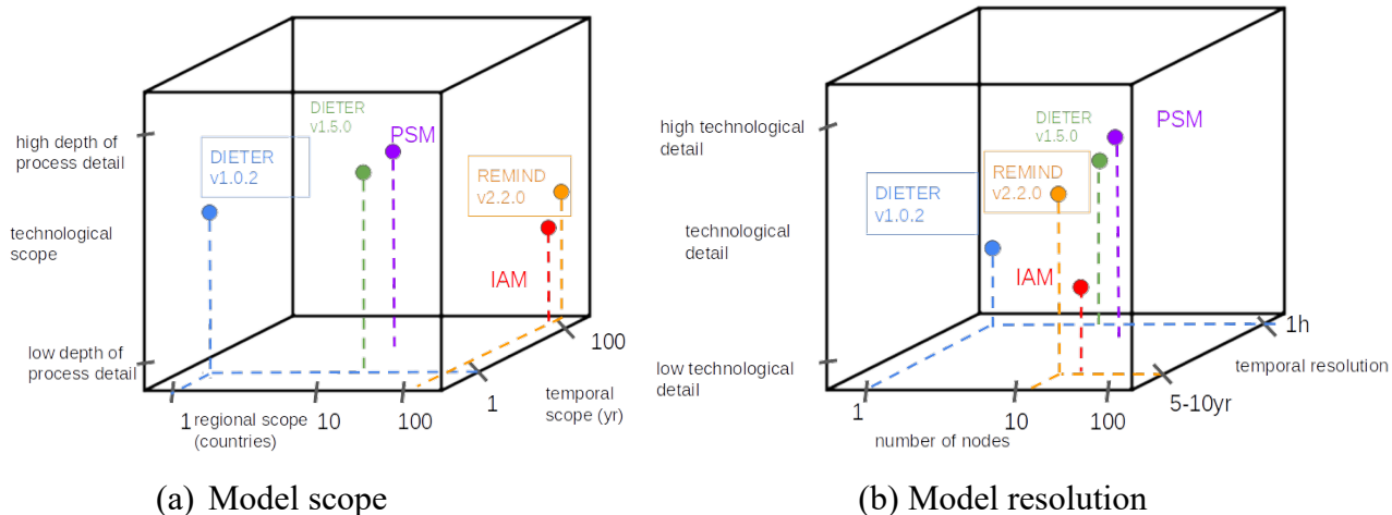
Figure A1: Comparison of resolution and scope for REMIND and a typical IAM, as well as two versions of DIETER (v1.0.2 is used in this study) and a typical PSM.
