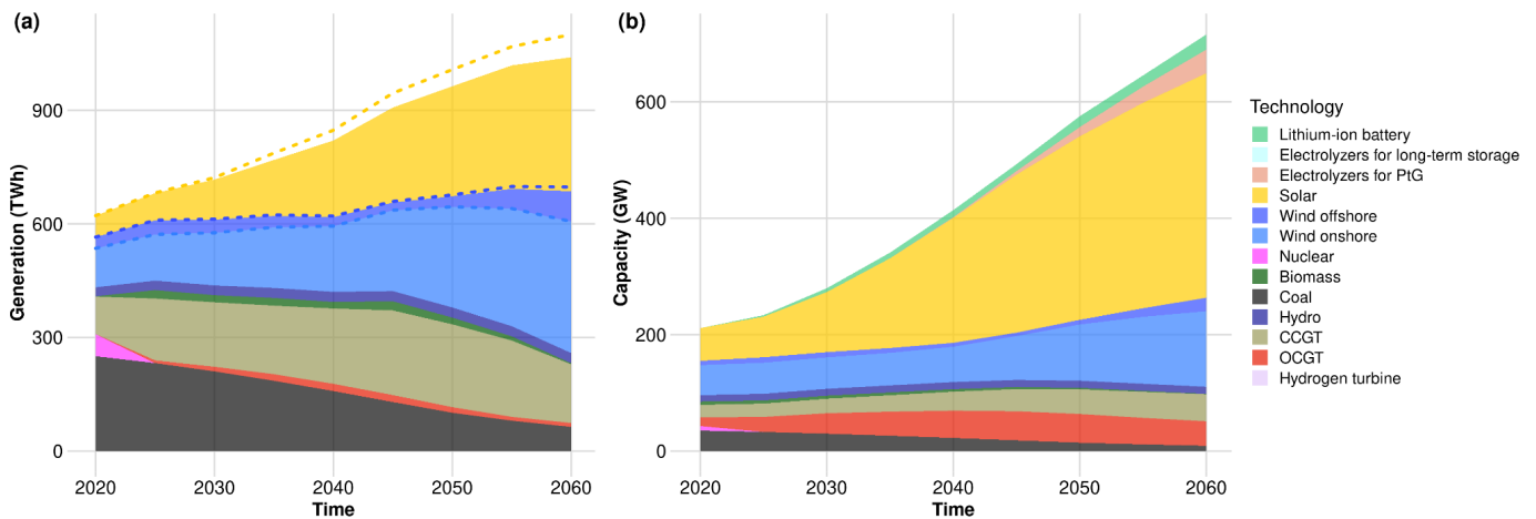
Figure 9: DIETER-REMIND converged results of the long-term (a) generation and (b) capacity expansion for Germany’s power sector in the baseline scenario, assuming a constant 37$/tCO 2 CO 2 price. Dashed lines represent generation before storage loss and curtailment. Storage generation is not visualized in (a).
