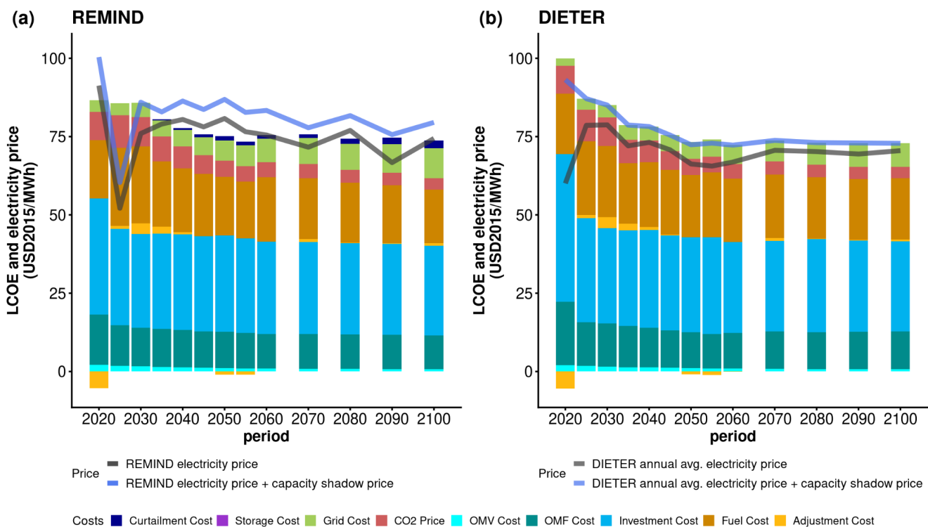
Figure 7: Cost components of the system LCOEs (bars), electricity prices (grey lines) and the sum of electricity prices and capacity shadow prices for (a) REMIND and (b) DIETER under “proof-of-concept” baseline scenario. Visually the ZPRs for both models are satisfied within numerical tolerance. The intertemporal structure of the LCOE breakdown is very similar for most of the coupled periods. For DIETER, a small remaining difference exists between the price (grey line) and the LCOE (bars), which can be entirely explained by the capacity shadow price due to the standing capacity constraint. The REMIND price time series is a rolling average of 3 time periods. The large negative adjustment costs in 2020 are due to coal and nuclear phase-out.
