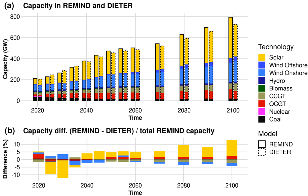
Figure 6: Capacity convergence at the final iteration of a coupled run for Germany under the “proof-of-concept” baseline scenario. (a) Side-by-side comparison of the two models’ capacity mix at the end of the coupled run. (b) The capacity difference between the two models as a share of total REMIND capacity.
