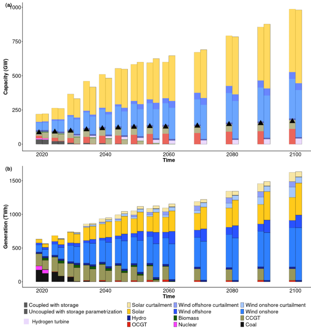
Figure J1: Under the 2C global scenario (no German net-zero goal), we compare (a) the capacity mix and (b) the generation mix of Germany for the DIETER-coupled version of REMIND with endogenous storage (dashed bar) and for the uncoupled version of REMIND with parametrized storage (solid bar). In (a), triangle dots indicate the peak residual demand of the year as determined in DIETER.
