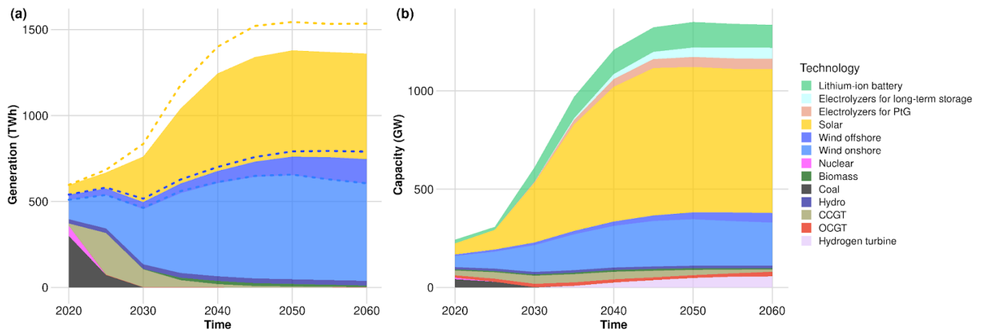
Figure 10: DIETER-REMIND results of the long-term generation and capacity expansion for Germany’s power sector in the “net-zero 2045” scenario. CO 2 price is endogenously determined based on the climate goal. It is 115$/tCO 2 for 2030, 292$/tCO 2 for 2035, 464$/tCO 2 for 2040, and 636$/tCO 2 for 2045. Dashed lines represent pre-curtailment generation. Storage generation is not visualized in (a).
