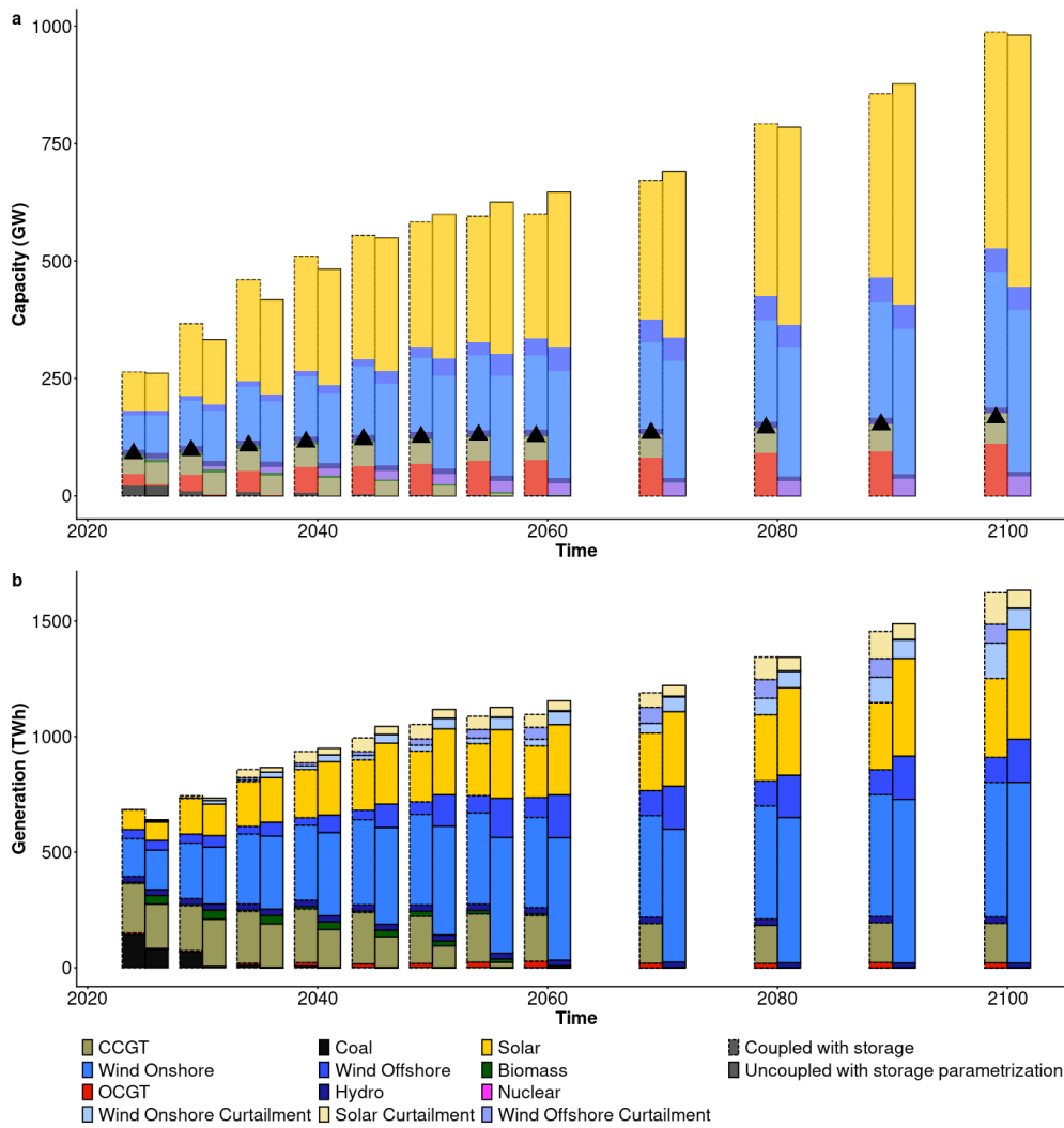
1841 1842 Figure J1: Under the 2C global scenario (no German net-zero goal), we compare (a) the capacity mix and (b) the 1843 generation mix of Germany for the DIETER-coupled version of REMIND with endogenous storage (dashed bar) and for 1844 the uncoupled version of REMIND with parametrized storage (solid bar). In (a), triangle dots indicate the peak residual 1845 demand of the year as determined in DIETER.
