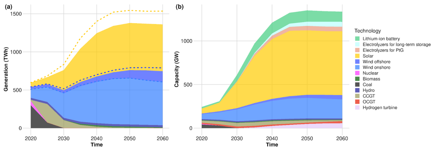
969 970 Figure 10: DIETER-REMIND results of the long-term generation and capacity expansion for Germany's power sector 971 in the “net-zero 2045” scenario. CO 2 price is endogenously determined based on the climate goal. It is 115$/tCO 2 for 972 2030, 292$/tCO 2 for 2035, 464$/tCO 2 for 2040, and 636$/tCO 2 for 2045. Dashed lines represent pre-curtailment 973 generation. Storage generation is not visualized in (a).
