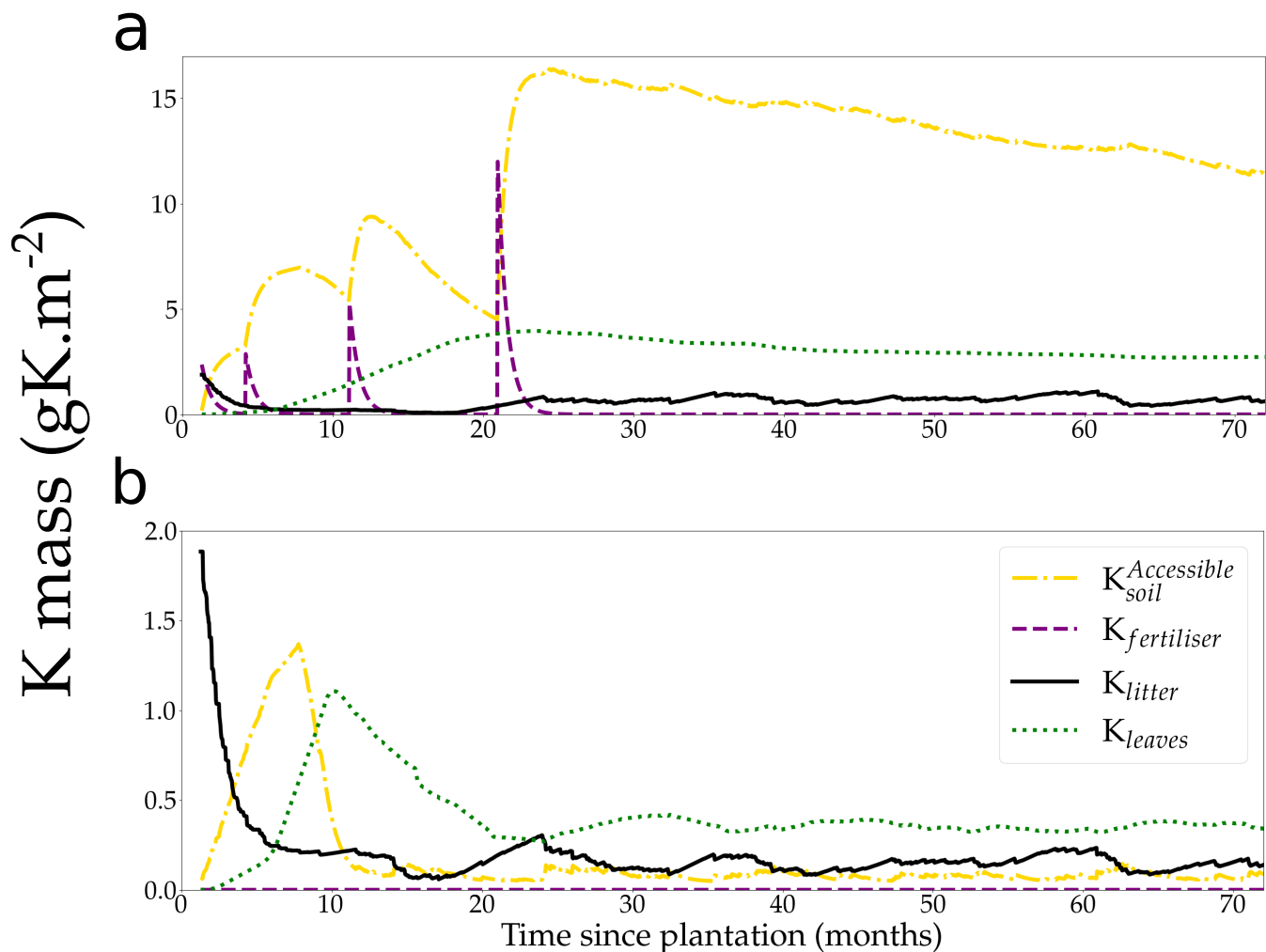
Figure 3. Simulated stocks of K in the soil, litter, fertiliser and canopy compartments, in a non K-limited (+K) stand (a) and in the same K-limited (oK) stand (b). Note differences of the y-axis scales for better visualisation.
