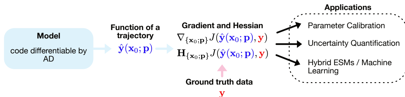
Figure 1. Differentiable programming enables gradient- and Hessian-based optimization of ESMs. For that purpose usually gradients of a cost function J that measures a distance between a desired function evaluation of a trajectory \hat{y} and ground truth data y , e.g. from observations, are computed. The main benefits of this approach that we outline in this article are parameter calibration, uncertainty quantification and the integration of ML methods into Hybrid ESMs
