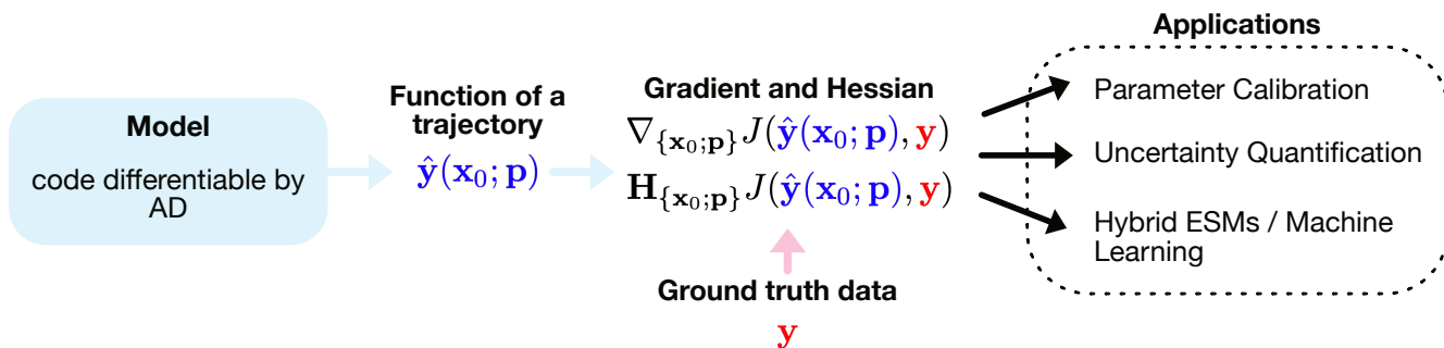
Figure 1. Differentiable programming enables gradient- and Hessian-based optimization of ESMs. Usually, gradients of a cost function J that measures a distance between a desired function evaluation of a trajectory \hat{\mathbf{y}} and ground truth data \mathbf{y} , e.g. from observations, are computed. The main benefits of this approach that we outline in this article are parameter calibration, uncertainty quantification and the integration of ML methods into Hybrid ESMs
