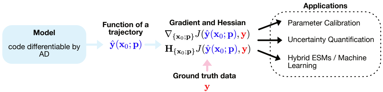
Figure 1. Differentiable programming enables gradient- and Hessian-based optimization of ESMs. For that purpose usually Usually , gradients of a cost function J that measures a distance between a desired function evaluation of a trajectory \hat{\mathbf{y}} and ground truth data \mathbf{y} , e.g. from observations, are computed. The main benefits of this approach that we outline in this article are parameter calibration, uncertainty quantification and the integration of ML methods into Hybrid ESMs
