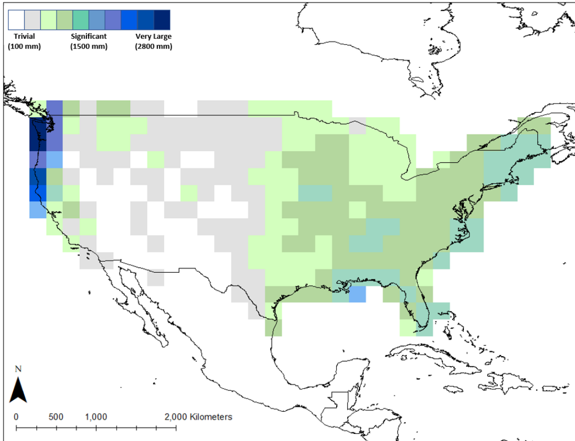
Figure S1. The difference between aggregated PRISM precipitation (1.9x1.9 degree) and modeled CAM-chem precipitation (1.9x1.9 degree) over the US in 2010. The greatest differences are in coastal areas.
