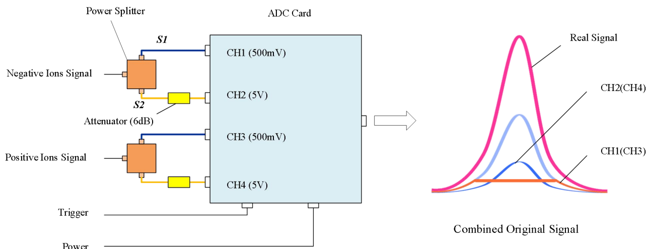
485 Figure 2: Schematic diagram of the working principle of multi-channel data acquisition. The ion signals were acquired separately using two channels with different ranges (500mV and 5V) of the ADC (8-bit). Finally, the real signal intensity was obtained by synthesizing the signals of two channels through software algorithms, and the dynamic acquisition range reached 4mV~20V.
