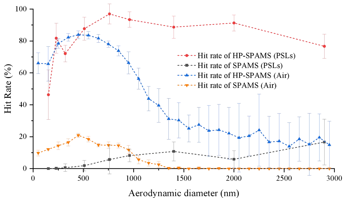
455 Figure 5: The HP-SPAMS and SPAMS hit rate plots for PSLs and air at different particle sizes. Both for measuring PSLs and air, HP-SPAMS had a higher hit rate than SPAMS. For PSLs particles, the hit rate of HP-SPAMS could be maintained in the range of 200-3000 nm from 80 % to 100 % for PSLs, while the SPAMS was within 20 %.
