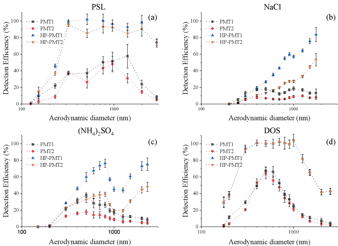
450 Figure 4: Comparison of HP-SPAMS and SPAMS for different particle sizing scattering efficiency ranged from 100~3000 nm. The PMT1 and PMT2 represent the detection efficiencies of the two photomultiplier tubes of SPAMS, respectively, and HP-PMT1 and HP-PMT2 are the detection efficiencies of the two photomultiplier tubes of HP-SPAMS scattering efficiency.
